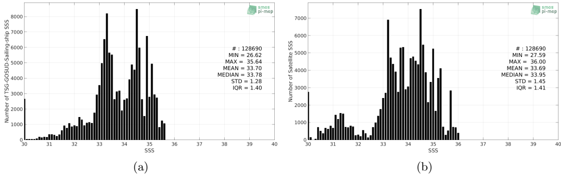
Figure 2: Histograms of SSS from TSG-GOSUD-Sailing-ship (a) and SMOS-L3-CATDS-CECOS-LOCEAN-V3-9DAYS-25KM (b) considering all match-up pairs per bins of 0.1 over the North Pacific Ocean Pi-MEP region and for the full satellite product period.
