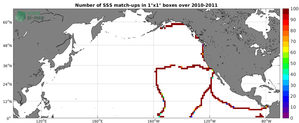
Figure 4: Number of SSS match-ups between TSG-GOSUD-Sailing-ship SSS and the SMOS-L3-CATDS-CECOS-LOCEAN-V3-9DAYS-25KM SSS product for the North Pacific Ocean Pi-MEP region over 1°x1° boxes and for the full satellite product period.
