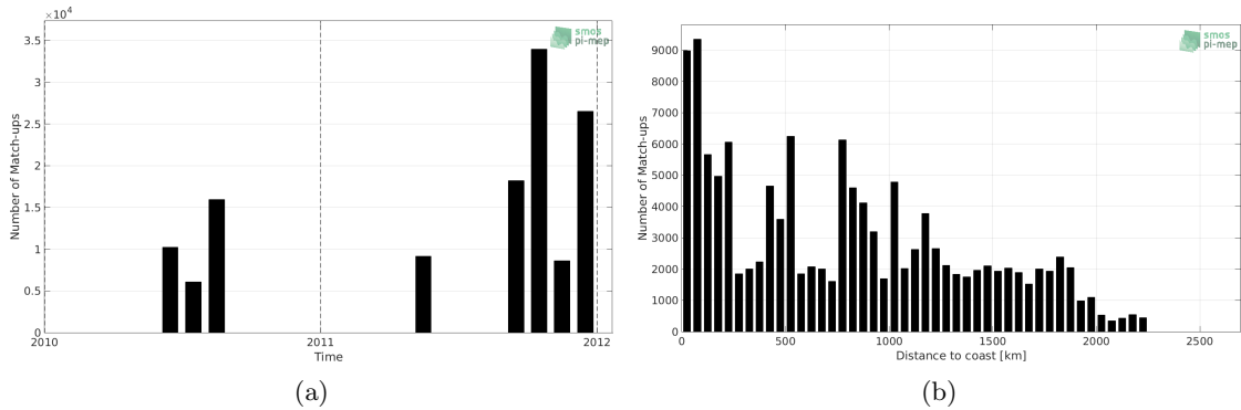
Figure 1: Number of match-ups between TSG-GOSUD-Sailing-ship and SMOS-L3-CATDS-CECOS-LOCEAN-V3-9DAYS-25KM SSS as a function of time (a) and as function of the distance to coast (b) over the North Pacific Ocean Pi-MEP region and for the full satellite product period.
