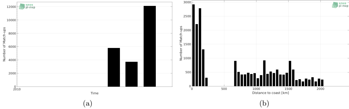
Figure 1: Number of match-ups between TSG-GOSUD-Sailing-ship and SMOS-L3-CATDS-CECOS-LOCEAN-V3-9DAYS-25KM SSS as a function of time (a) and as function of the distance to coast (b) over the North Pacific Ocean Pi-MEP region and for the full satellite product period.
