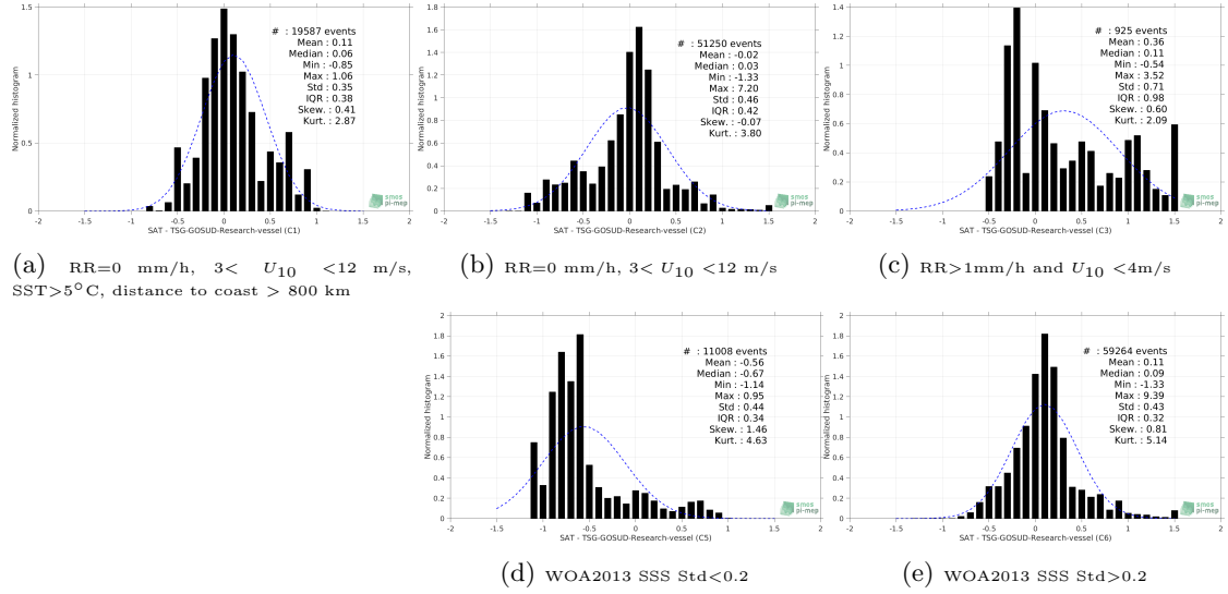
Figure 13: Normalized histogram of \Delta\text{SSS} (SMOS-L3-CATDS-CECOS-LOCEAN-V3-9DAYS-25KM - TSG-GOSUD-Research-vessel) for 5 different subdatasets corresponding to: RR=0 mm/h, 3 < U_{10} < 12 m/s, SST > 5^\circ\text{C} , distance to coast > 800 km (a), RR=0 mm/h, 3 < U_{10} < 12 m/s (b), RR > 1 mm/h and U_{10} < 4 m/s (c), WOA2013 SSS Std < 0.2 (d), WOA2013 SSS Std > 0.2 (e).
