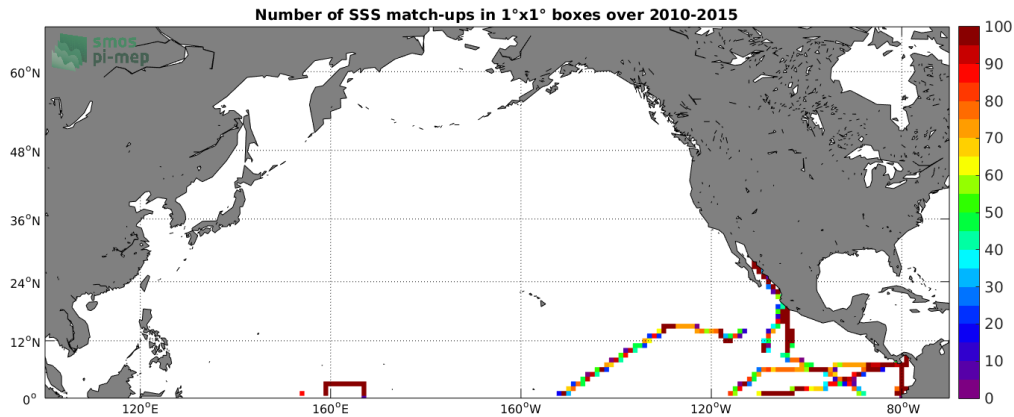
Figure 4: Number of SSS match-ups between TSG-GOSUD-Research-vessel SSS and the SMOS-L3-CATDS-CECOS-LOCEAN-V3-9DAYS-25KM SSS product for the North Pacific Ocean Pi-MEP region over 1°x1° boxes and for the full satellite product period.
