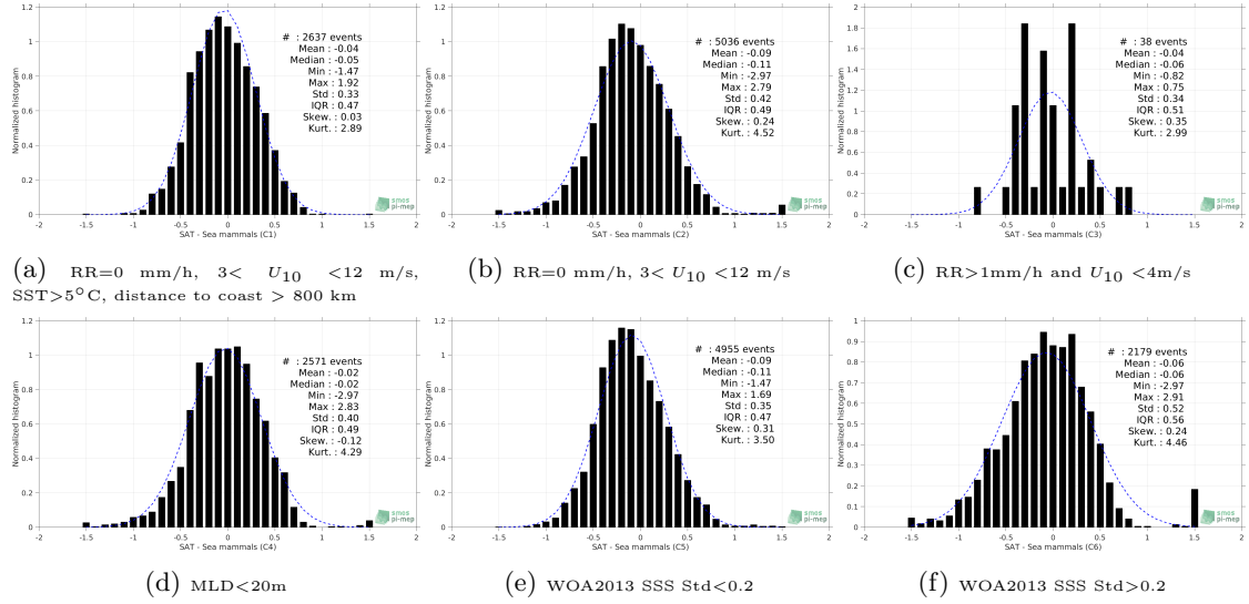
Figure 13: Normalized histogram of \Delta\text{SSS} (SMOS-L3-CATDS-CECOS-LOCEAN-V3-9DAYS-25KM - Sea mammals) for 6 different subdatasets corresponding to: RR=0 mm/h, 3 < U_{10} < 12 m/s, SST>5°C, distance to coast > 800 km (a), RR=0 mm/h, 3 < U_{10} < 12 m/s (b), RR>1mm/h and U_{10} < 4 m/s (c), MLD<20m (d), WOA2013 SSS Std<0.2 (e), WOA2013 SSS Std>0.2 (f).
