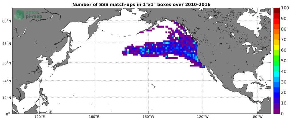
Figure 4: Number of SSS match-ups between Sea mammals SSS and the SMOS-L3-CATDS-CECOS-LOCEAN-V3-9DAYS-25KM SSS product for the North Pacific Ocean Pi-MEP region over 1^\circ \times 1^\circ boxes and for the full satellite product period.
