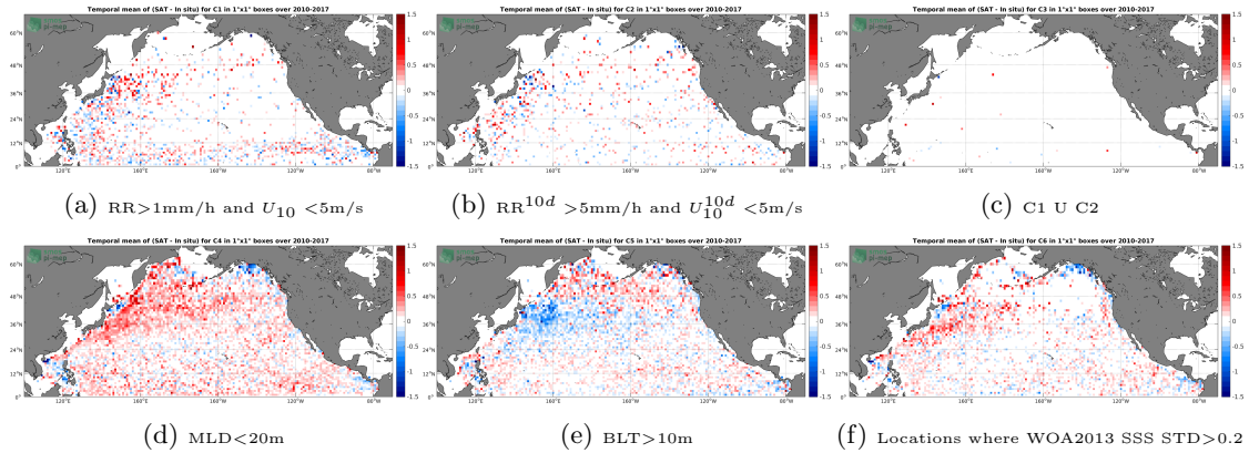
Figure 12: Temporal mean gridded over spatial boxes of size 1°x1° of \Delta SSS (SMOS-L3-CATDS-CECOS-LOCEAN-V3-9DAYS-25KM - Argo) for 6 different subdatasets corresponding to:RR>1mm/h and U_{10} < 5m/s (a), RR^{10d} > 5mm/h and U_{10}^{10d} < 5m/s (b), C1 U C2 (c),MLD<20m (d),BLT>10m (e),Locations where WOA2013 SSS STD>0.2 (f).
