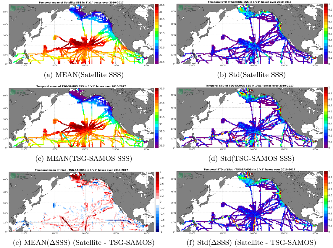
Figure 6: Temporal mean (left) and Std (right) of SSS from SMOS-L3-CATDS-CECOS-LOCEAN-V3-18DAYS-25KM (top), TSG-SAMOS (middle), and of \Delta SSS (Satellite - TSG-SAMOS). Only match-up pairs are used to generate these maps.
