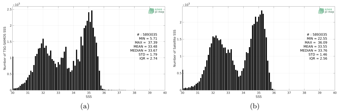
Figure 2: Histograms of SSS from TSG-SAMOS (a) and SMOS-L3-CATDS-CECOS-LOCEAN-V3-18DAYS-25KM (b) considering all match-up pairs per bins of 0.1 over the North Pacific Ocean Pi-MEP region and for the full satellite product period.
