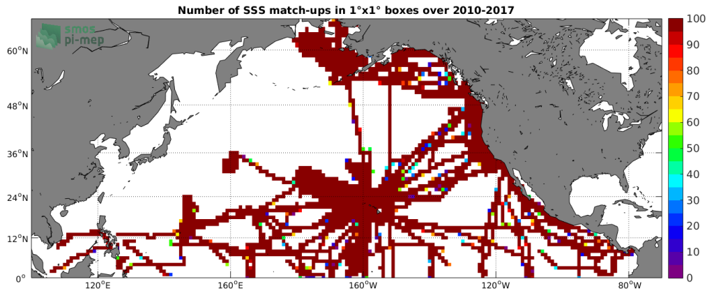
Figure 4: Number of SSS match-ups between TSG-SAMOS SSS and the SMOS-L3-CATDS-CECOS-LOCEAN-V3-18DAYS-25KM SSS product for the North Pacific Ocean Pi-MEP region over 1^\circ \times 1^\circ boxes and for the full satellite product period.
