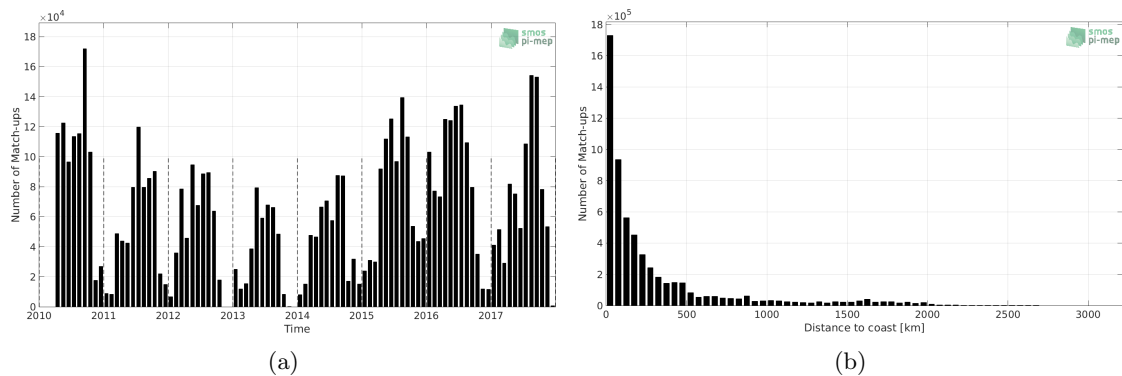
Figure 1: Number of match-ups between TSG-SAMOS and SMOS-L3-CATDS-CECOS-LOCEAN-V3-18DAYS-25KM SSS as a function of time (a) and as function of the distance to coast (b) over the North Pacific Ocean Pi-MEP region and for the full satellite product period.
