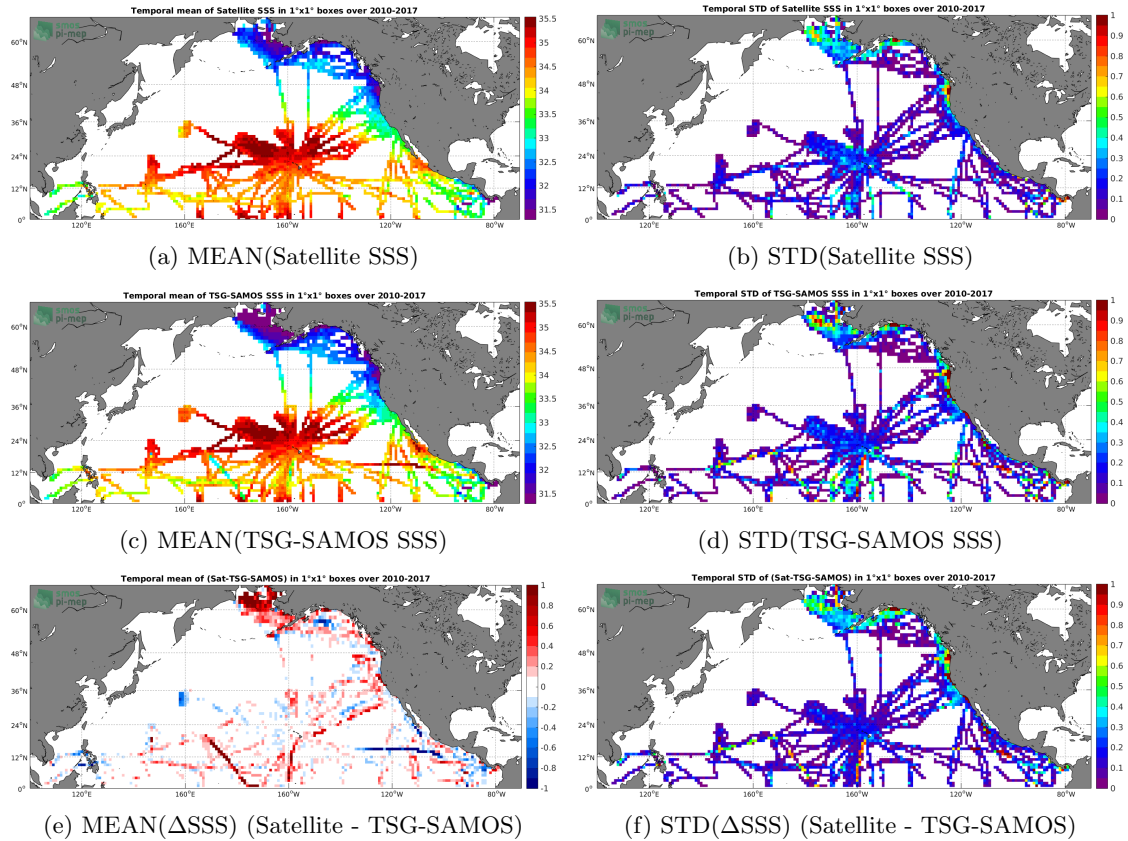
Figure 6: Temporal mean (left) and STD (right) of SSS from SMOS-L3-CATDS-CECOS-LOCEAN-V3-18DAYS-25KM satellite SSS product (top), TSG-SAMOS (middle), and of \Delta SSS (Satellite - TSG-SAMOS). Only match-up pairs are used to generate these maps.
