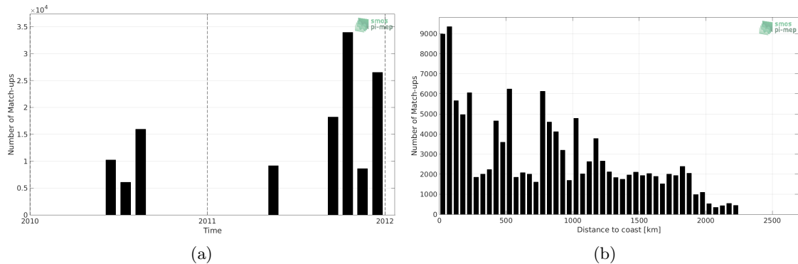
Figure 1: Number of match-ups between TSG-GOSUD-Sailing-ship and SMOS-L3-CATDS-CECOS-LOCEAN-V3-18DAYS-25KM SSS as a function of time (a) and as function of the distance to coast (b) over the North Pacific Ocean Pi-MEP region and for the full satellite product period.
