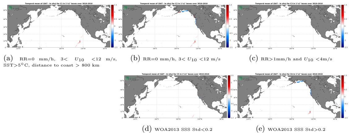
Figure 12: Temporal mean gridded over spatial boxes of size 1^\circ \times 1^\circ of \Delta SSS (SMOS-L3-CATDS-CECOS-LOCEAN-V3-18DAYS-25KM - TSG-GOSUD-Sailing-ship) for 5 different subdatasets corresponding to:RR=0 mm/h, 3 < U_{10} < 12 m/s, SST >5^\circ C, distance to coast > 800 km (a), RR=0 mm/h, 3 < U_{10} < 12 m/s (b), RR >1 mm/h and U_{10} < 4 m/s (c), WOA2013 SSS Std <0.2 (d), WOA2013 SSS Std >0.2 (e).
