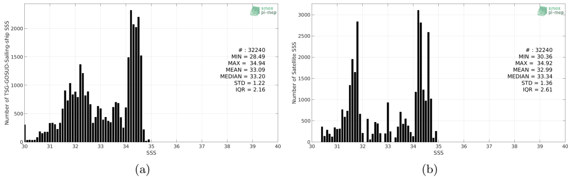
Figure 2: Histograms of SSS from TSG-GOSUD-Sailing-ship (a) and SMOS-L3-CATDS-CECOS-LOCEAN-V3-18DAYS-25KM (b) considering all match-up pairs per bins of 0.1 over the North Pacific Ocean Pi-MEP region and for the full satellite product period.
