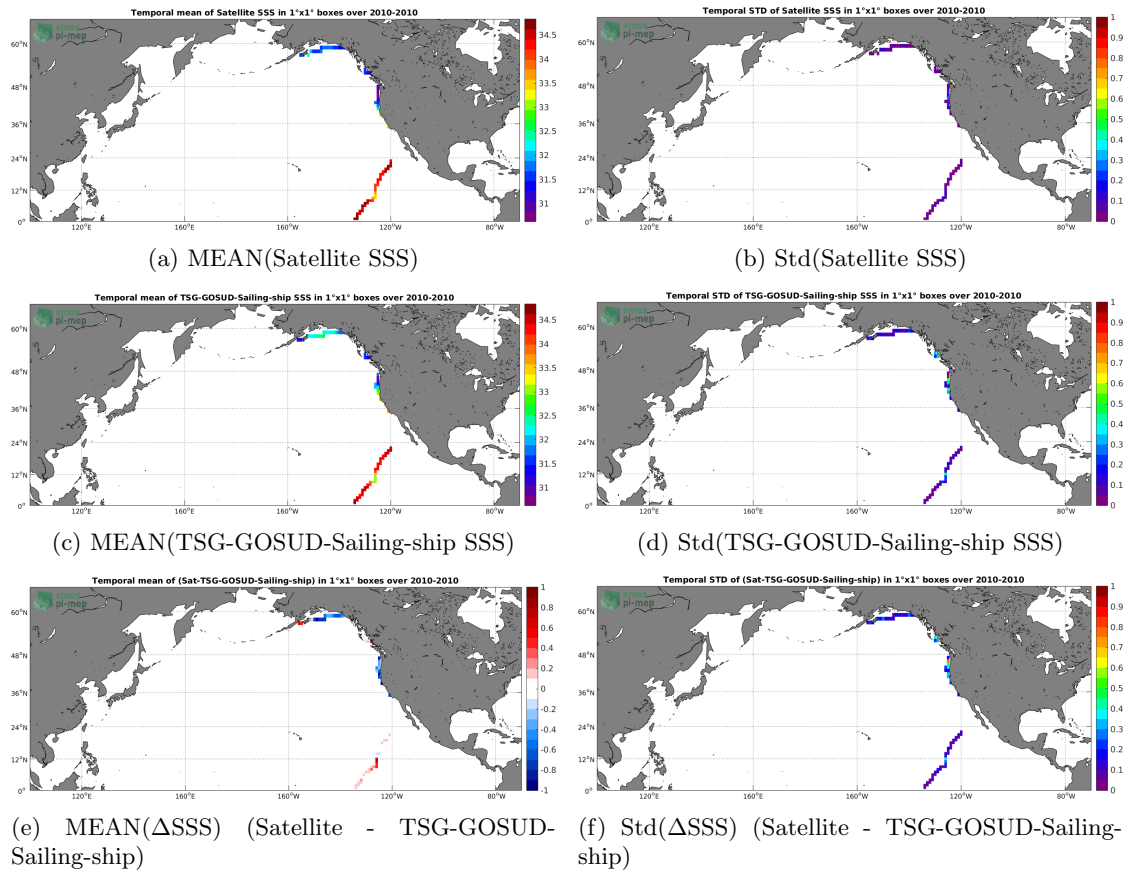
Figure 6: Temporal mean (left) and Std (right) of SSS from SMOS-L3-CATDS-CECOS-LOCEAN-V3-18DAYS-25KM (top), TSG-GOSUD-Sailing-ship (middle), and of \Delta SSS (Satellite - TSG-GOSUD-Sailing-ship). Only match-up pairs are used to generate these maps.
