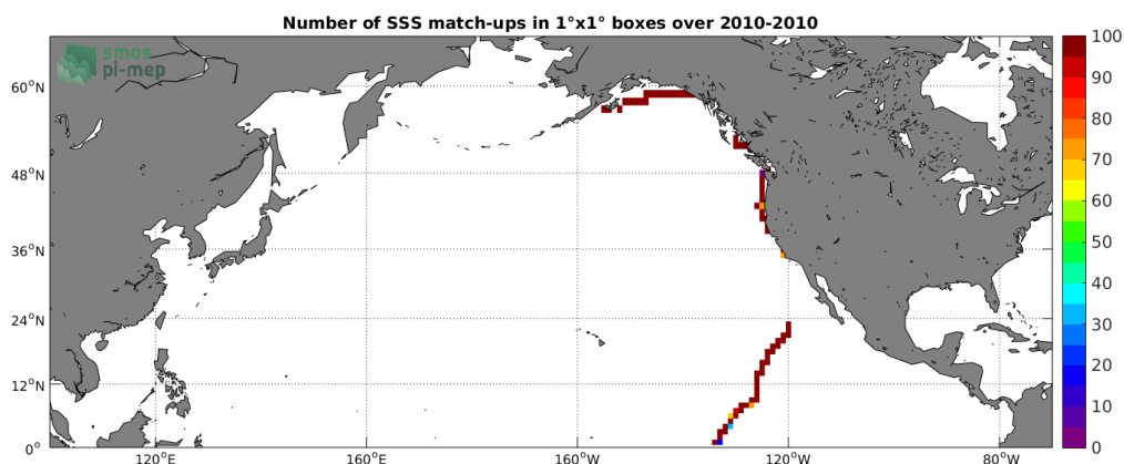
Figure 4: Number of SSS match-ups between TSG-GOSUD-Sailing-ship SSS and the SMOS-L3-CATDS-CECOS-LOCEAN-V3-18DAYS-25KM SSS product for the North Pacific Ocean Pi-MEP region over 1^\circ \times 1^\circ boxes and for the full satellite product period.
