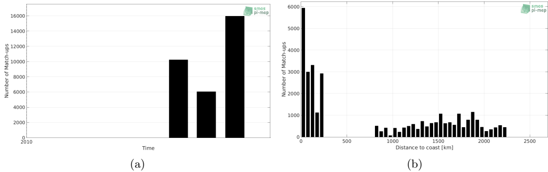
Figure 1: Number of match-ups between TSG-GOSUD-Sailing-ship and SMOS-L3-CATDS-CECOS-LOCEAN-V3-18DAYS-25KM SSS as a function of time (a) and as function of the distance to coast (b) over the North Pacific Ocean Pi-MEP region and for the full satellite product period.
