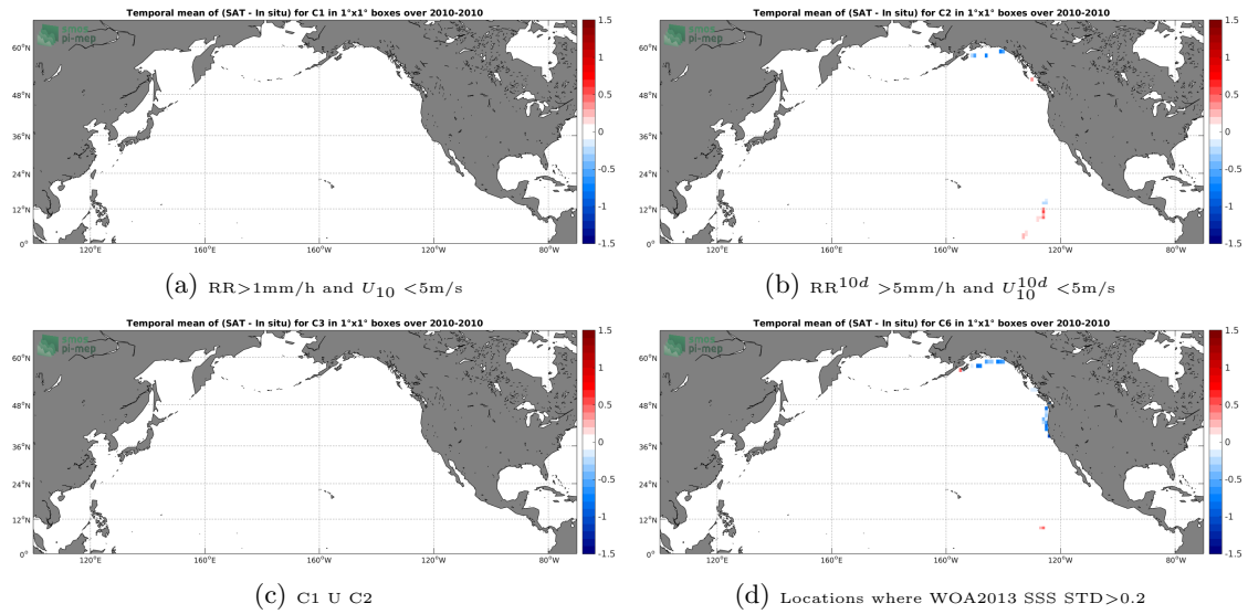
Figure 12: Temporal mean gridded over spatial boxes of size 1^\circ \times 1^\circ of \Delta SSS (SMOS-L3-CATDS-CECOS-LOCEAN-V3-18DAYS-25KM - TSG-GOSUD-Sailing-ship) for 4 different subdatasets corresponding to: RR > 1\text{mm/h} and U_{10} < 5\text{m/s} (a), RR^{10d} > 5\text{mm/h} and U_{10}^{10d} < 5\text{m/s} (b), C1 U C2 (c), Locations where WOA2013 SSS STD > 0.2 (d).
