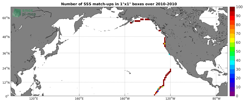
Figure 4: Number of SSS match-ups between TSG-GOSUD-Sailing-ship SSS and the SMOS-L3-CATDS-CECOS-LOCEAN-V3-18DAYS-25KM SSS product for the North Pacific Ocean Pi-MEP region over 1^{\circ} \times 1^{\circ} boxes and for the full satellite product period.
