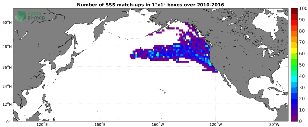
Figure 4: Number of SSS match-ups between Sea mammals SSS and the SMOS-L3-CATDS-CECOS-LOCEAN-V3-18DAYS-25KM SSS product for the North Pacific Ocean Pi-MEP region over 1°x1° boxes and for the full satellite product period.
