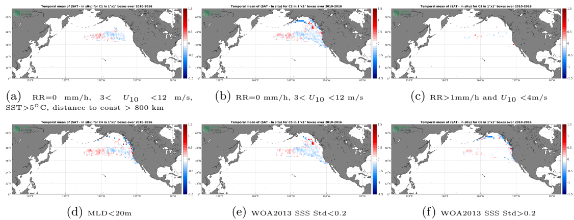
Figure 12: Temporal mean gridded over spatial boxes of size 1^\circ \times 1^\circ of \Delta SSS (SMOS-L3-CATDS-CECOS-LOCEAN-V3-18DAYS-25KM - Sea mammals) for 6 different subdatasets corresponding to:RR=0 mm/h, 3 < U_{10} < 12 m/s, SST >5^\circ C, distance to coast > 800 km (a), RR=0 mm/h, 3 < U_{10} < 12 m/s (b), RR >1 mm/h and U_{10} < 4 m/s (c),MLD <20 m (d),WOA2013 SSS Std <0.2 (e),WOA2013 SSS Std >0.2 (f).
