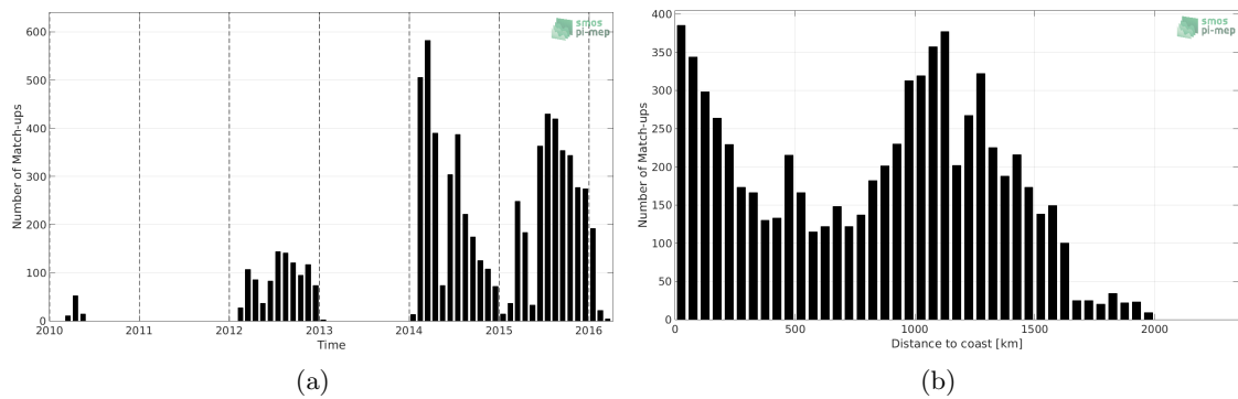
Figure 1: Number of match-ups between Sea mammals and SMOS-L3-CATDS-CECOS-LOCEAN-V3-18DAYS-25KM SSS as a function of time (a) and as function of the distance to coast (b) over the North Pacific Ocean Pi-MEP region and for the full satellite product period.
