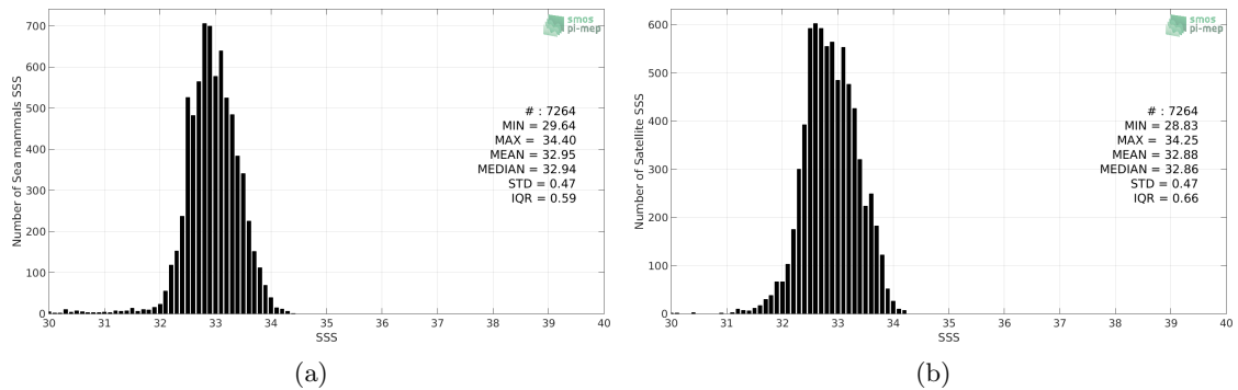
Figure 2: Histograms of SSS from Sea mammals (a) and SMOS-L3-CATDS-CECOS-LOCEAN-V3-18DAYS-25KM (b) considering all match-up pairs per bins of 0.1 over the North Pacific Ocean Pi-MEP region and for the full satellite product period.
