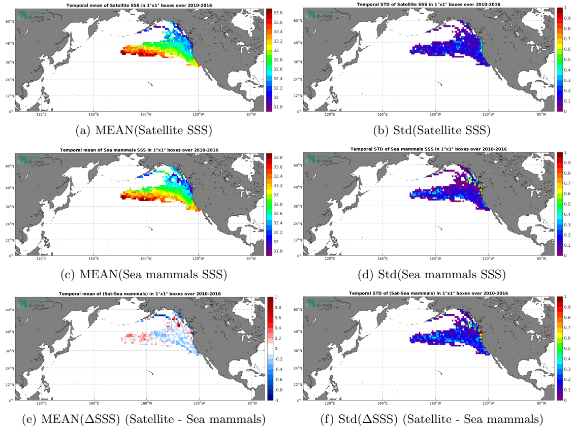
Figure 6: Temporal mean (left) and Std (right) of SSS from SMOS-L3-CATDS-CECOS-LOCEAN-V3-18DAYS-25KM (top), Sea mammals (middle), and of \Delta SSS (Satellite - Sea mammals). Only match-up pairs are used to generate these maps.
