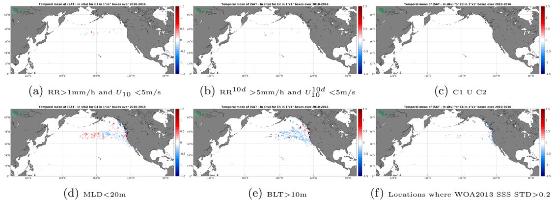
Figure 12: Temporal mean gridded over spatial boxes of size 1°x1° of \Delta SSS (SMOS-L3-CATDS-CECOS-LOCEAN-V3-18DAYS-25KM - Sea mammals) for 6 different subdatasets corresponding to:RR>1mm/h and U_{10} < 5m/s (a), RR^{10d} > 5mm/h and U_{10}^{10d} < 5m/s (b), C1 U C2 (c),MLD<20m (d),BLT>10m (e),Locations where WOA2013 SSS STD>0.2 (f).
