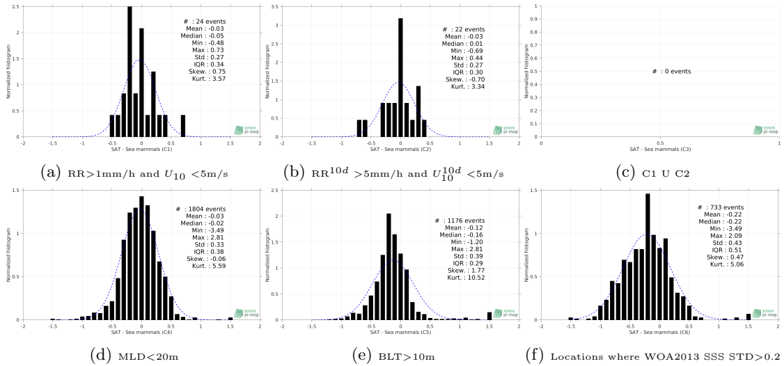
Figure 13: Normalized histogram of \Delta SSS (SMOS-L3-CATDS-CECOS-LOCEAN-V3-18DAYS-25KM - Sea mammals) for 6 different subdatasets corresponding to: RR>1mm/h and U_{10} < 5m/s (a), RR^{10d} > 5mm/h and U_{10}^{10d} < 5m/s (b), C1 U C2 (c),MLD<20m (d),BLT>10m (e),Locations where WOA2013 SSS STD>0.2 (f).
