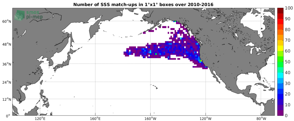
Figure 4: Number of SSS match-ups between Sea mammals SSS and the SMOS-L3-CATDS-CECOS-LOCEAN-V3-18DAYS-25KM SSS product for the North Pacific Ocean Pi-MEP region over 1^\circ \times 1^\circ boxes and for the full satellite product period.
