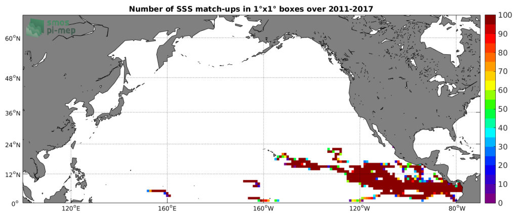
Figure 3: Number of SSS match-ups between Surface drifters SSS and the SMOS-L3-CATDS-CECOS-LOCEAN-V3-18DAYS-25KM SSS product for the North Pacific Ocean Pi-MEP region over 1°x1° boxes and for the full satellite product period.
