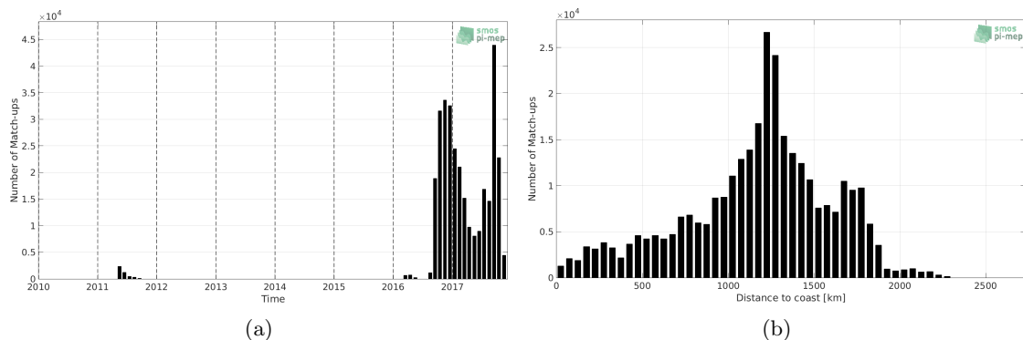
Figure 1: Number of match-ups between Surface drifters and SMOS-L3-CATDS-CECOS-LOCEAN-V3-18DAYS-25KM SSS as a function of time (a) and as function of the distance to coast (b) over the North Pacific Ocean Pi-MEP region and for the full satellite product period.
