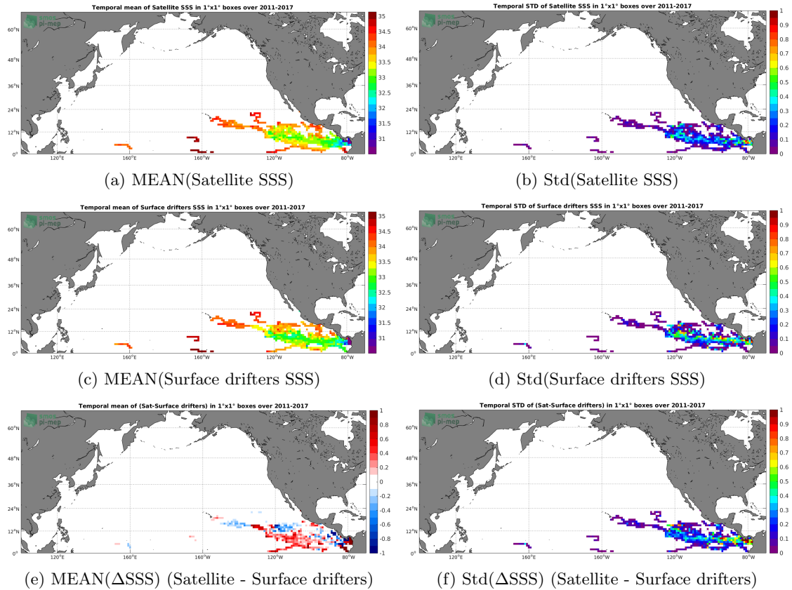
Figure 5: Temporal mean (left) and Std (right) of SSS from SMOS-L3-CATDS-CECOS-LOCEAN-V3-18DAYS-25KM (top), Surface drifters (middle), and of \Delta SSS (Satellite - Surface drifters). Only match-up pairs are used to generate these maps.
