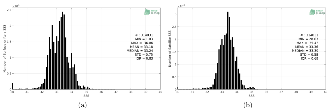
Figure 2: Histograms of SSS from Surface drifters (a) and SMOS-L3-CATDS-CECOS-LOCEAN-V3-18DAYS-25KM (b) considering all match-up pairs per bins of 0.1 over the North Pacific Ocean Pi-MEP region and for the full satellite product period.
