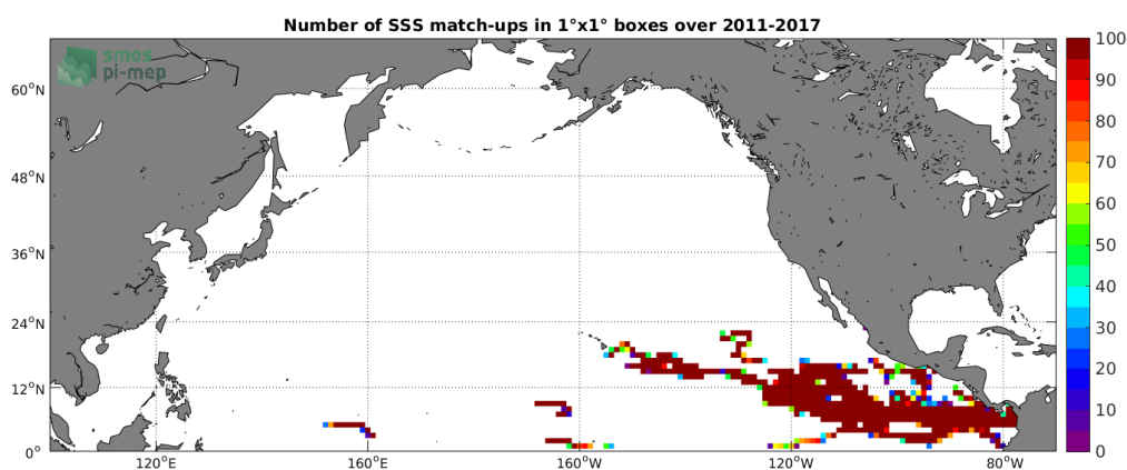
Figure 3: Number of SSS match-ups between Surface drifters SSS and the SMOS-L3-CATDS-CECOS-LOCEAN-V3-18DAYS-25KM SSS product for the North Pacific Ocean Pi-MEP region over 1°x1° boxes and for the full satellite product period.
