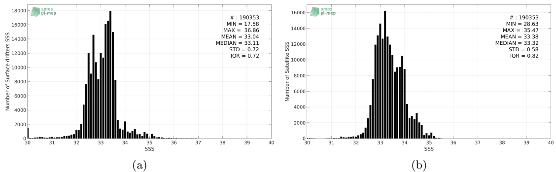
Figure 2: Histograms of SSS from Surface drifters (a) and SMOS-L3-CATDS-CECOS-LOCEAN-V3-18DAYS-25KM (b) considering all match-up pairs per bins of 0.1 over the North Pacific Ocean Pi-MEP region and for the full satellite product period.
