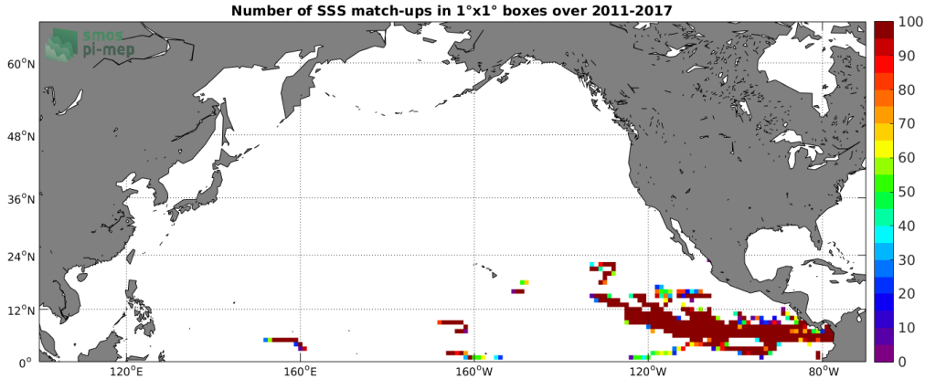
Figure 3: Number of SSS match-ups between Surface drifters SSS and the SMOS-L3-CATDS-CECOS-LOCEAN-V3-18DAYS-25KM SSS product for the North Pacific Ocean Pi-MEP region over 1^\circ \times 1^\circ boxes and for the full satellite product period.
