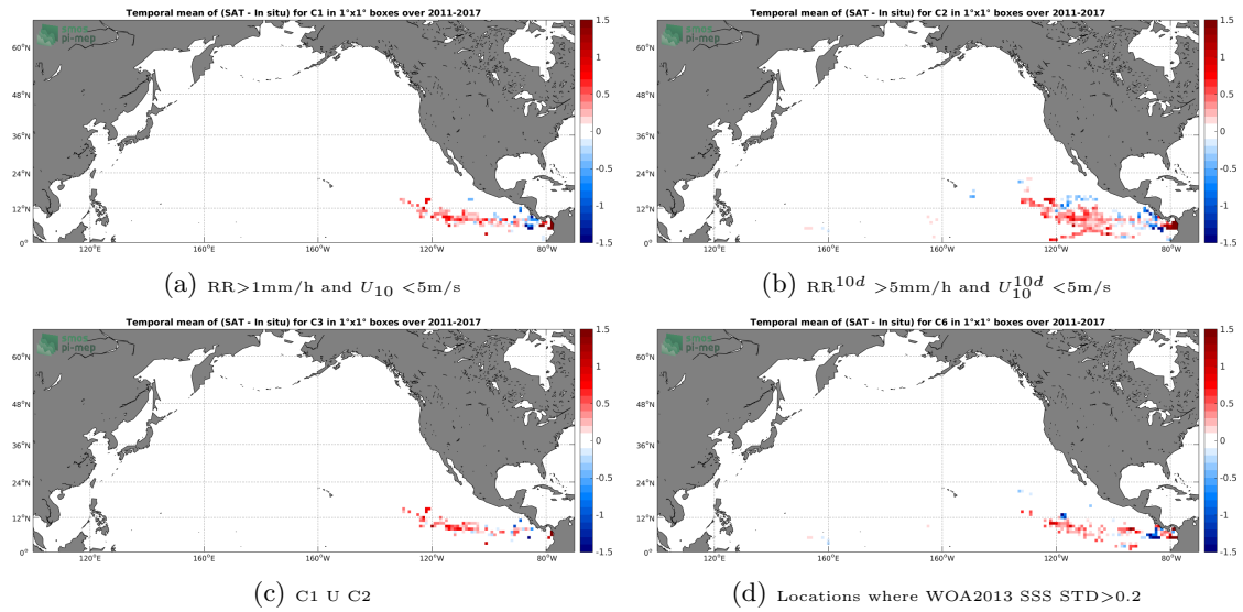
Figure 11: Temporal mean gridded over spatial boxes of size 1^\circ \times 1^\circ of \Delta SSS (SMOS-L3-CATDS-CECOS-LOCEAN-V3-18DAYS-25KM - Surface drifters) for 4 different subdatasets corresponding to: RR > 1mm/h and U_{10} < 5\text{m/s} (a), RR^{10d} > 5\text{mm/h} and U_{10}^{10d} < 5\text{m/s} (b), C1 U C2 (c), Locations where WOA2013 SSS STD > 0.2 (d).
