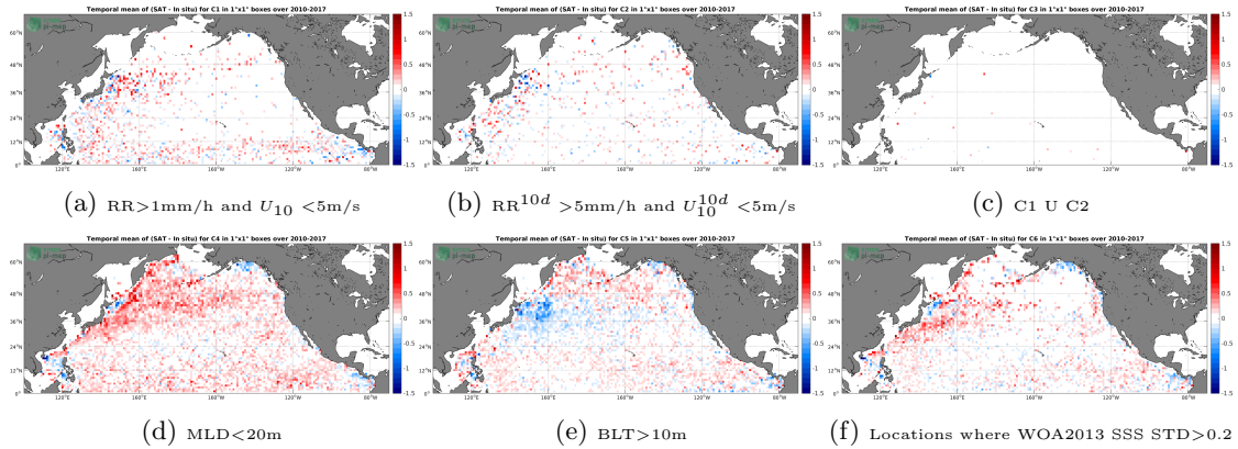
Figure 12: Temporal mean gridded over spatial boxes of size 1^\circ \times 1^\circ of \Delta SSS (SMOS-L3-CATDS-CECOS-LOCEAN-V3-18DAYS-25KM - Argo) for 6 different subdatasets corresponding to: RR > 1\text{mm/h} and U_{10} < 5\text{m/s} (a), RR^{10d} > 5\text{mm/h} and U_{10}^{10d} < 5\text{m/s} (b), C1 U C2 (c), MLD < 20\text{m} (d), BLT > 10\text{m} (e), Locations where WOA2013 SSS STD > 0.2 (f).
