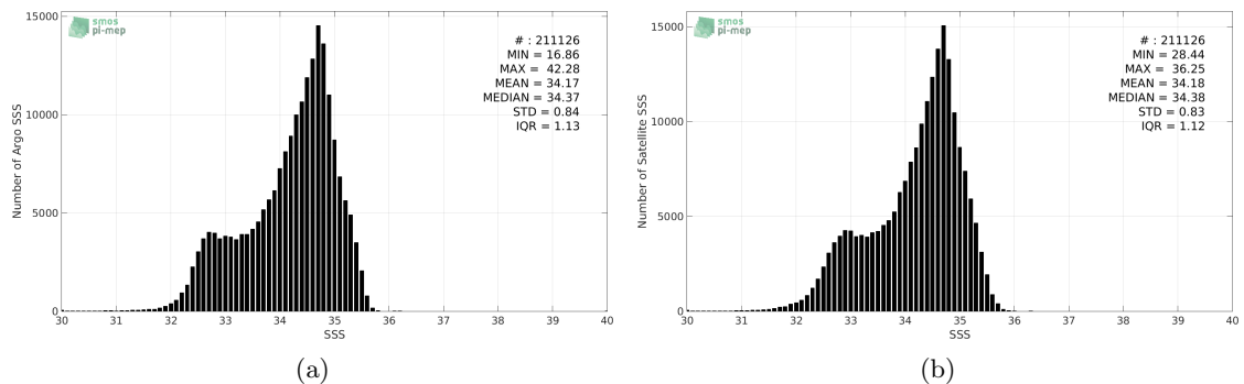
Figure 2: Histograms of SSS from Argo (a) and SMOS-L3-CATDS-CECOS-LOCEAN-V3-18DAYS-25KM (b) considering all match-up pairs per bins of 0.1 over the North Pacific Ocean Pi-MEP region and for the full satellite product period.
