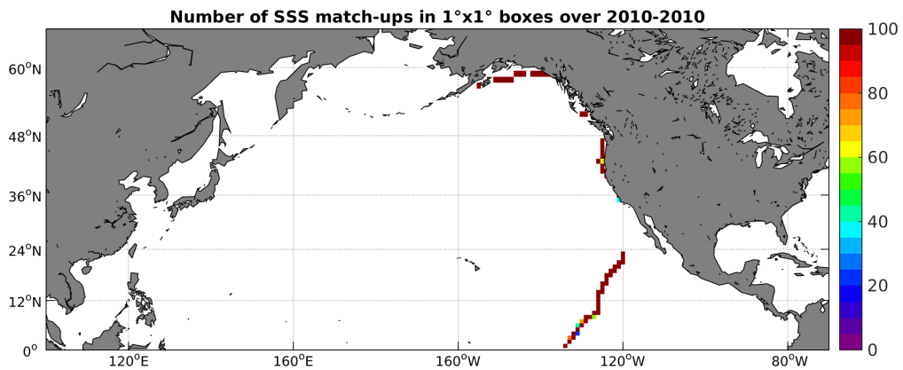
Figure 4: Number of SSS match-ups between TSG-GOSUD-Sailing-ship SSS and the SMOS-L3-CATDS-CECOS-LOCEAN-V2.1-9DAYS-25KM SSS product for the North Pacific Ocean Pi-MEP region over 1^\circ \times 1^\circ boxes and for the full satellite product period.
