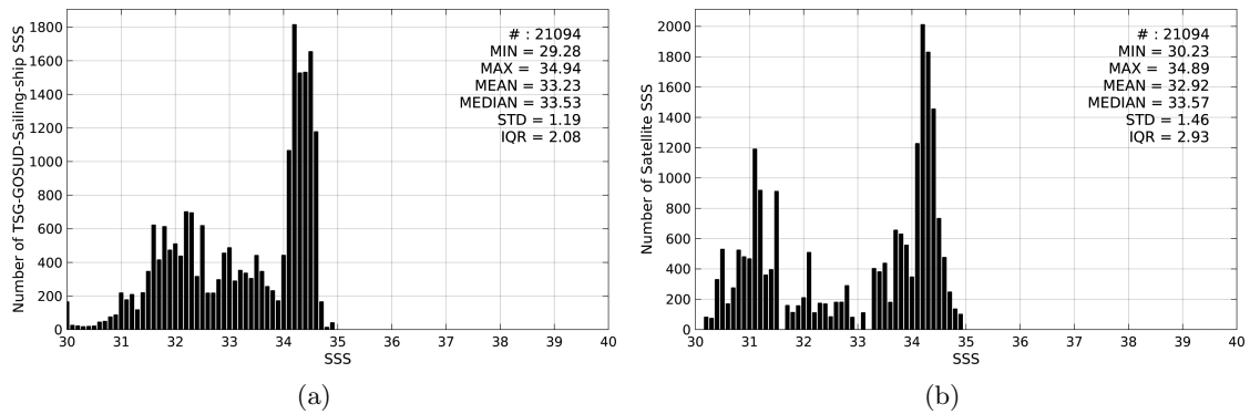
Figure 2: Histograms of SSS from TSG-GOSUD-Sailing-ship (a) and SMOS-L3-CATDS-CECOS-LOCEAN-V2.1-9DAYS-25KM (b) considering all match-up pairs per bins of 0.1 over the North Pacific Ocean Pi-MEP region and for the full satellite product period.
