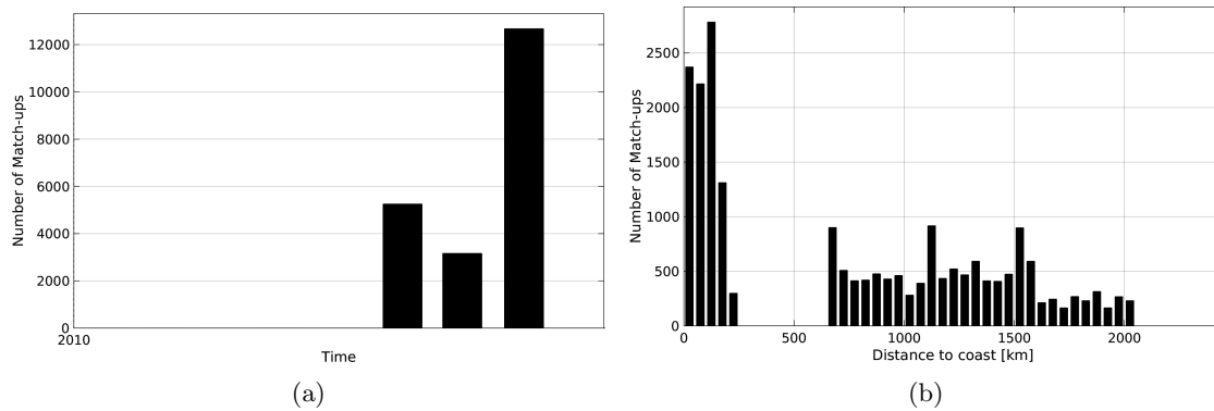
Figure 1: Number of match-ups between TSG-GOSUD-Sailing-ship and SMOS-L3-CATDS-CECOS-LOCEAN-V2.1-9DAYS-25KM SSS as a function of time (a) and as function of the distance to coast (b) over the North Pacific Ocean Pi-MEP region and for the full satellite product period.
