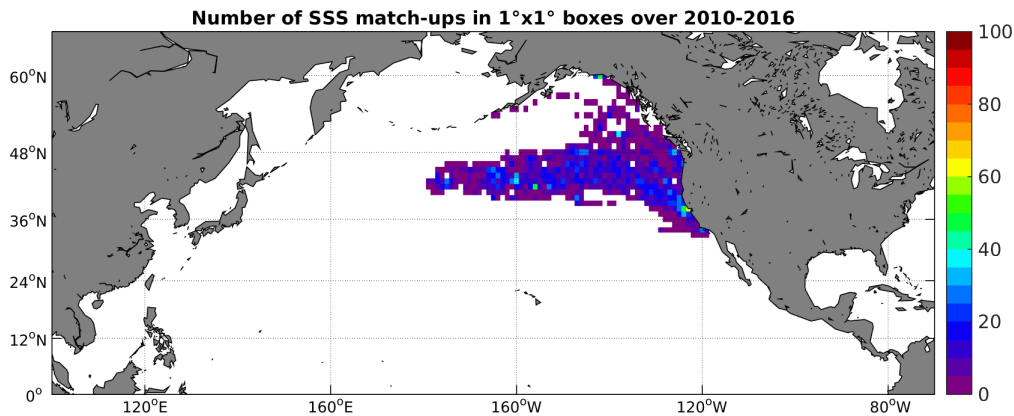
Figure 4: Number of SSS match-ups between Sea mammals SSS and the SMOS-L3-CATDS-CECOS-LOCEAN-V2.1-9DAYS-25KM SSS product for the North Pacific Ocean Pi-MEP region over 1°x1° boxes and for the full satellite product period.
