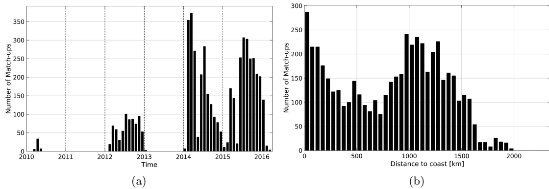
Figure 1: Number of match-ups between Sea mammals and SMOS-L3-CATDS-CECOS-LOCEAN-V2.1-9DAYS-25KM SSS as a function of time (a) and as function of the distance to coast (b) over the North Pacific Ocean Pi-MEP region and for the full satellite product period.
