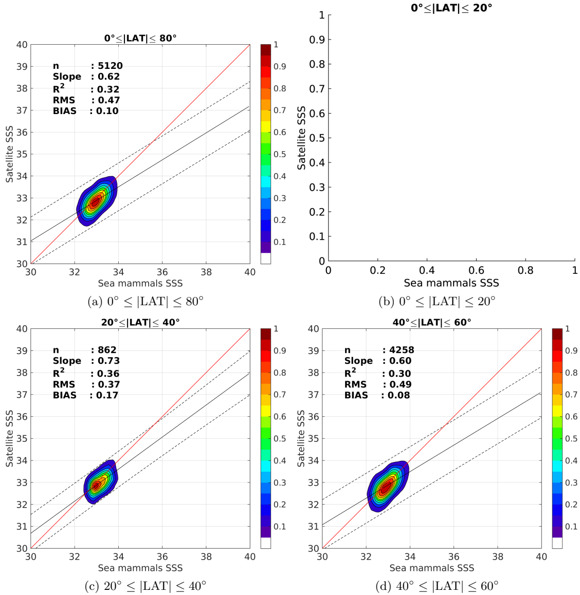
Figure 9: Contour maps of the concentration of SMOS-L3-CATDS-CECOS-LOCEAN-V2.1-9DAYS-25KM SSS (y-axis) versus Sea mammals SSS (x-axis) at match-up pairs for different latitude bands. For each plot, the red line shows x=y . The black thin and dashed lines indicate a linear fit through the data cloud and the \pm 95\% confidence levels, respectively. The number match-up pairs n , the slope and R^2 coefficient of the linear fit, the root mean square (RMS) and the mean bias between satellite and in situ data are indicated for each latitude band in each plots.
