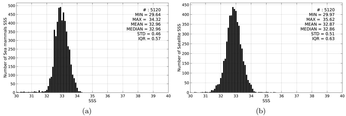
Figure 2: Histograms of SSS from Sea mammals (a) and SMOS-L3-CATDS-CECOS-LOCEAN-V2.1-9DAYS-25KM (b) considering all match-up pairs per bins of 0.1 over the North Pacific Ocean Pi-MEP region and for the full satellite product period.
