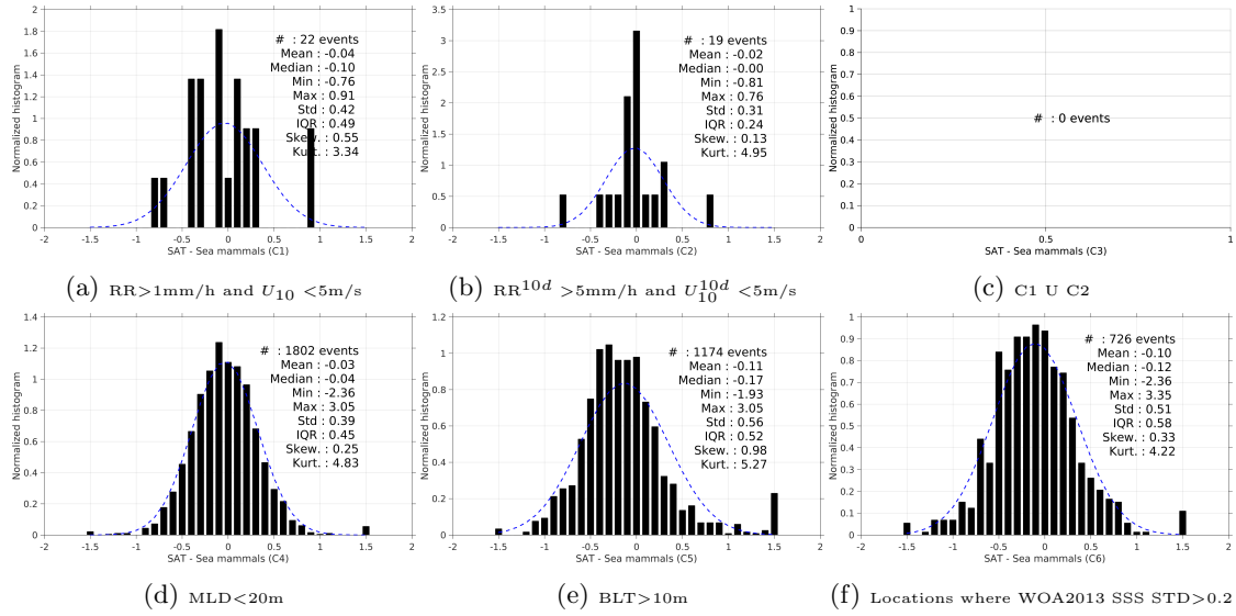
Figure 13: Normalized histogram of \Delta SSS (SMOS-L3-CATDS-CECOS-LOCEAN-V2.1-9DAYS-25KM - Sea mammals) for 6 different subdatasets corresponding to: RR > 1mm/h and U_{10} < 5 m/s (a), RR^{10d} > 5 mm/h and U_{10}^{10d} < 5 m/s (b), C1 U C2 (c), MLD < 20m (d), BLT > 10m (e), Locations where WOA2013 SSS STD > 0.2 (f).
