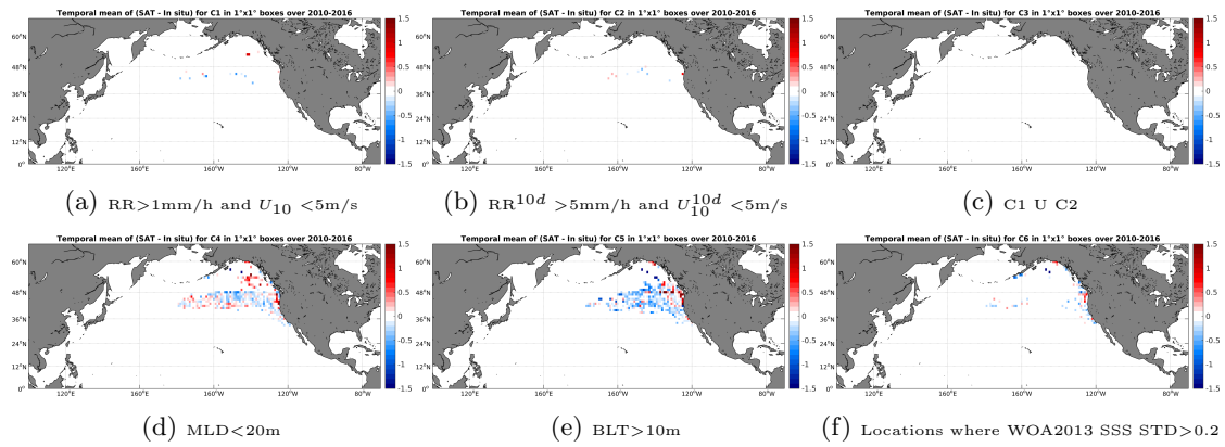
Figure 12: Temporal mean gridded over spatial boxes of size 1^\circ \times 1^\circ of \Delta SSS (SMOS-L3-CATDS-CECOS-LOCEAN-V2.1-9DAYS-25KM - Sea mammals) for 6 different subdatasets corresponding to: RR > 1\text{mm/h} and U_{10} < 5\text{m/s} (a), RR^{10d} > 5\text{mm/h} and U_{10}^{10d} < 5\text{m/s} (b), C1 U C2 (c), MLD < 20\text{m} (d), BLT > 10\text{m} (e), Locations where WOA2013 SSS STD > 0.2 (f).
