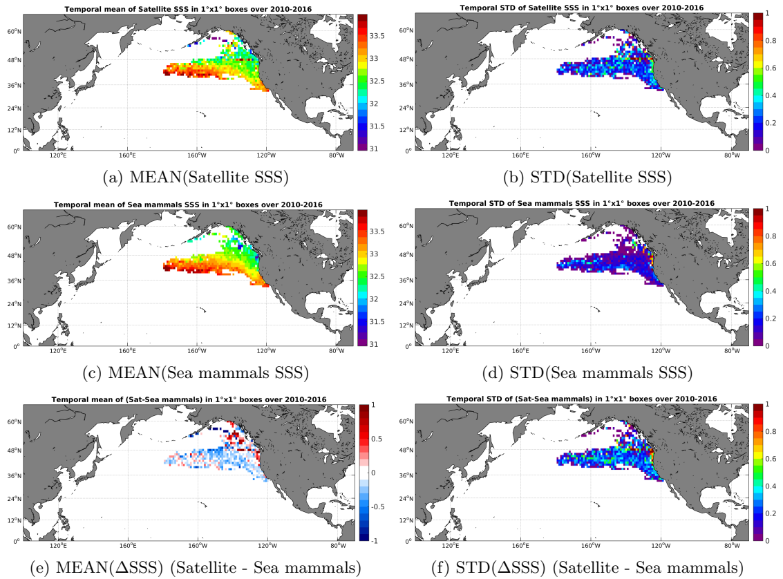
Figure 6: Temporal mean (left) and STD (right) of SSS from SMOS-L3-CATDS-CECOS-LOCEAN-V2.1-9DAYS-25KM (top), Sea mammals (middle), and of \Delta SSS (Satellite - Sea mammals). Only match-up pairs are used to generate these maps.
