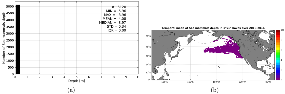
Figure 3: Histograms of the depth of the upper level SSS measurements from Sea mammals in the Match-up DataBase for the North Pacific Ocean Pi-MEP region (a) and temporal mean spatial distribution of pressure of the in situ SSS data over 1^\circ \times 1^\circ boxes and for the full satellite product period (b).
