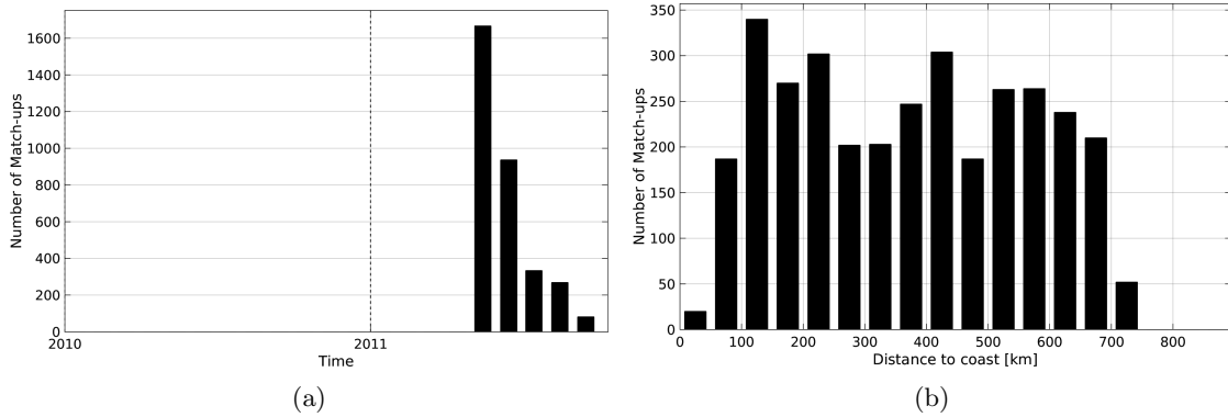
Figure 1: Number of match-ups between Surface drifters and SMOS-L3-CATDS-CECOS-LOCEAN-V2.1-9DAYS-25KM SSS as a function of time (a) and as function of the distance to coast (b) over the North Pacific Ocean Pi-MEP region and for the full satellite product period.
