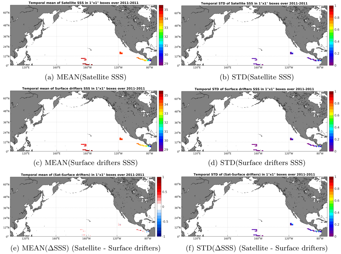
Figure 5: Temporal mean (left) and STD (right) of SSS from SMOS-L3-CATDS-CECOS-LOCEAN-V2.1-9DAYS-25KM (top), Surface drifters (middle), and of \Delta SSS (Satellite - Surface drifters). Only match-up pairs are used to generate these maps.
