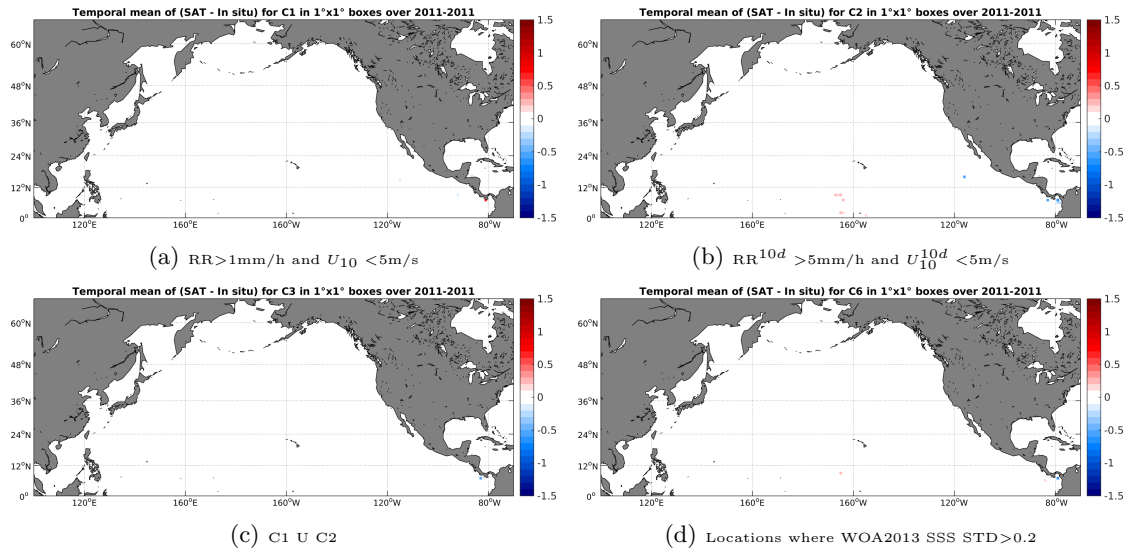
Figure 11: Temporal mean gridded over spatial boxes of size 1^\circ \times 1^\circ of \Delta SSS (SMOS-L3-CATDS-CECOS-LOCEAN-V2.1-9DAYS-25KM - Surface drifters) for 4 different subdatasets corresponding to: RR > 1\text{mm/h} and U_{10} < 5\text{m/s} (a), RR^{10d} > 5\text{mm/h} and U_{10}^{10d} < 5\text{m/s} (b), C1 U C2 (c), Locations where WOA2013 SSS STD > 0.2 (d).
