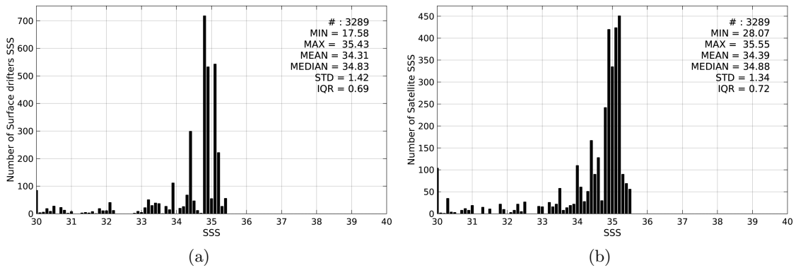
Figure 2: Histograms of SSS from Surface drifters (a) and SMOS-L3-CATDS-CECOS-LOCEAN-V2.1-9DAYS-25KM (b) considering all match-up pairs per bins of 0.1 over the North Pacific Ocean Pi-MEP region and for the full satellite product period.
