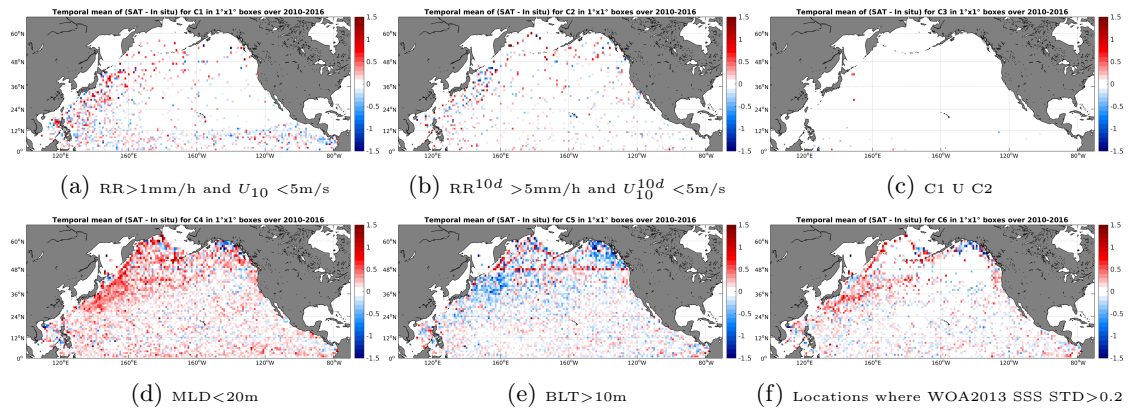
Figure 12: Temporal mean gridded over spatial boxes of size 1^\circ \times 1^\circ of \Delta SSS (SMOS-L3-CATDS-CECOS-LOCEAN-V2.1-9DAYS-25KM - Argo) for 6 different subdatasets corresponding to: RR > 1\text{mm/h} and U_{10} < 5\text{m/s} (a), RR^{10d} > 5\text{mm/h} and U_{10}^{10d} < 5\text{m/s} (b), C1 U C2 (c), MLD < 20\text{m} (d), BLT > 10\text{m} (e), Locations where WOA2013 SSS STD > 0.2 (f).
