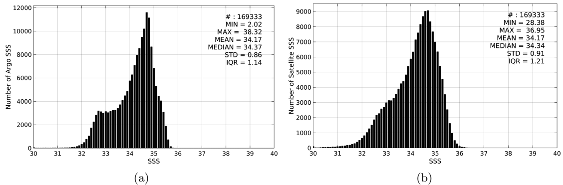
Figure 2: Histograms of SSS from Argo (a) and SMOS-L3-CATDS-CECOS-LOCEAN-V2.1-9DAYS-25KM (b) considering all match-up pairs per bins of 0.1 over the North Pacific Ocean Pi-MEP region and for the full satellite product period.
