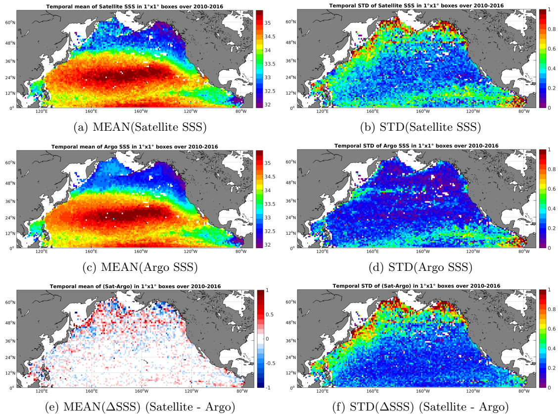
Figure 6: Temporal mean (left) and STD (right) of SSS from SMOS-L3-CATDS-CECOS-LOCEAN-V2.1-9DAYS-25KM (top), Argo (middle), and of \Delta SSS (Satellite - Argo). Only match-up pairs are used to generate these maps.
