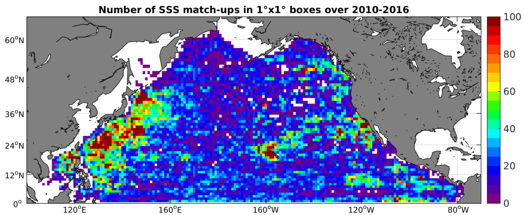
Figure 4: Number of SSS match-ups between Argo SSS and the SMOS-L3-CATDS-CECOS-LOCEAN-V2.1-9DAYS-25KM SSS product for the North Pacific Ocean Pi-MEP region over 1^\circ \times 1^\circ boxes and for the full satellite product period.
