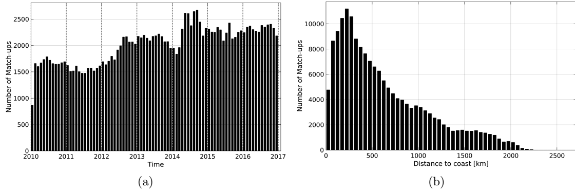
Figure 1: Number of match-ups between Argo and SMOS-L3-CATDS-CECOS-LOCEAN-V2.1-9DAYS-25KM SSS as a function of time (a) and as function of the distance to coast (b) over the North Pacific Ocean Pi-MEP region and for the full satellite product period.
