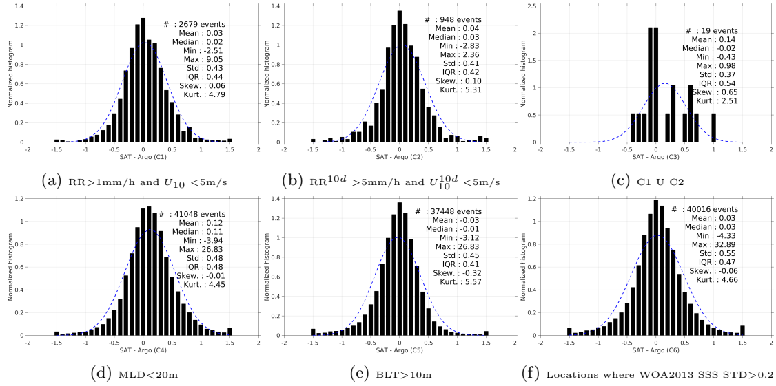
Figure 13: Normalized histogram of \Delta SSS (SMOS-L3-CATDS-CECOS-LOCEAN-V2.1-9DAYS-25KM - Argo) for 6 different subdatasets corresponding to: RR>1mm/h and U_{10} <5m/s (a), RR 10d >5mm/h and U_{10}^{10d} <5m/s (b), C1 U C2 (c),MLD<20m (d),BLT>10m (e),Locations where WOA2013 SSS STD>0.2 (f).
