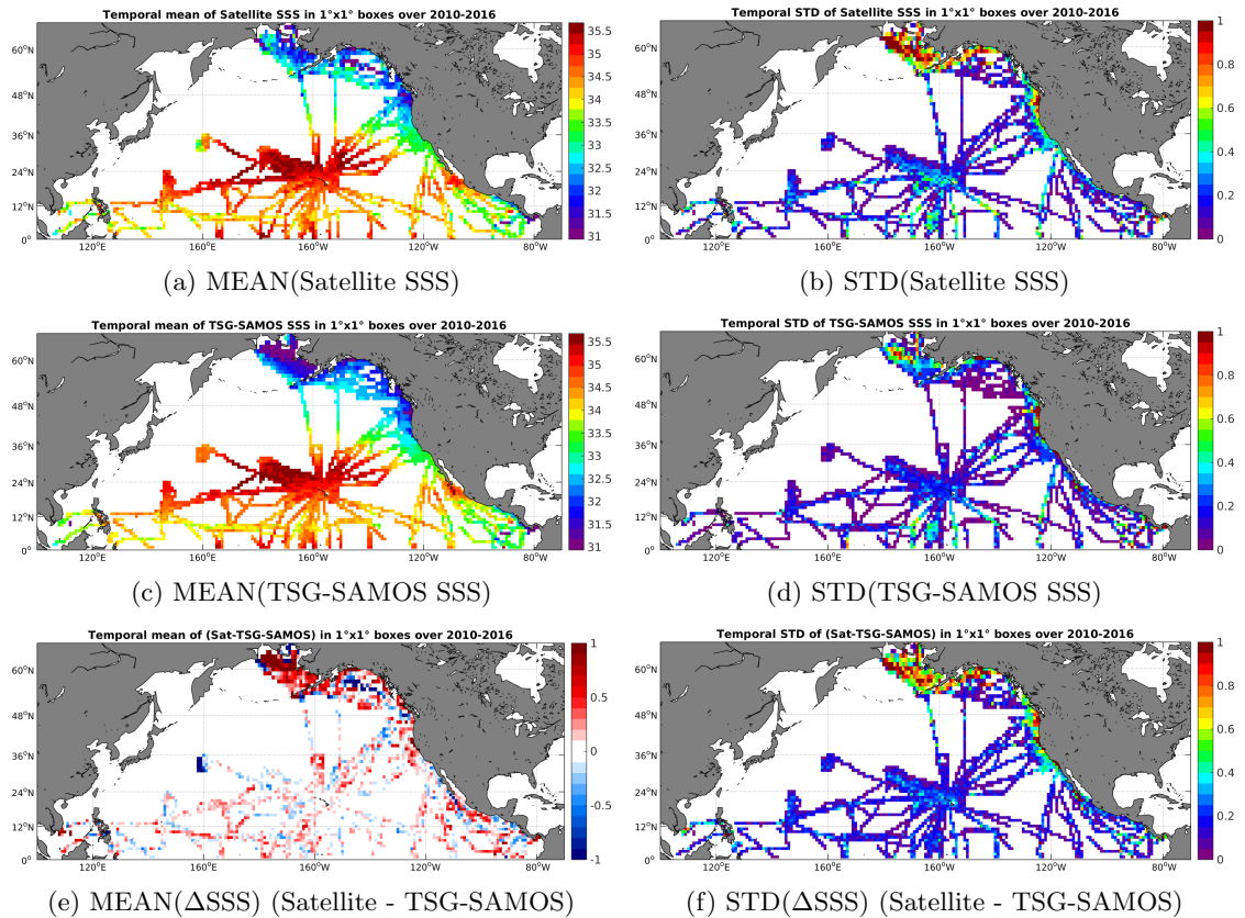
Figure 6: Temporal mean (left) and STD (right) of SSS from SMOS-L3-CATDS-CECOS-LOCEAN-V2-9DAYS-25KM (top), TSG-SAMOS (middle), and of \Delta SSS (Satellite - TSG-SAMOS). Only match-up pairs are used to generate these maps.
