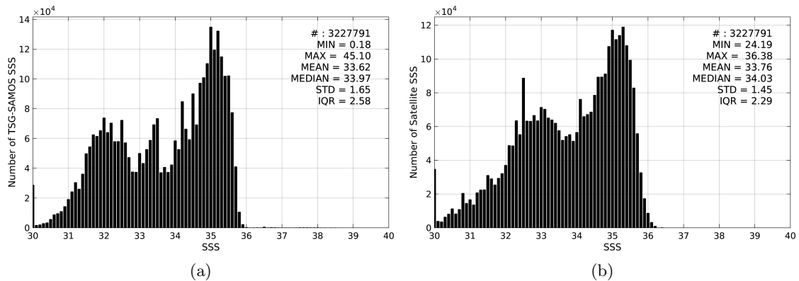
Figure 2: Histograms of SSS from TSG-SAMOS (a) and SMOS-L3-CATDS-CECOS-LOCEAN-V2-9DAYS-25KM (b) considering all match-up pairs per bins of 0.1 over the North Pacific Ocean Pi-MEP region and for the full satellite product period.
