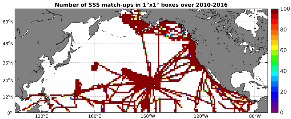
Figure 4: Number of SSS match-ups between TSG-SAMOS SSS and the SMOS-L3-CATDS-CECOS-LOCEAN-V2-9DAYS-25KM SSS product for the North Pacific Ocean Pi-MEP region over 1^\circ \times 1^\circ boxes and for the full satellite product period.
