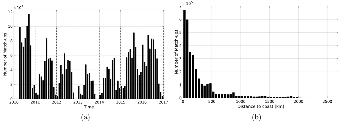
Figure 1: Number of match-ups between TSG-SAMOS and SMOS-L3-CATDS-CECOS-LOCEAN-V2-9DAYS-25KM SSS as a function of time (a) and as function of the distance to coast (b) over the North Pacific Ocean Pi-MEP region and for the full satellite product period.
