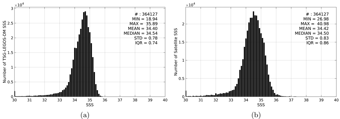
Figure 2: Histograms of SSS from TSG-LEGOS-DM (a) and SMOS-L3-CATDS-CECOS-LOCEAN-V2-9DAYS-25KM (b) considering all match-up pairs per bins of 0.1 over the North Pacific Ocean Pi-MEP region and for the full satellite product period.
