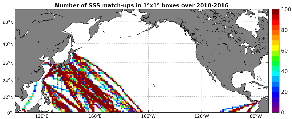
Figure 4: Number of SSS match-ups between TSG-LEGOS-DM SSS and the SMOS-L3-CATDS-CECOS-LOCEAN-V2-9DAYS-25KM SSS product for the North Pacific Ocean Pi-MEP region over 1^\circ \times 1^\circ boxes and for the full satellite product period.
