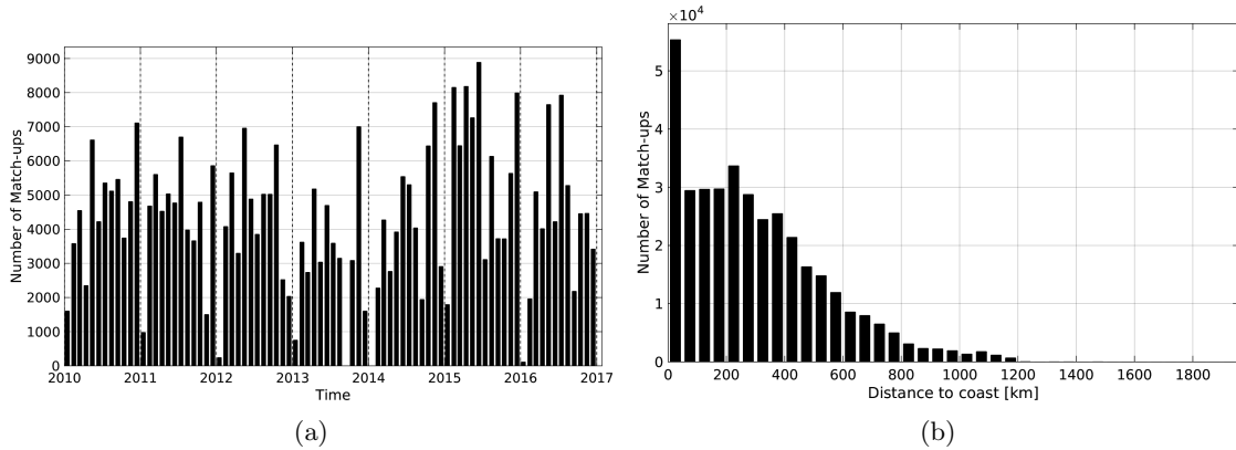
Figure 1: Number of match-ups between TSG-LEGOS-DM and SMOS-L3-CATDS-CECOS-LOCEAN-V2-9DAYS-25KM SSS as a function of time (a) and as function of the distance to coast (b) over the North Pacific Ocean Pi-MEP region and for the full satellite product period.
