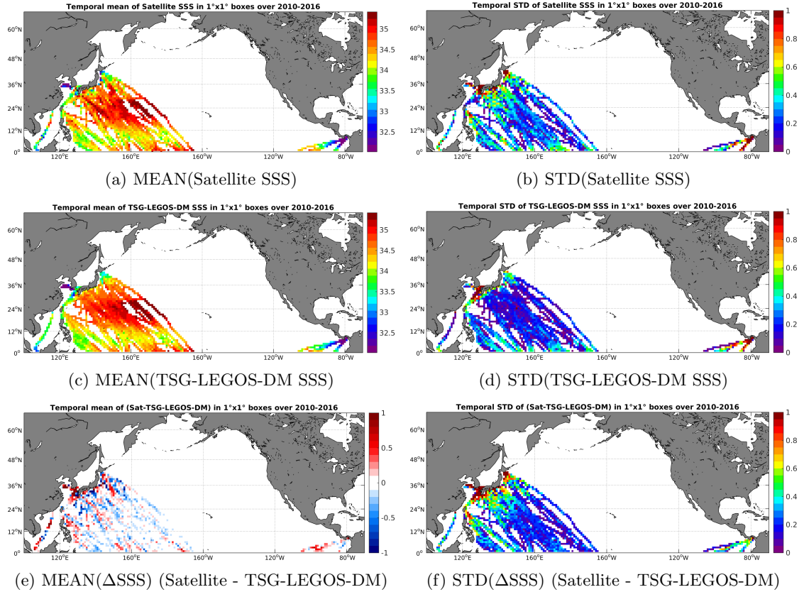
Figure 6: Temporal mean (left) and STD (right) of SSS from SMOS-L3-CATDS-CECOS-LOCEAN-V2-9DAYS-25KM (top), TSG-LEGOS-DM (middle), and of \Delta SSS (Satellite - TSG-LEGOS-DM). Only match-up pairs are used to generate these maps.
