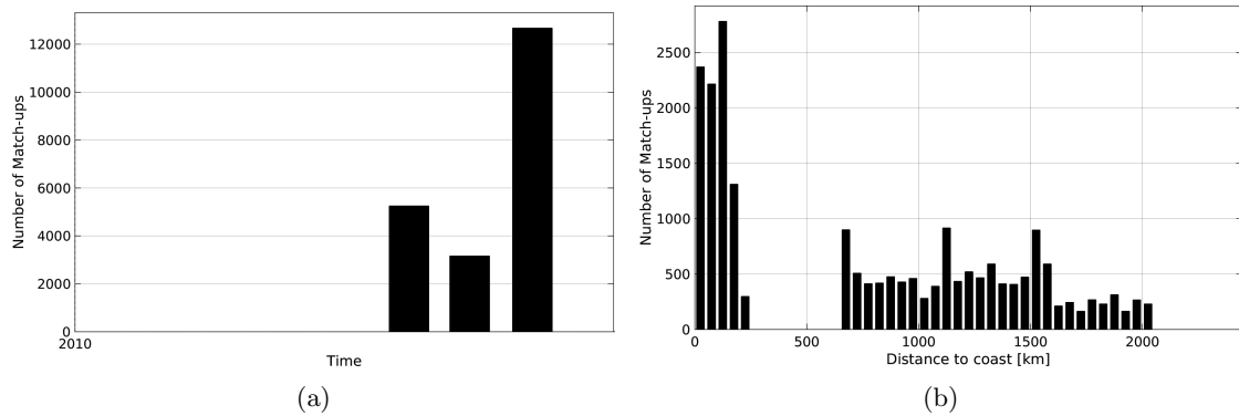
Figure 1: Number of match-ups between TSG-GOSUD-Sailing-ship and SMOS-L3-CATDS-CECOS-LOCEAN-V2-9DAYS-25KM SSS as a function of time (a) and as function of the distance to coast (b) over the North Pacific Ocean Pi-MEP region and for the full satellite product period.
