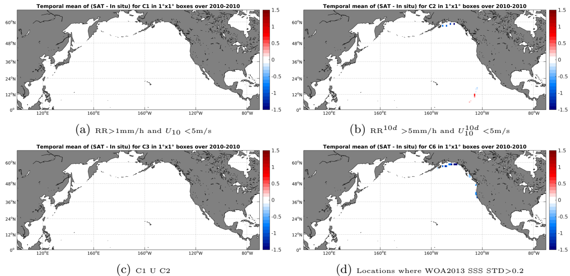
Figure 12: Temporal mean gridded over spatial boxes of size 1^\circ \times 1^\circ of \Delta SSS (SMOS-L3-CATDS-CECOS-LOCEAN-V2-9DAYS-25KM - TSG-GOSUD-Sailing-ship) for 4 different subdatasets corresponding to: RR > 1\text{mm/h} and U_{10} < 5\text{m/s} (a), RR^{10d} > 5\text{mm/h} and U_{10}^{10d} < 5\text{m/s} (b), C1 U C2 (c), Locations where WOA2013 SSS STD > 0.2 (d).
