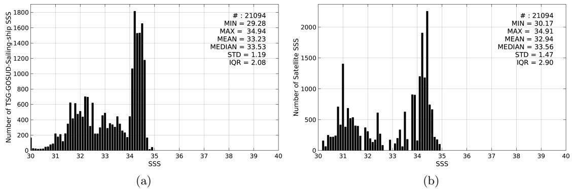
Figure 2: Histograms of SSS from TSG-GOSUD-Sailing-ship (a) and SMOS-L3-CATDS-CECOS-LOCEAN-V2-9DAYS-25KM (b) considering all match-up pairs per bins of 0.1 over the North Pacific Ocean Pi-MEP region and for the full satellite product period.
