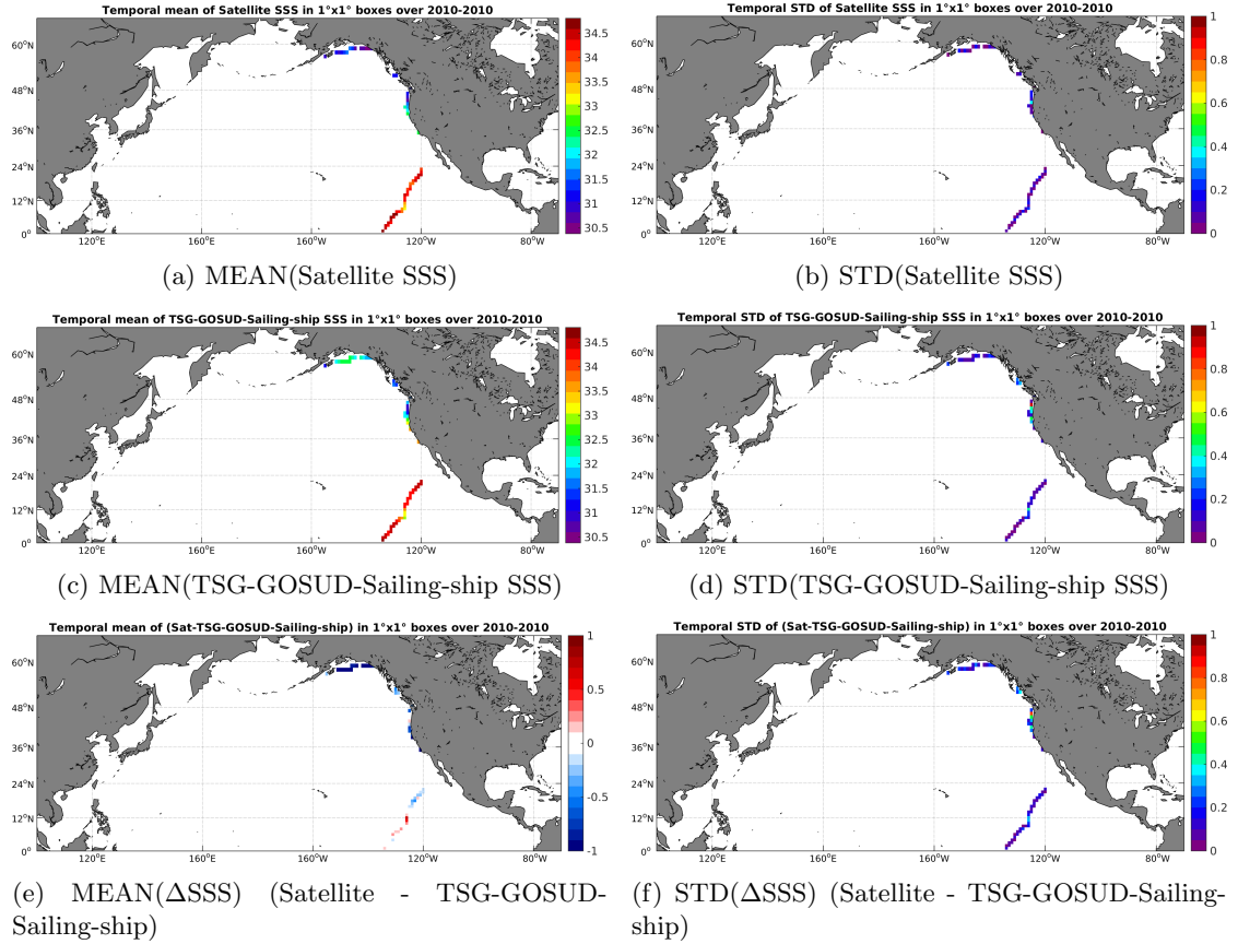
Figure 6: Temporal mean (left) and STD (right) of SSS from SMOS-L3-CATDS-CECOS-LOCEAN-V2-9DAYS-25KM (top), TSG-GOSUD-Sailing-ship (middle), and of \Delta SSS (Satellite - TSG-GOSUD-Sailing-ship). Only match-up pairs are used to generate these maps.
