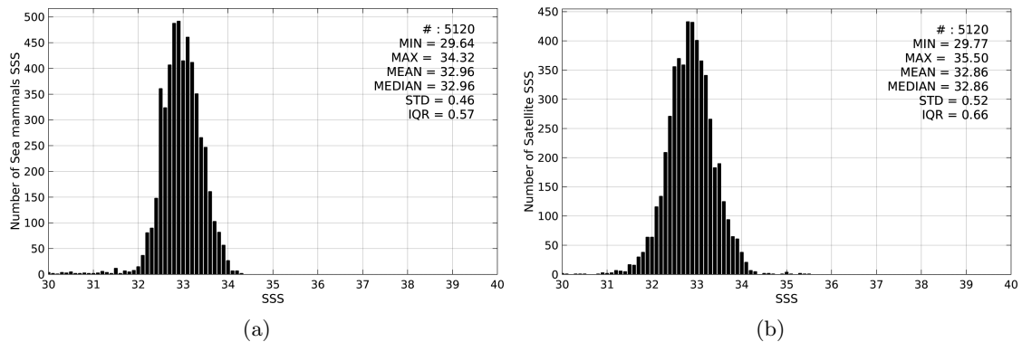
Figure 2: Histograms of SSS from Sea mammals (a) and SMOS-L3-CATDS-CECOS-LOCEAN-V2-9DAYS-25KM (b) considering all match-up pairs per bins of 0.1 over the North Pacific Ocean Pi-MEP region and for the full satellite product period.
