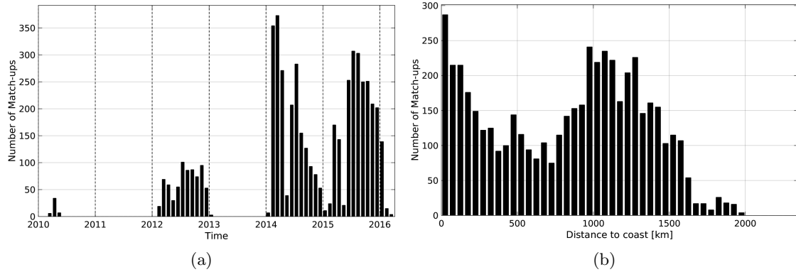
Figure 1: Number of match-ups between Sea mammals and SMOS-L3-CATDS-CECOS-LOCEAN-V2-9DAYS-25KM SSS as a function of time (a) and as function of the distance to coast (b) over the North Pacific Ocean Pi-MEP region and for the full satellite product period.
