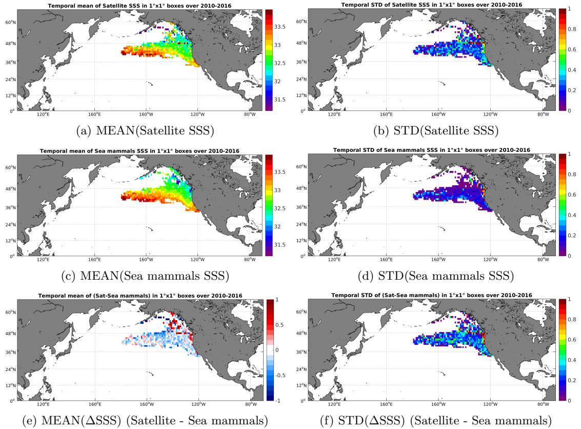
Figure 6: Temporal mean (left) and STD (right) of SSS from SMOS-L3-CATDS-CECOS-LOCEAN-V2-9DAYS-25KM (top), Sea mammals (middle), and of \Delta SSS (Satellite - Sea mammals). Only match-up pairs are used to generate these maps.
