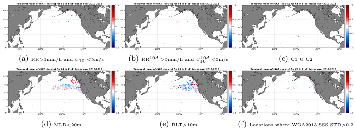
Figure 12: Temporal mean gridded over spatial boxes of size 1^\circ \times 1^\circ of \Delta SSS (SMOS-L3-CATDS-CECOS-LOCEAN-V2-9DAYS-25KM - Sea mammals) for 6 different subdatasets corresponding to: RR > 1\text{mm/h} and U_{10} < 5\text{m/s} (a), RR^{10d} > 5\text{mm/h} and U_{10}^{10d} < 5\text{m/s} (b), C1 U C2 (c), MLD < 20\text{m} (d), BLT > 10\text{m} (e), Locations where WOA2013 SSS STD > 0.2 (f).
