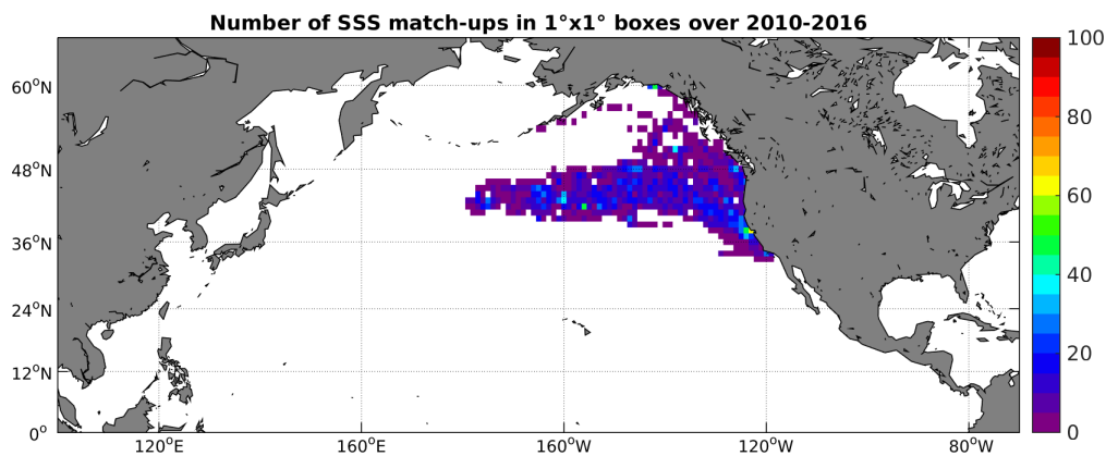
Figure 4: Number of SSS match-ups between Sea mammals SSS and the SMOS-L3-CATDS-CECOS-LOCEAN-V2-9DAYS-25KM SSS product for the North Pacific Ocean Pi-MEP region over 1^\circ \times 1^\circ boxes and for the full satellite product period.
