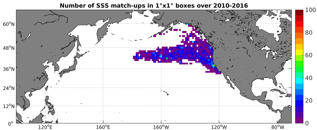
Figure 4: Number of SSS match-ups between Sea mammals SSS and the SMOS-L3-CATDS-CECOS-LOCEAN-V2-9DAYS-25KM SSS product for the North Pacific Ocean Pi-MEP region over 1°x1° boxes and for the full satellite product period.
