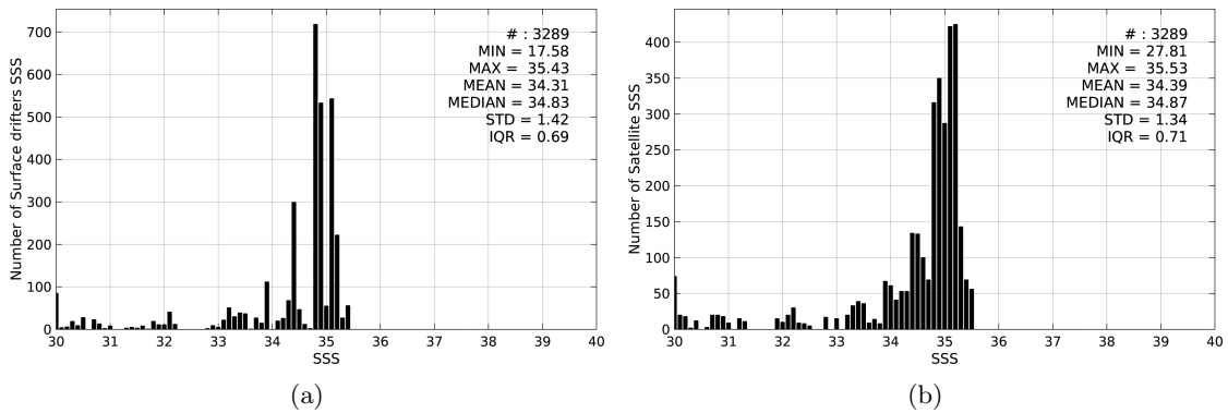
Figure 2: Histograms of SSS from Surface drifters (a) and SMOS-L3-CATDS-CECOS-LOCEAN-V2-9DAYS-25KM (b) considering all match-up pairs per bins of 0.1 over the North Pacific Ocean Pi-MEP region and for the full satellite product period.
