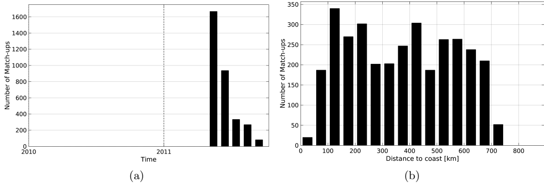
Figure 1: Number of match-ups between Surface drifters and SMOS-L3-CATDS-CECOS-LOCEAN-V2-9DAYS-25KM SSS as a function of time (a) and as function of the distance to coast (b) over the North Pacific Ocean Pi-MEP region and for the full satellite product period.
