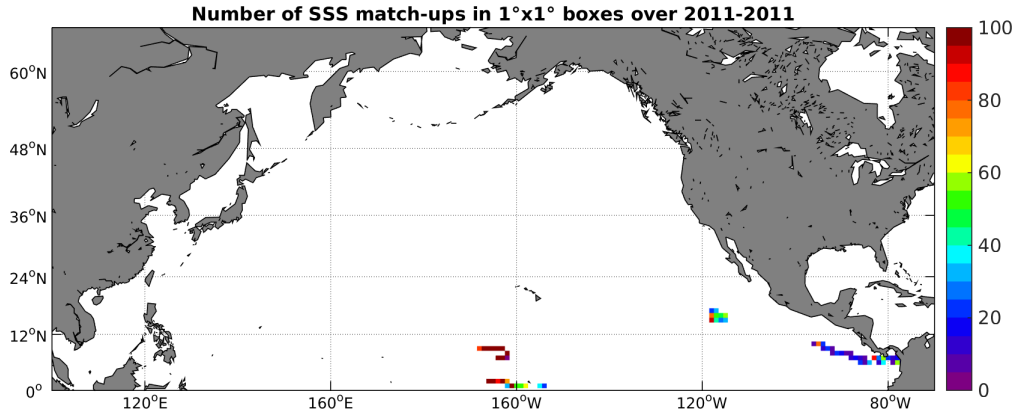
Figure 3: Number of SSS match-ups between Surface drifters SSS and the SMOS-L3-CATDS-CECOS-LOCEAN-V2-9DAYS-25KM SSS product for the North Pacific Ocean Pi-MEP region over 1^\circ \times 1^\circ boxes and for the full satellite product period.
