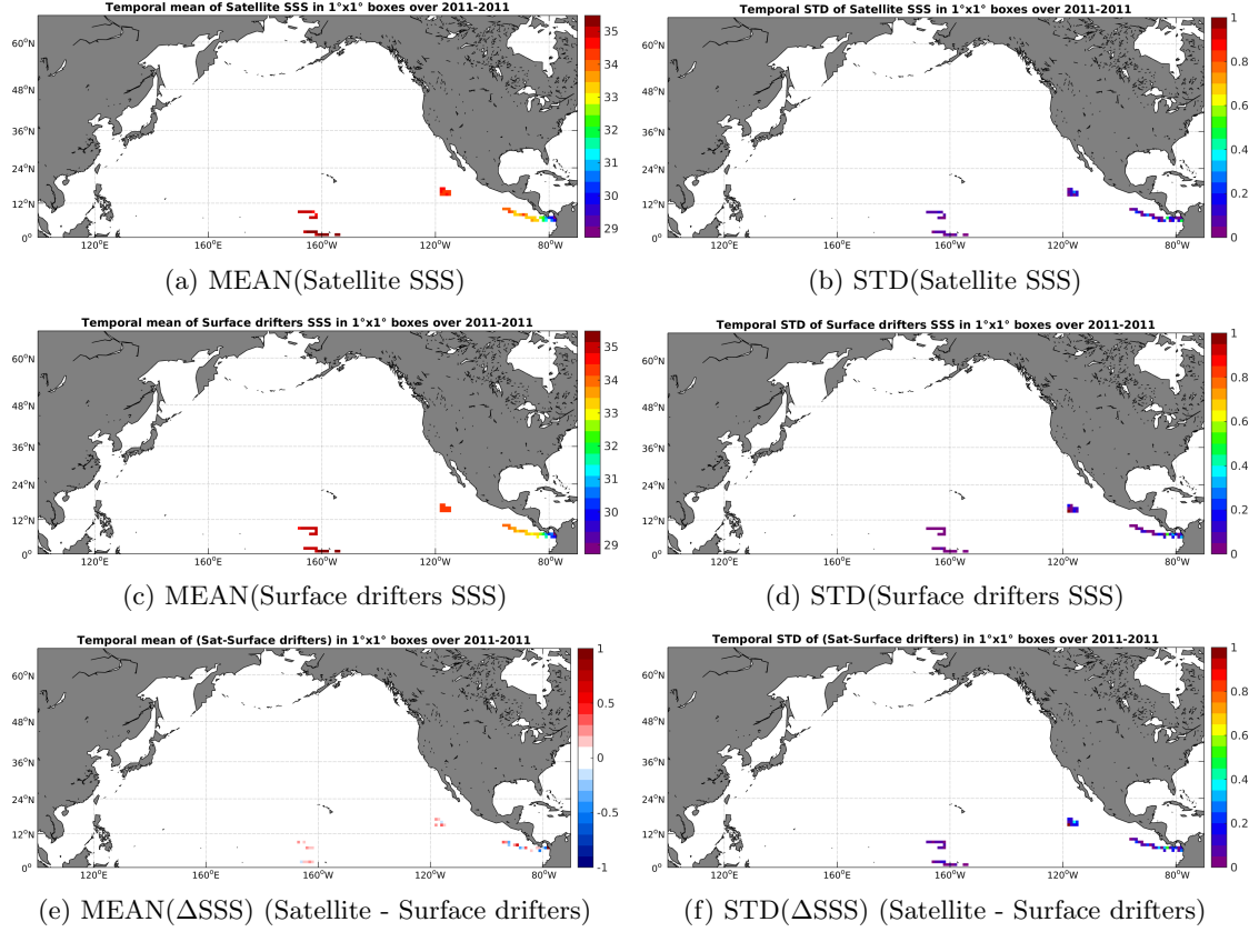
Figure 5: Temporal mean (left) and STD (right) of SSS from SMOS-L3-CATDS-CECOS-LOCEAN-V2-9DAYS-25KM (top), Surface drifters (middle), and of \Delta SSS (Satellite - Surface drifters). Only match-up pairs are used to generate these maps.
