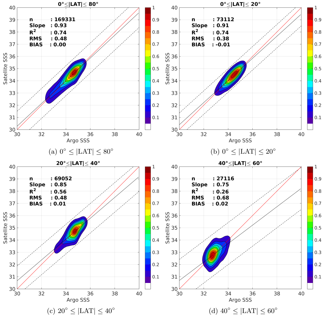
Figure 9: Contour maps of the concentration of SMOS-L3-CATDS-CECOS-LOCEAN-V2-9DAYS-25KM SSS (y-axis) versus Argo SSS (x-axis) at match-up pairs for different latitude bands. For each plot, the red line shows x=y . The black thin and dashed lines indicate a linear fit through the data cloud and the \pm 95\% confidence levels, respectively. The number match-up pairs n , the slope and R^2 coefficient of the linear fit, the root mean square (RMS) and the mean bias between satellite and in situ data are indicated for each latitude band in each plots.
