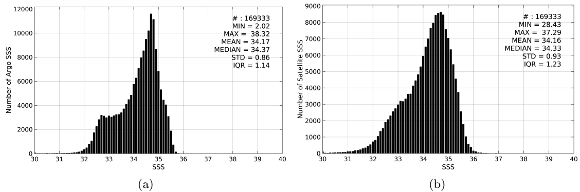
Figure 2: Histograms of SSS from Argo (a) and SMOS-L3-CATDS-CECOS-LOCEAN-V2-9DAYS-25KM (b) considering all match-up pairs per bins of 0.1 over the North Pacific Ocean Pi-MEP region and for the full satellite product period.
