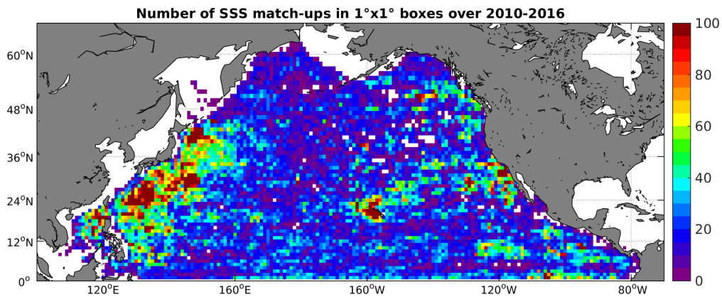
Figure 4: Number of SSS match-ups between Argo SSS and the SMOS-L3-CATDS-CECOS-LOCEAN-V2-9DAYS-25KM SSS product for the North Pacific Ocean Pi-MEP region over 1^\circ \times 1^\circ boxes and for the full satellite product period.
