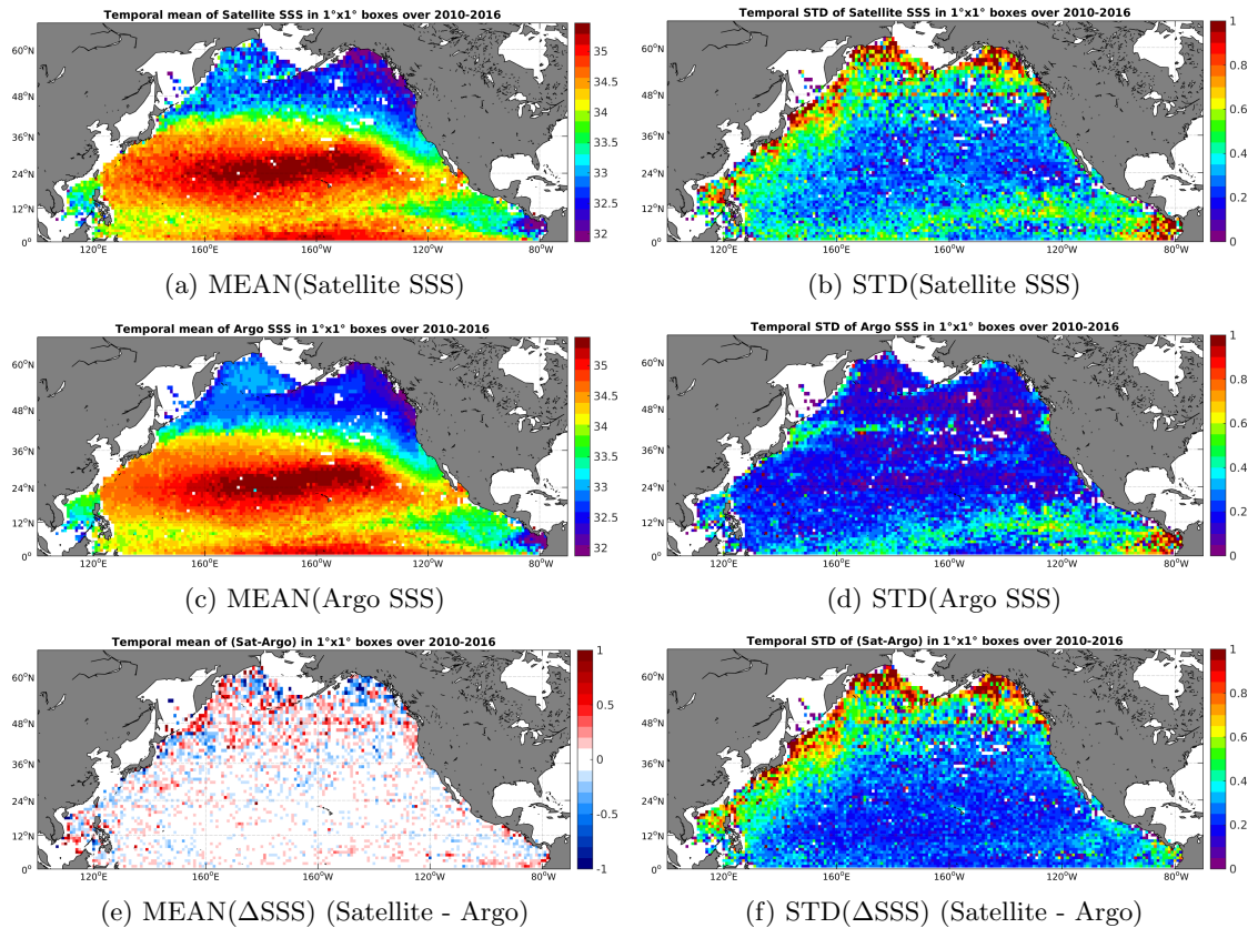
Figure 6: Temporal mean (left) and STD (right) of SSS from SMOS-L3-CATDS-CECOS-LOCEAN-V2-9DAYS-25KM (top), Argo (middle), and of \Delta SSS (Satellite - Argo). Only match-up pairs are used to generate these maps.
