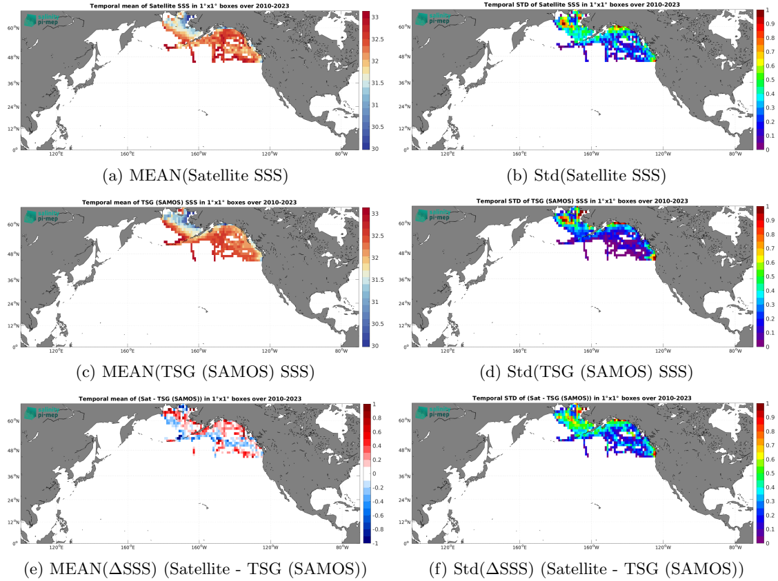
Figure 7: Temporal mean (left) and Std (right) of SSS from SMOS SSS L3 Arctic v2 - 9 Days (CATDS-CEC-LOCEAN) (top), TSG (SAMOS) (middle), and of \Delta\text{SSS} (Satellite - TSG (SAMOS)). Only match-up pairs are used to generate these maps.
