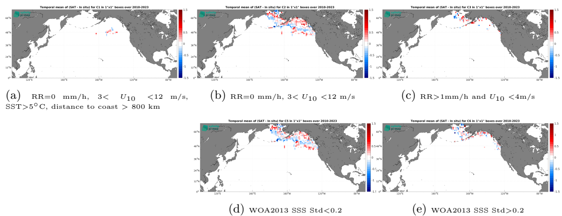
Figure 14: Temporal mean gridded over spatial boxes of size 1^\circ \times 1^\circ of \Delta SSS (SMOS SSS L3 Arctic v2 - 9 Days (CATDS-CEC-LOCEAN) - TSG (SAMOS)) for 5 different subdatasets corresponding to:RR=0 mm/h, 3 < U_{10} < 12 m/s, SST>5°C, distance to coast > 800 km (a), RR=0 mm/h, 3 < U_{10} < 12 m/s (b), RR>1mm/h and U_{10} < 4 m/s (c), WOA2013 SSS Std<0.2 (d), WOA2013 SSS Std>0.2 (e).
