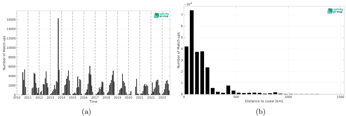
Figure 2: Number of match-ups between TSG (SAMOS) and SMOS SSS L3 Arctic v2 - 9 Days (CATDS-CEC-LOCEAN) SSS as a function of time (a) and as function of the distance to coast (b) over the North Pacific Ocean Pi-MEP region and for the full satellite product period.
