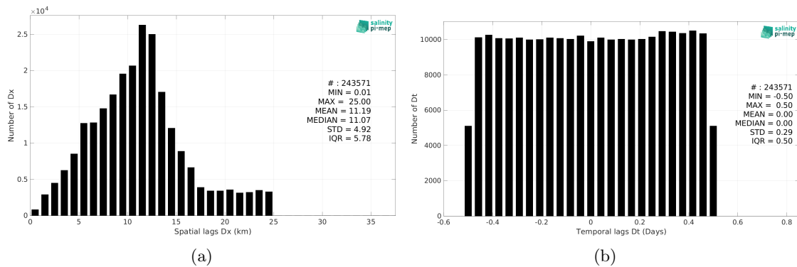
Figure 6: Histograms of the spatial (a) and temporal (b) lags between the location/time of the TSG (SAMOS) measurement and the date of the corresponding SMOS SSS L3 Arctic v2 - 9 Days (CATDS-CEC-LOCEAN) SSS pixel.
