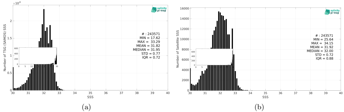
Figure 3: Histograms of SSS from TSG (SAMOS) (a) and SMOS SSS L3 Arctic v2 - 9 Days (CATDS-CEC-LOCEAN) (b) considering all match-up pairs per bins of 0.1 over the North Pacific Ocean Pi-MEP region and for the full satellite product period.
