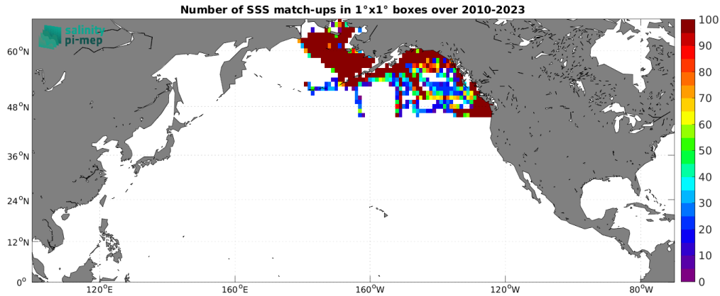
Figure 5: Number of SSS match-ups between TSG (SAMOS) SSS and the SMOS SSS L3 Arctic v2 - 9 Days (CATDS-CEC-LOCEAN) SSS product for the North Pacific Ocean Pi-MEP region over 1^\circ \times 1^\circ boxes and for the full satellite product period.
