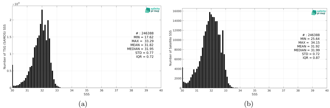
Figure 2: Histograms of SSS from TSG (SAMOS) (a) and SMOS SSS L3 Arctic v2 - 9 Days (CATDS-CEC-LOCEAN) (b) considering all match-up pairs per bins of 0.1 over the North Pacific Ocean Pi-MEP region and for the full satellite product period.
