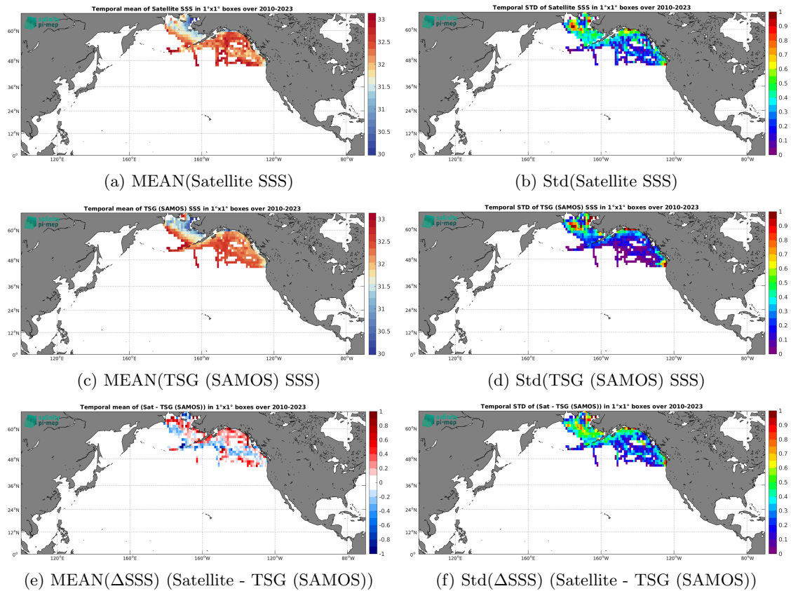
Figure 6: Temporal mean (left) and Std (right) of SSS from SMOS SSS L3 Arctic v2 - 9 Days (CATDS-CEC-LOCEAN) (top), TSG (SAMOS) (middle), and of \Delta SSS (Satellite - TSG (SAMOS)). Only match-up pairs are used to generate these maps.
