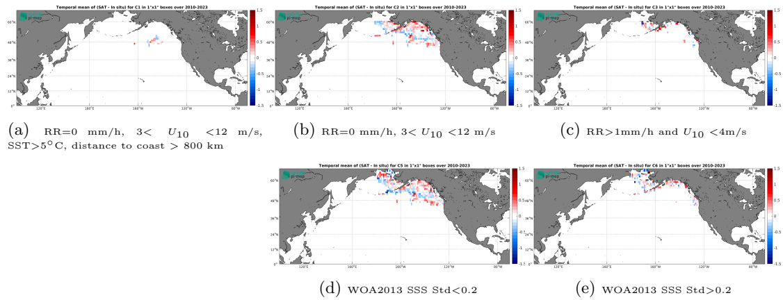
Figure 12: Temporal mean gridded over spatial boxes of size 1^{\circ}\times 1^{\circ} of \Delta\text{SSS} (SMOS SSS L3 Arctic v2 - 9 Days (CATDS-CEC-LOCEAN) - TSG (SAMOS)) for 5 different subdatasets corresponding to:RR=0 mm/h, 3 < U_{10} < 12 m/s, SST > 5^{\circ}\text{C} , distance to coast > 800 km (a), RR=0 mm/h, 3 < U_{10} < 12 m/s (b), RR > 1 mm/h and U_{10} < 4 m/s (c), WOA2013 SSS Std < 0.2 (d), WOA2013 SSS Std > 0.2 (e).
