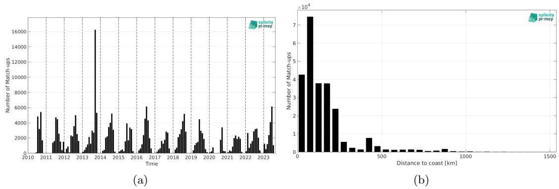
Figure 1: Number of match-ups between TSG (SAMOS) and SMOS SSS L3 Arctic v2 - 9 Days (CATDS-CEC-LOCEAN) SSS as a function of time (a) and as function of the distance to coast (b) over the North Pacific Ocean Pi-MEP region and for the full satellite product period.
