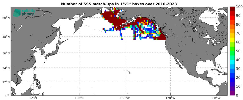
Figure 4: Number of SSS match-ups between TSG (SAMOS) SSS and the SMOS SSS L3 Arctic v2 - 9 Days (CATDS-CEC-LOCEAN) SSS product for the North Pacific Ocean Pi-MEP region over 1^\circ \times 1^\circ boxes and for the full satellite product period.
