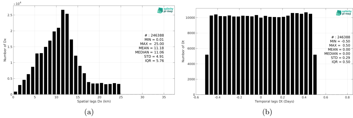
Figure 5: Histograms of the spatial (a) and temporal (b) lags between the location/time of the TSG (SAMOS) measurement and the date of the corresponding SMOS SSS L3 Arctic v2 - 9 Days (CATDS-CEC-LOCEAN) SSS pixel.
