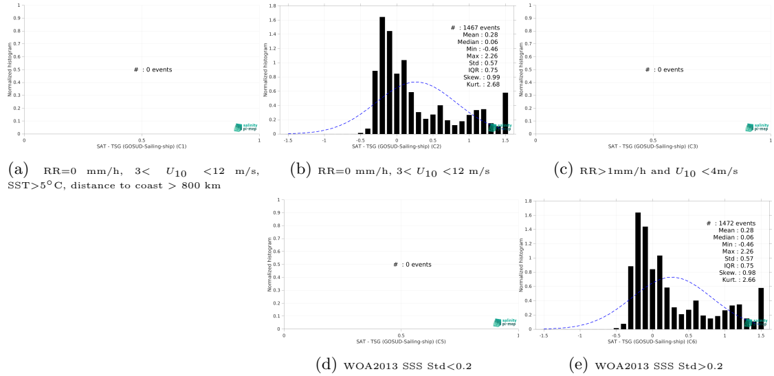
Figure 15: Normalized histogram of \Delta SSS (SMOS SSS L3 Arctic v2 - 9 Days (CATDS-CEC-LOCEAN) - TSG (GOSUD-Sailing-ship)) for 5 different subdatasets corresponding to: RR=0 mm/h, 3 < U_{10} < 12 m/s, SST > 5°C, distance to coast > 800 km (a), RR=0 mm/h, 3 < U_{10} < 12 m/s (b), RR > 1mm/h and U_{10} < 4 m/s (c), WOA2013 SSS Std < 0.2 (d), WOA2013 SSS Std > 0.2 (e).
