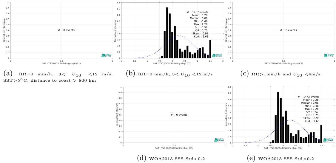
Figure 13: Normalized histogram of \Delta SSS (SMOS SSS L3 Arctic v2 - 9 Days (CATDS-CEC-LOCEAN) - TSG (GOSUD-Sailing-ship)) for 5 different subdatasets corresponding to: RR=0 mm/h, 3 < U_{10} < 12 m/s, SST > 5°C, distance to coast > 800 km (a), RR=0 mm/h, 3 < U_{10} < 12 m/s (b), RR > 1mm/h and U_{10} < 4 m/s (c), WOA2013 SSS Std < 0.2 (d), WOA2013 SSS Std > 0.2 (e).
