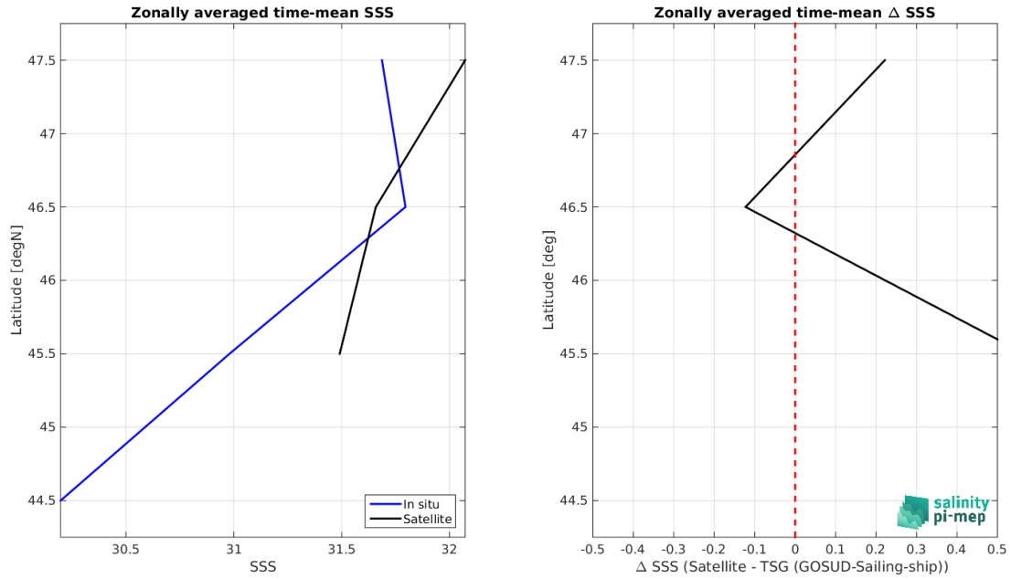
Figure 8: Left panel: Zonal mean SSS from SMOS SSS L3 Arctic v2 - 9 Days (CATDS-CEC-LOCEAN) satellite product (black) and from TSG (GOSUD-Sailing-ship) (blue). Right panel: Zonal mean of \Delta SSS (Satellite - TSG (GOSUD-Sailing-ship)) for all the collected Pi-MEP match-up pairs estimated over the full satellite product period.
