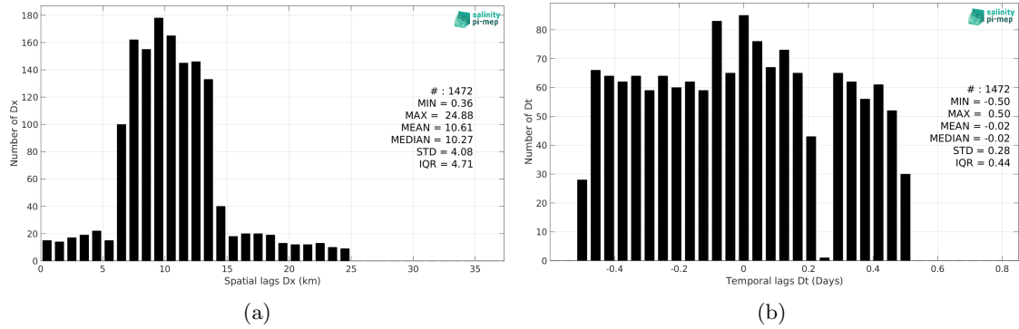
Figure 5: Histograms of the spatial (a) and temporal (b) lags between the location/time of the TSG (GOSUD-Sailing-ship) measurement and the date of the corresponding SMOS SSS L3 Arctic v2 - 9 Days (CATDS-CEC-LOCEAN) SSS pixel.
