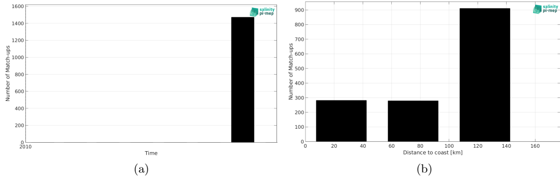
Figure 1: Number of match-ups between TSG (GOSUD-Sailing-ship) and SMOS SSS L3 Arctic v2 - 9 Days (CATDS-CEC-LOCEAN) SSS as a function of time (a) and as function of the distance to coast (b) over the North Pacific Ocean Pi-MEP region and for the full satellite product period.
