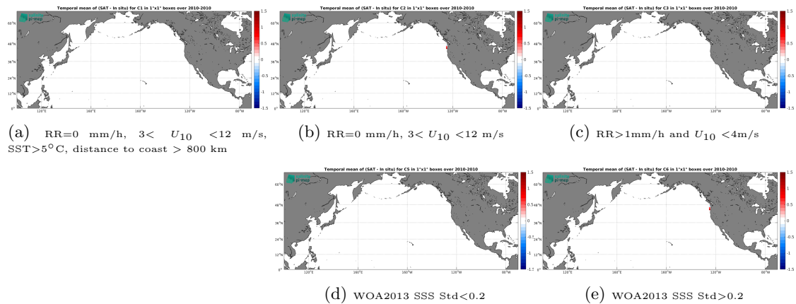
Figure 12: Temporal mean gridded over spatial boxes of size 1^{\circ}\times 1^{\circ} of \Delta SSS (SMOS SSS L3 Arctic v2 - 9 Days (CATDS-CEC-LOCEAN) - TSG (GOSUD-Sailing-ship)) for 5 different subdatasets corresponding to:RR=0 mm/h, 3 < U_{10} < 12 m/s, SST > 5^{\circ}\text{C} , distance to coast > 800 km (a), RR=0 mm/h, 3 < U_{10} < 12 m/s (b), RR > 1 mm/h and U_{10} < 4 m/s (c), WOA2013 SSS Std < 0.2 (d), WOA2013 SSS Std > 0.2 (e).
