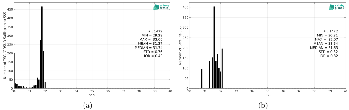
Figure 2: Histograms of SSS from TSG (GOSUD-Sailing-ship) (a) and SMOS SSS L3 Arctic v2 - 9 Days (CATDS-CEC-LOCEAN) (b) considering all match-up pairs per bins of 0.1 over the North Pacific Ocean Pi-MEP region and for the full satellite product period.
