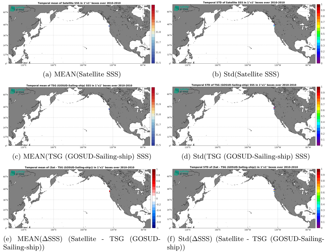
Figure 6: Temporal mean (left) and Std (right) of SSS from SMOS SSS L3 Arctic v2 - 9 Days (CATDS-CEC-LOCEAN) (top), TSG (GOSUD-Sailing-ship) (middle), and of \Delta SSS (Satellite - TSG (GOSUD-Sailing-ship)). Only match-up pairs are used to generate these maps.
