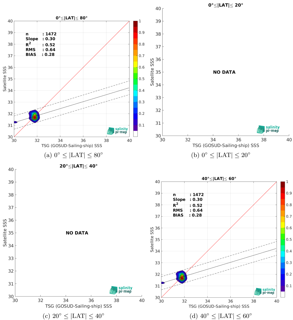
Figure 9: Contour maps of the concentration of SMOS SSS L3 Arctic v2 - 9 Days (CATDS-CEC-LOCEAN) SSS (y-axis) versus TSG (GOSUD-Sailing-ship) SSS (x-axis) at match-up pairs for different latitude bands. For each plot, the red line shows x=y . The black thin and dashed lines indicate a linear fit through the data cloud and the \pm 95\% confidence levels, respectively. The number match-up pairs n , the slope and R^2 coefficient of the linear fit, the root mean square (RMS) and the mean bias between satellite and in situ data are indicated for each latitude band in each plots.
