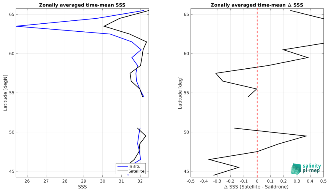
Figure 8: Left panel: Zonal mean SSS from SMOS SSS L3 Arctic v2 - 9 Days (CATDS-CEC-LOCEAN) satellite product (black) and from Sairdron (blue). Right panel: Zonal mean of \Delta SSS (Satellite - Sairdron) for all the collected Pi-MEP match-up pairs estimated over the full satellite product period.
