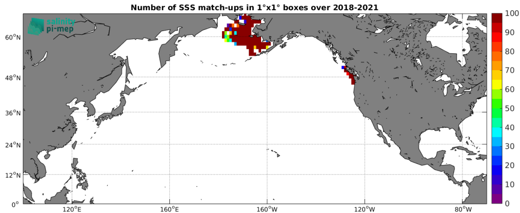
Figure 4: Number of SSS match-ups between Saildrone SSS and the SMOS SSS L3 Arctic v2 - 9 Days (CATDS-CEC-LOCEAN) SSS product for the North Pacific Ocean Pi-MEP region over 1^\circ \times 1^\circ boxes and for the full satellite product period.
