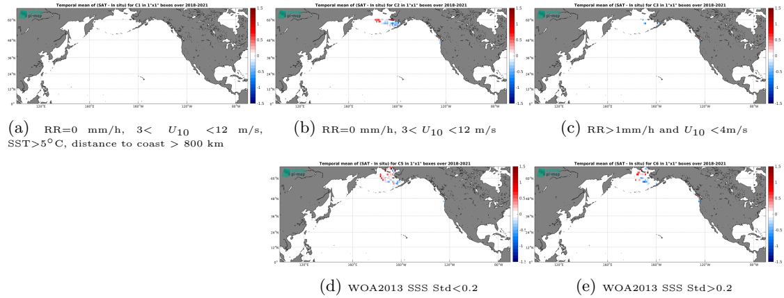
Figure 12: Temporal mean gridded over spatial boxes of size 1^{\circ}\times 1^{\circ} of \Delta\text{SSS} (SMOS SSS L3 Arctic v2 - 9 Days (CATDS-CEC-LOCEAN) - Saildrone) for 5 different subdatasets corresponding to:RR=0 mm/h, 3 < U_{10} < 12 m/s, SST > 5^{\circ}\text{C} , distance to coast > 800 km (a), RR=0 mm/h, 3 < U_{10} < 12 m/s (b), RR > 1 mm/h and U_{10} < 4 m/s (c), WOA2013 SSS Std < 0.2 (d), WOA2013 SSS Std > 0.2 (e).
