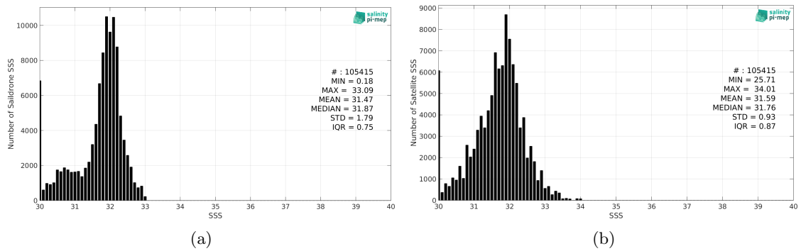
Figure 2: Histograms of SSS from Saildrone (a) and SMOS SSS L3 Arctic v2 - 9 Days (CATDS-CEC-LOCEAN) (b) considering all match-up pairs per bins of 0.1 over the North Pacific Ocean Pi-MEP region and for the full satellite product period.
