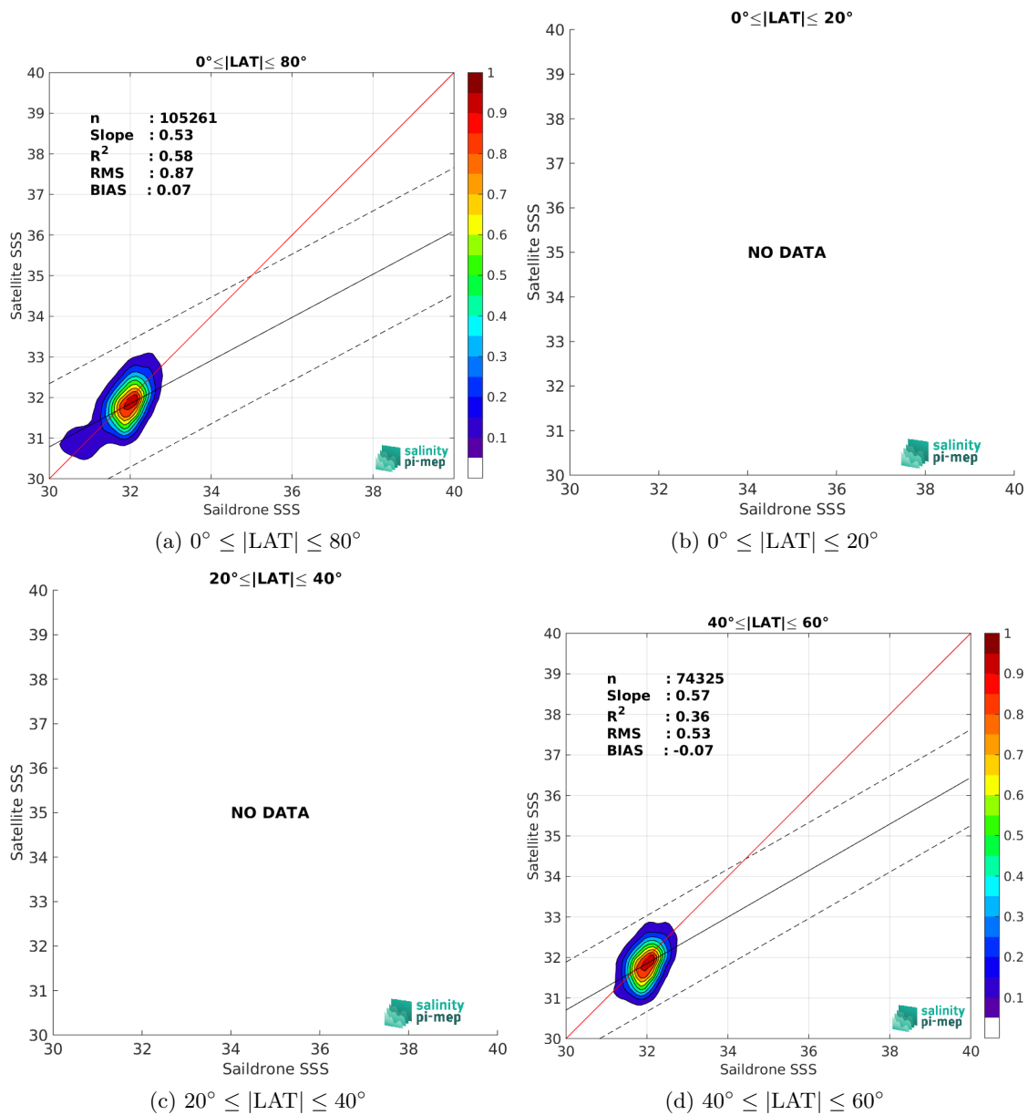
Figure 9: Contour maps of the concentration of SMOS SSS L3 Arctic v2 - 9 Days (CATDS-CEC-LOCEAN) SSS (y-axis) versus Saildrone SSS (x-axis) at match-up pairs for different latitude bands. For each plot, the red line shows x=y . The black thin and dashed lines indicate a linear fit through the data cloud and the \pm 95\% confidence levels, respectively. The number match-up pairs n , the slope and R^2 coefficient of the linear fit, the root mean square (RMS) and the mean bias between satellite and in situ data are indicated for each latitude band in each plots.
