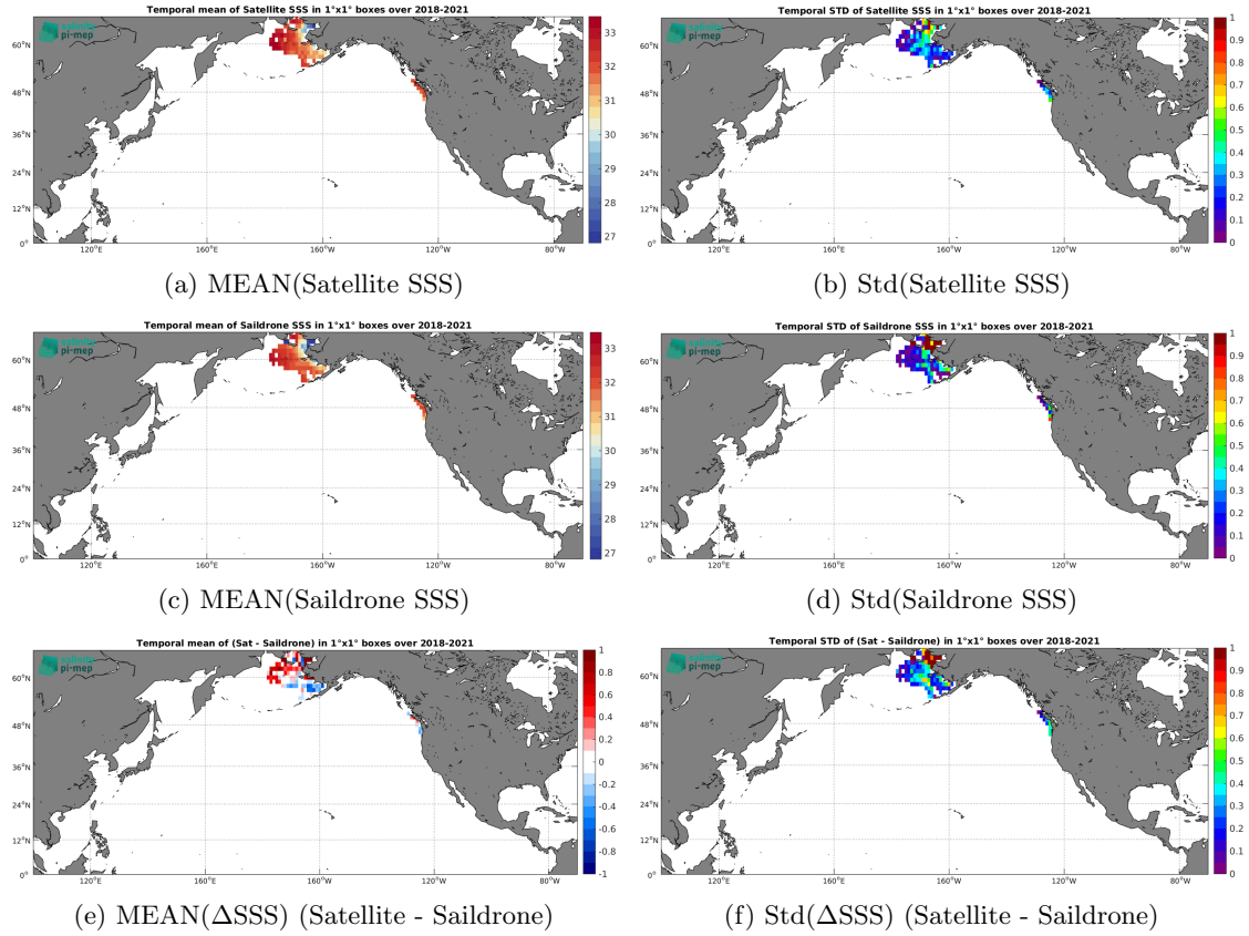
Figure 6: Temporal mean (left) and Std (right) of SSS from SMOS SSS L3 Arctic v2 - 9 Days (CATDS-CEC-LOCEAN) (top), Saildrone (middle), and of \Delta SSS (Satellite - Saildrone). Only match-up pairs are used to generate these maps.
