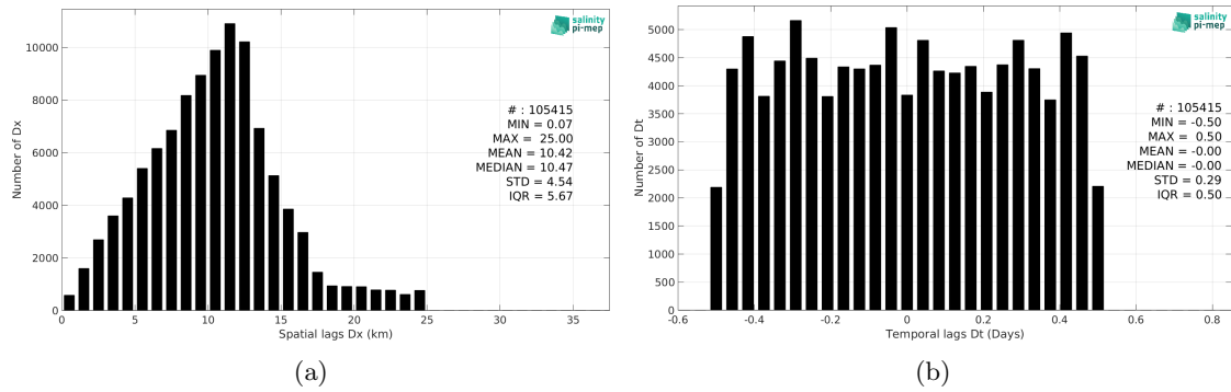
Figure 5: Histograms of the spatial (a) and temporal (b) lags between the location/time of the Saildrone measurement and the date of the corresponding SMOS SSS L3 Arctic v2 - 9 Days (CATDS-CEC-LOCEAN) SSS pixel.
