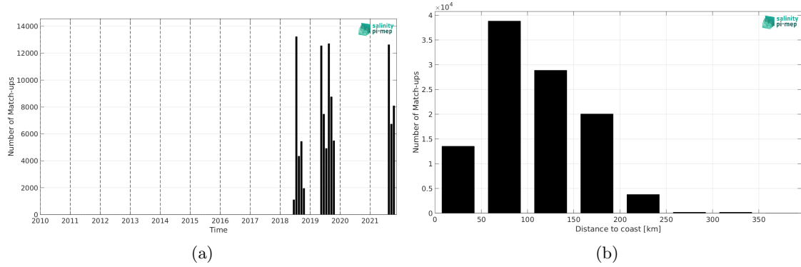
Figure 1: Number of match-ups between Saildrone and SMOS SSS L3 Arctic v2 - 9 Days (CATDS-CEC-LOCEAN) SSS as a function of time (a) and as function of the distance to coast (b) over the North Pacific Ocean Pi-MEP region and for the full satellite product period.
