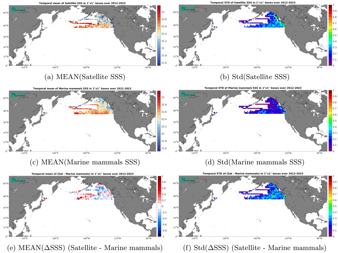
Figure 7: Temporal mean (left) and Std (right) of SSS from SMOS SSS L3 Arctic v2 - 9 Days (CATDS-CEC-LOCEAN) (top), Marine mammals (middle), and of \Delta SSS (Satellite - Marine mammals). Only match-up pairs are used to generate these maps.
