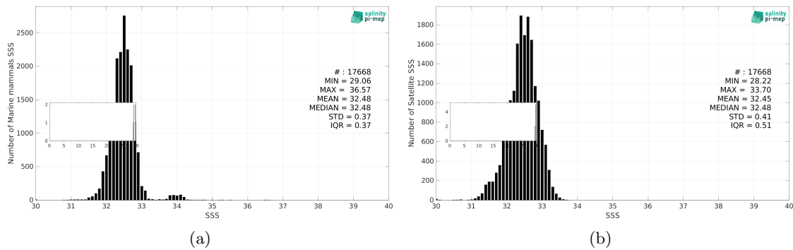
Figure 3: Histograms of SSS from Marine mammals (a) and SMOS SSS L3 Arctic v2 - 9 Days (CATDS-CEC-LOCEAN) (b) considering all match-up pairs per bins of 0.1 over the North Pacific Ocean Pi-MEP region and for the full satellite product period.
