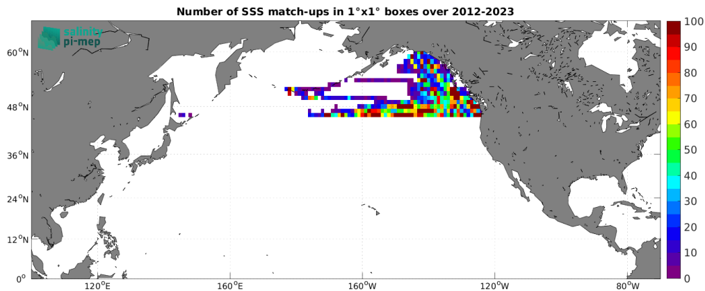
Figure 5: Number of SSS match-ups between Marine mammals SSS and the SMOS SSS L3 Arctic v2 - 9 Days (CATDS-CEC-LOCEAN) SSS product for the North Pacific Ocean Pi-MEP region over 1^\circ \times 1^\circ boxes and for the full satellite product period.
