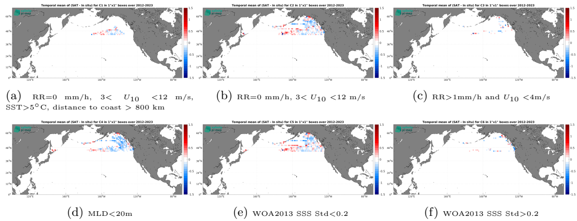
Figure 14: Temporal mean gridded over spatial boxes of size 1^\circ \times 1^\circ of \Delta SSS (SMOS SSS L3 Arctic v2 - 9 Days (CATDS-CEC-LOCEAN) - Marine mammals) for 6 different subdatasets corresponding to:RR=0 mm/h, 3 < U_{10} < 12 m/s, SST >5^\circ C, distance to coast > 800 km (a), RR=0 mm/h, 3 < U_{10} < 12 m/s (b), RR >1 mm/h and U_{10} < 4 m/s (c),MLD <20 m (d),WOA2013 SSS Std <0.2 (e),WOA2013 SSS Std >0.2 (f).
