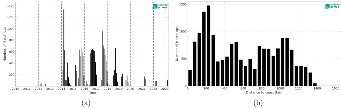
Figure 2: Number of match-ups between Marine mammals and SMOS SSS L3 Arctic v2 - 9 Days (CATDS-CEC-LOCEAN) SSS as a function of time (a) and as function of the distance to coast (b) over the North Pacific Ocean Pi-MEP region and for the full satellite product period.
