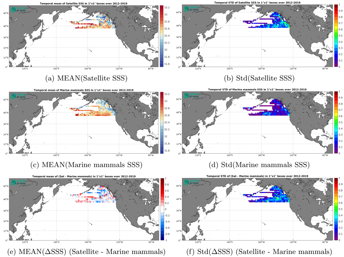
Figure 6: Temporal mean (left) and Std (right) of SSS from SMOS SSS L3 Arctic v2 - 9 Days (CATDS-CEC-LOCEAN) (top), Marine mammals (middle), and of \Delta SSS (Satellite - Marine mammals). Only match-up pairs are used to generate these maps.
