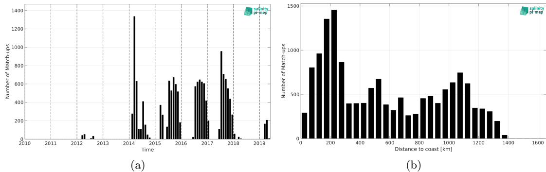
Figure 1: Number of match-ups between Marine mammals and SMOS SSS L3 Arctic v2 - 9 Days (CATDS-CEC-LOCEAN) SSS as a function of time (a) and as function of the distance to coast (b) over the North Pacific Ocean Pi-MEP region and for the full satellite product period.
