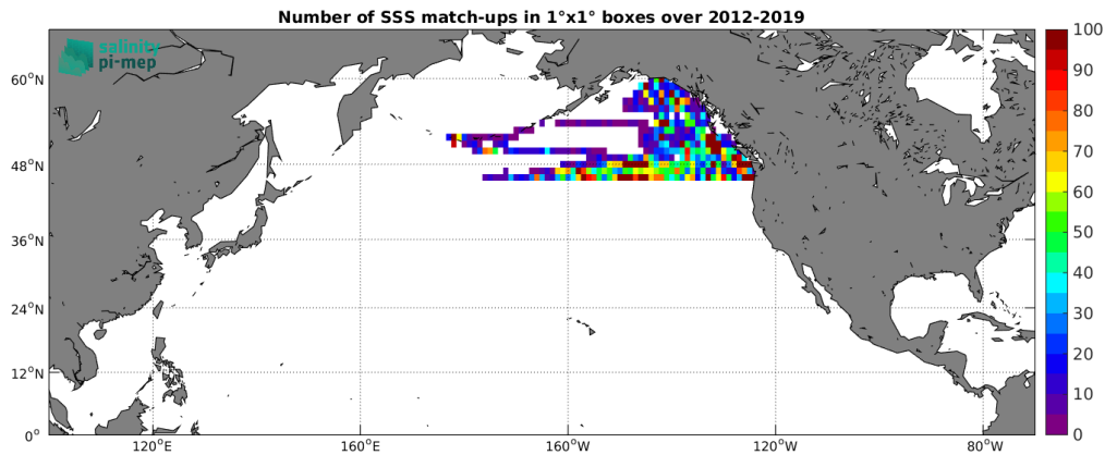
Figure 4: Number of SSS match-ups between Marine mammals SSS and the SMOS SSS L3 Arctic v2 - 9 Days (CATDS-CEC-LOCEAN) SSS product for the North Pacific Ocean Pi-MEP region over 1^\circ \times 1^\circ boxes and for the full satellite product period.
