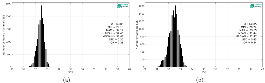
Figure 2: Histograms of SSS from Marine mammals (a) and SMOS SSS L3 Arctic v2 - 9 Days (CATDS-CEC-LOCEAN) (b) considering all match-up pairs per bins of 0.1 over the North Pacific Ocean Pi-MEP region and for the full satellite product period.
