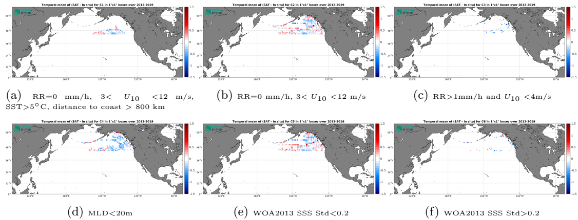
Figure 12: Temporal mean gridded over spatial boxes of size 1^{\circ}\times 1^{\circ} of \Delta\text{SSS} (SMOS SSS L3 Arctic v2 - 9 Days (CATDS-CEC-LOCEAN) - Marine mammals) for 6 different subdatasets corresponding to:RR=0 mm/h, 3 < U_{10} < 12 m/s, SST > 5^{\circ}\text{C} , distance to coast > 800 km (a), RR=0 mm/h, 3 < U_{10} < 12 m/s (b), RR > 1\text{mm/h} and U_{10} < 4\text{m/s} (c),MLD < 20\text{m} (d),WOA2013 SSS Std < 0.2 (e),WOA2013 SSS Std > 0.2 (f).
