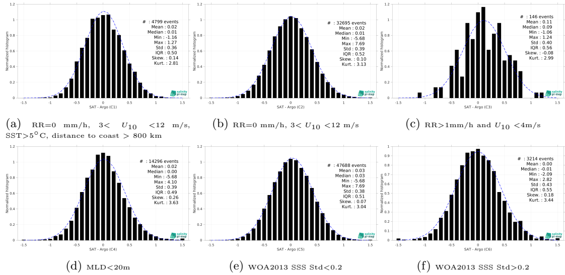
Figure 15: Normalized histogram of \Delta SSS (SMOS SSS L3 Arctic v2 - 9 Days (CATDS-CEC-LOCEAN) - Argo) for 6 different subdatasets corresponding to: RR=0 mm/h, 3 < U_{10} < 12 m/s, SST > 5°C, distance to coast > 800 km (a), RR=0 mm/h, 3 < U_{10} < 12 m/s (b), RR > 1mm/h and U_{10} < 4 m/s (c), MLD < 20m (d), WOA2013 SSS Std < 0.2 (e), WOA2013 SSS Std > 0.2 (f).
