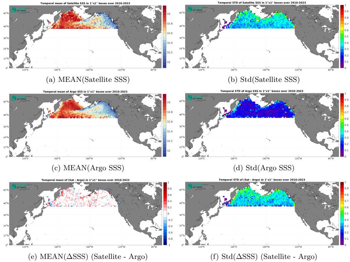
Figure 7: Temporal mean (left) and Std (right) of SSS from SMOS SSS L3 Arctic v2 - 9 Days (CATDS-CEC-LOCEAN) (top), Argo (middle), and of \Delta SSS (Satellite - Argo). Only match-up pairs are used to generate these maps.
