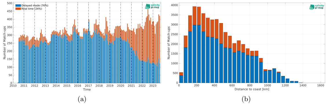
Figure 2: Number of match-ups between Argo and SMOS SSS L3 Arctic v2 - 9 Days (CATDS-CEC-LOCEAN) SSS as a function of time (a) and as function of the distance to coast (b) over the North Pacific Ocean Pi-MEP region and for the full satellite product period.
