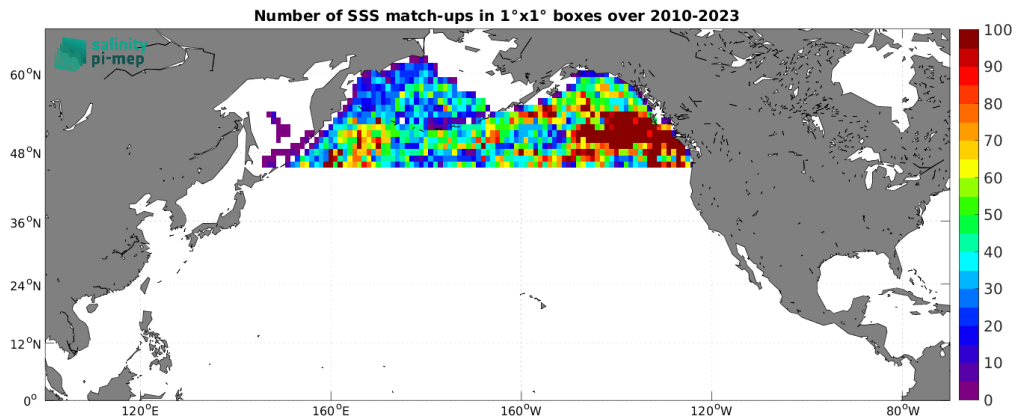
Figure 5: Number of SSS match-ups between Argo SSS and the SMOS SSS L3 Arctic v2 - 9 Days (CATDS-CEC-LOCEAN) SSS product for the North Pacific Ocean Pi-MEP region over 1^\circ \times 1^\circ boxes and for the full satellite product period.
