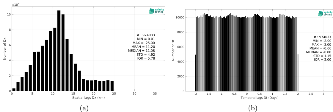
Figure 6: Histograms of the spatial (a) and temporal (b) lags between the location/time of the TSG (SAMOS) measurement and the date of the corresponding SMOS SSS L3 Arctic v2 - 18 Days (CATDS-CEC-LOCEAN) SSS pixel.
