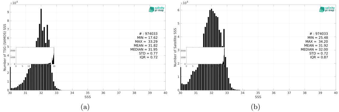
Figure 3: Histograms of SSS from TSG (SAMOS) (a) and SMOS SSS L3 Arctic v2 - 18 Days (CATDS-CEC-LOCEAN) (b) considering all match-up pairs per bins of 0.1 over the North Pacific Ocean Pi-MEP region and for the full satellite product period.
