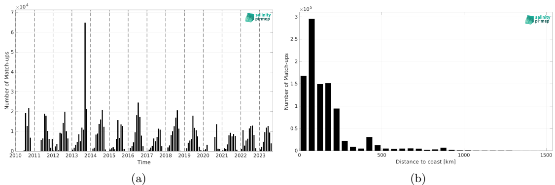
Figure 2: Number of match-ups between TSG (SAMOS) and SMOS SSS L3 Arctic v2 - 18 Days (CATDS-CEC-LOCEAN) SSS as a function of time (a) and as function of the distance to coast (b) over the North Pacific Ocean Pi-MEP region and for the full satellite product period.
