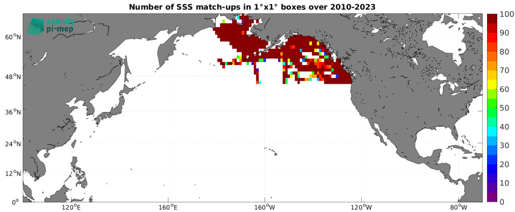
Figure 5: Number of SSS match-ups between TSG (SAMOS) SSS and the SMOS SSS L3 Arctic v2 - 18 Days (CATDS-CEC-LOCEAN) SSS product for the North Pacific Ocean Pi-MEP region over 1^\circ \times 1^\circ boxes and for the full satellite product period.
