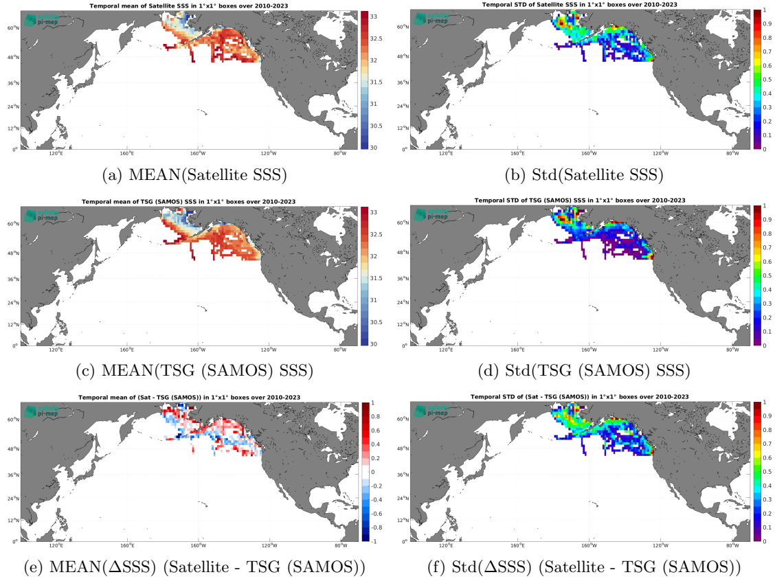
Figure 7: Temporal mean (left) and Std (right) of SSS from SMOS SSS L3 Arctic v2 - 18 Days (CATDS-CEC-LOCEAN) (top), TSG (SAMOS) (middle), and of \Delta SSS (Satellite - TSG (SAMOS)). Only match-up pairs are used to generate these maps.
