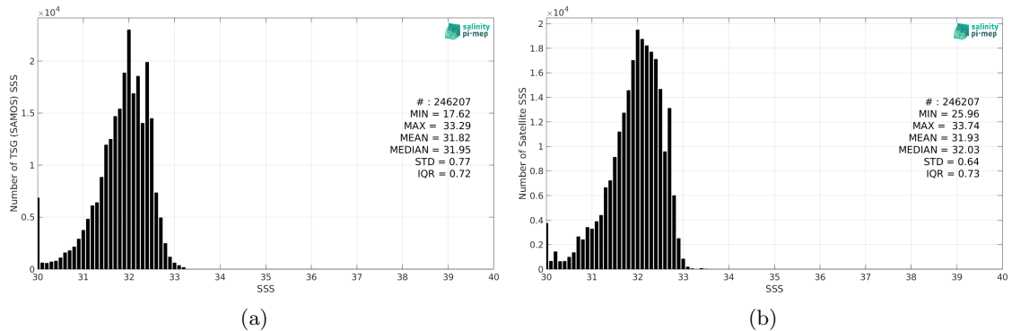
Figure 2: Histograms of SSS from TSG (SAMOS) (a) and SMOS SSS L3 Arctic v2 - 18 Days (CATDS-CEC-LOCEAN) (b) considering all match-up pairs per bins of 0.1 over the North Pacific Ocean Pi-MEP region and for the full satellite product period.
