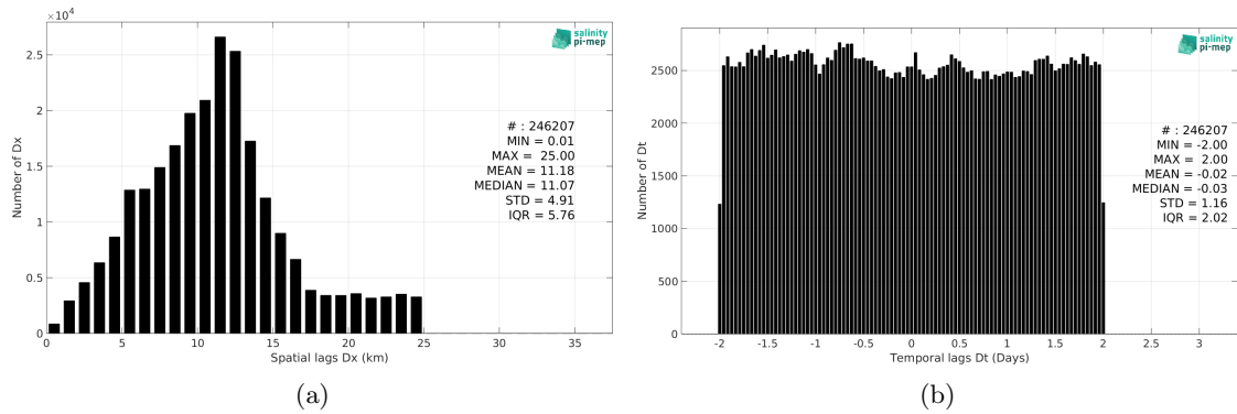
Figure 5: Histograms of the spatial (a) and temporal (b) lags between the location/time of the TSG (SAMOS) measurement and the date of the corresponding SMOS SSS L3 Arctic v2 - 18 Days (CATDS-CEC-LOCEAN) SSS pixel.
