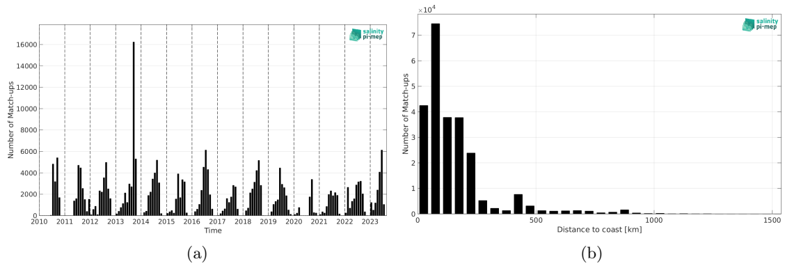
Figure 1: Number of match-ups between TSG (SAMOS) and SMOS SSS L3 Arctic v2 - 18 Days (CATDS-CEC-LOCEAN) SSS as a function of time (a) and as function of the distance to coast (b) over the North Pacific Ocean Pi-MEP region and for the full satellite product period.
