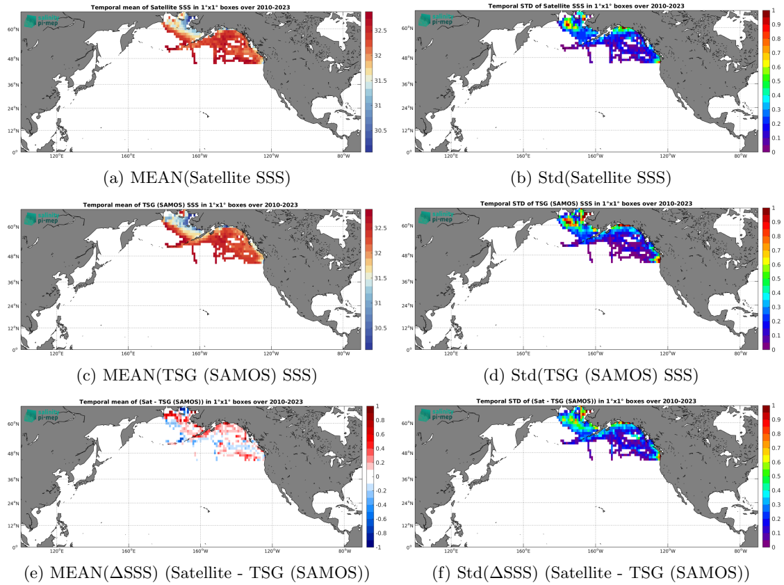
Figure 6: Temporal mean (left) and Std (right) of SSS from SMOS SSS L3 Arctic v2 - 18 Days (CATDS-CEC-LOCEAN) (top), TSG (SAMOS) (middle), and of \Delta SSS (Satellite - TSG (SAMOS)). Only match-up pairs are used to generate these maps.
