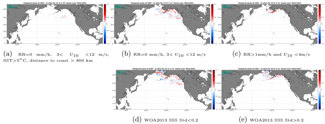
Figure 12: Temporal mean gridded over spatial boxes of size 1^{\circ}\times 1^{\circ} of \Delta\text{SSS} (SMOS SSS L3 Arctic v2 - 18 Days (CATDS-CEC-LOCEAN) - TSG (SAMOS)) for 5 different subdatasets corresponding to:RR=0 mm/h, 3 < U_{10} < 12 m/s, SST > 5^{\circ}\text{C} , distance to coast > 800 km (a), RR=0 mm/h, 3 < U_{10} < 12 m/s (b), RR > 1 mm/h and U_{10} < 4 m/s (c), WOA2013 SSS Std < 0.2 (d), WOA2013 SSS Std > 0.2 (e).
