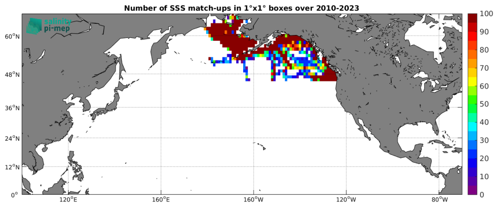
Figure 4: Number of SSS match-ups between TSG (SAMOS) SSS and the SMOS SSS L3 Arctic v2 - 18 Days (CATDS-CEC-LOCEAN) SSS product for the North Pacific Ocean Pi-MEP region over 1^\circ \times 1^\circ boxes and for the full satellite product period.
