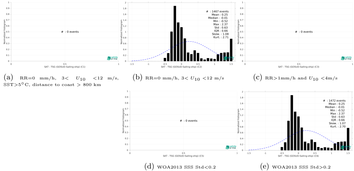
Figure 15: Normalized histogram of \Delta SSS (SMOS SSS L3 Arctic v2 - 18 Days (CATDS-CEC-LOCEAN) - TSG (GOSUD-Sailing-ship)) for 5 different subdatasets corresponding to: RR=0 mm/h, 3 < U_{10} < 12 m/s, SST > 5°C, distance to coast > 800 km (a), RR=0 mm/h, 3 < U_{10} < 12 m/s (b), RR > 1mm/h and U_{10} < 4 m/s (c), WOA2013 SSS Std < 0.2 (d), WOA2013 SSS Std > 0.2 (e).
