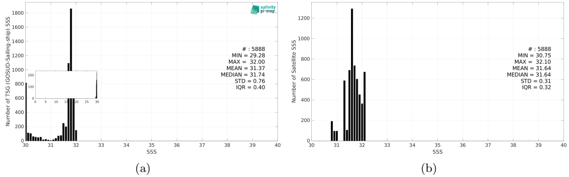
Figure 3: Histograms of SSS from TSG (GOSUD-Sailing-ship) (a) and SMOS SSS L3 Arctic v2 - 18 Days (CATDS-CEC-LOCEAN) (b) considering all match-up pairs per bins of 0.1 over the North Pacific Ocean Pi-MEP region and for the full satellite product period.
