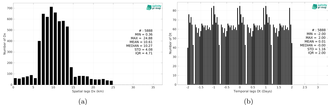
Figure 6: Histograms of the spatial (a) and temporal (b) lags between the location/time of the TSG (GOSUD-Sailing-ship) measurement and the date of the corresponding SMOS SSS L3 Arctic v2 - 18 Days (CATDS-CEC-LOCEAN) SSS pixel.
