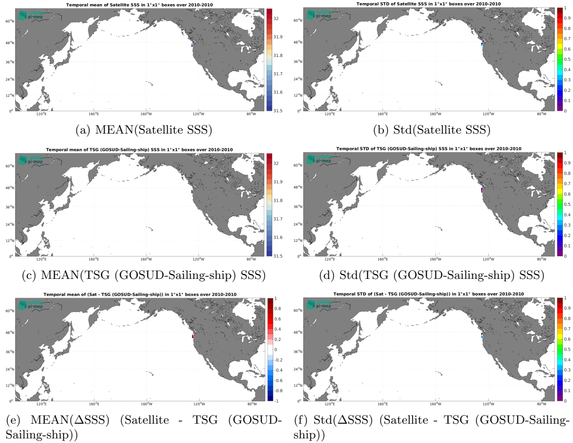
Figure 7: Temporal mean (left) and Std (right) of SSS from SMOS SSS L3 Arctic v2 - 18 Days (CATDS-CEC-LOCEAN) (top), TSG (GOSUD-Sailing-ship) (middle), and of \Delta\text{SSS} (Satellite - TSG (GOSUD-Sailing-ship)). Only match-up pairs are used to generate these maps.
