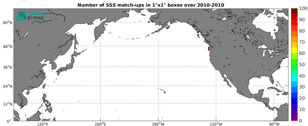
Figure 4: Number of SSS match-ups between TSG (GOSUD-Sailing-ship) SSS and the SMOS SSS L3 Arctic v2 - 18 Days (CATDS-CEC-LOCEAN) SSS product for the North Pacific Ocean Pi-MEP region over 1^\circ \times 1^\circ boxes and for the full satellite product period.
