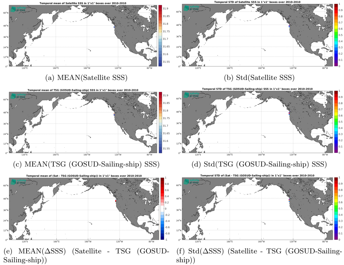
Figure 6: Temporal mean (left) and Std (right) of SSS from SMOS SSS L3 Arctic v2 - 18 Days (CATDS-CEC-LOCEAN) (top), TSG (GOSUD-Sailing-ship) (middle), and of \Delta SSS (Satellite - TSG (GOSUD-Sailing-ship)). Only match-up pairs are used to generate these maps.
