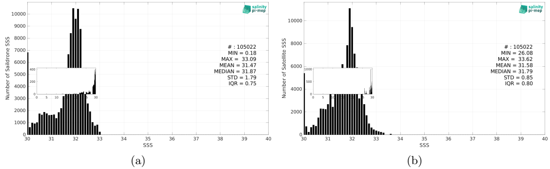
Figure 3: Histograms of SSS from Saildrone (a) and SMOS SSS L3 Arctic v2 - 18 Days (CATDS-CEC-LOCEAN) (b) considering all match-up pairs per bins of 0.1 over the North Pacific Ocean Pi-MEP region and for the full satellite product period.
