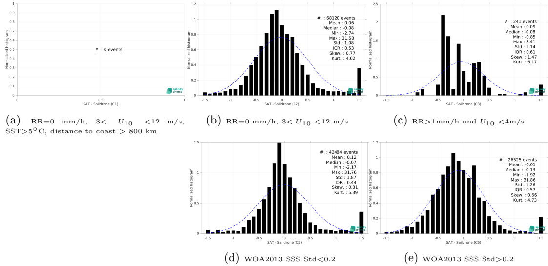
Figure 15: Normalized histogram of \Delta SSS (SMOS SSS L3 Arctic v2 - 18 Days (CATDS-CEC-LOCEAN) - Saldrone) for 5 different subdatasets corresponding to: RR=0 mm/h, 3 < U_{10} < 12 m/s, SST>5°C, distance to coast > 800 km (a), RR=0 mm/h, 3 < U_{10} < 12 m/s (b), RR>1mm/h and U_{10} < 4 m/s (c), WOA2013 SSS Std<0.2 (d), WOA2013 SSS Std>0.2 (e).
