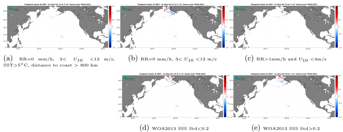
Figure 14: Temporal mean gridded over spatial boxes of size 1^\circ \times 1^\circ of \Delta SSS (SMOS SSS L3 Arctic v2 - 18 Days (CATDS-CEC-LOCEAN) - Saildrone) for 5 different subdatasets corresponding to:RR=0 mm/h, 3 < U_{10} < 12 m/s, SST >5^\circ\text{C} , distance to coast > 800 km (a), RR=0 mm/h, 3 < U_{10} < 12 m/s (b), RR >1 mm/h and U_{10} < 4 m/s (c), WOA2013 SSS Std <0.2 (d), WOA2013 SSS Std >0.2 (e).
