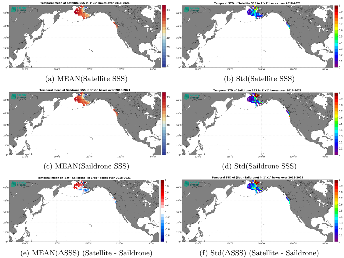
Figure 7: Temporal mean (left) and Std (right) of SSS from SMOS SSS L3 Arctic v2 - 18 Days (CATDS-CEC-LOCEAN) (top), Saildrone (middle), and of \Delta SSS (Satellite - Saildrone). Only match-up pairs are used to generate these maps.
