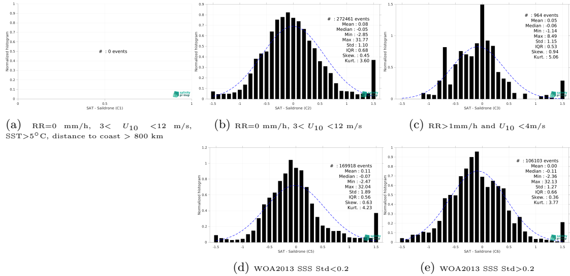
Figure 15: Normalized histogram of \Delta SSS (SMOS SSS L3 Arctic v2 - 18 Days (CATDS-CEC-LOCEAN) - Sailability) for 5 different subdatasets corresponding to: RR=0 mm/h, 3 < U_{10} < 12 m/s, SST > 5°C, distance to coast > 800 km (a), RR=0 mm/h, 3 < U_{10} < 12 m/s (b), RR > 1mm/h and U_{10} < 4 m/s (c), WOA2013 SSS Std < 0.2 (d), WOA2013 SSS Std > 0.2 (e).
