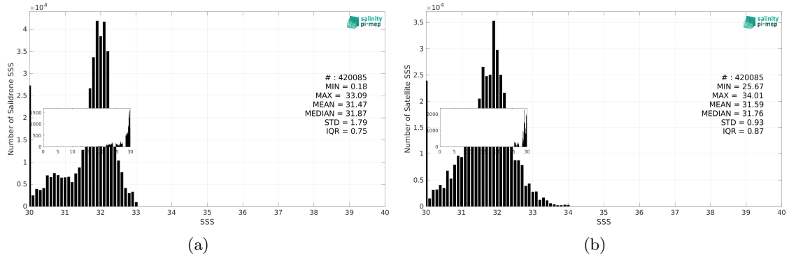
Figure 3: Histograms of SSS from Saildrone (a) and SMOS SSS L3 Arctic v2 - 18 Days (CATDS-CEC-LOCEAN) (b) considering all match-up pairs per bins of 0.1 over the North Pacific Ocean Pi-MEP region and for the full satellite product period.
