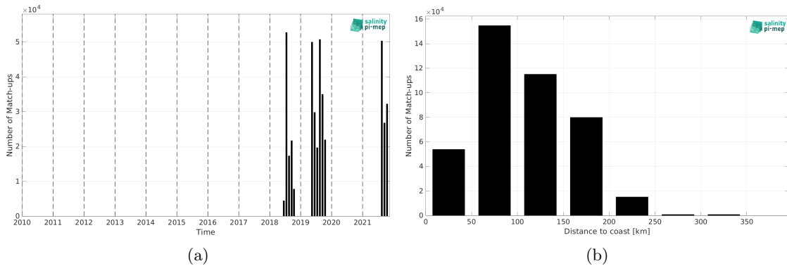
Figure 2: Number of match-ups between Saildrone and SMOS SSS L3 Arctic v2 - 18 Days (CATDS-CEC-LOCEAN) SSS as a function of time (a) and as function of the distance to coast (b) over the North Pacific Ocean Pi-MEP region and for the full satellite product period.
