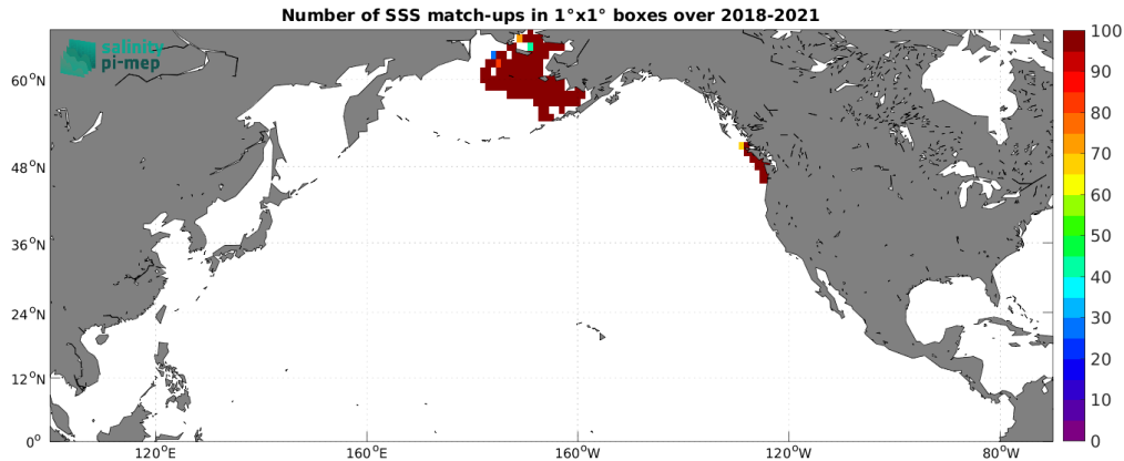
Figure 5: Number of SSS match-ups between Saildrone SSS and the SMOS SSS L3 Arctic v2 - 18 Days (CATDS-CEC-LOCEAN) SSS product for the North Pacific Ocean Pi-MEP region over 1^\circ \times 1^\circ boxes and for the full satellite product period.
