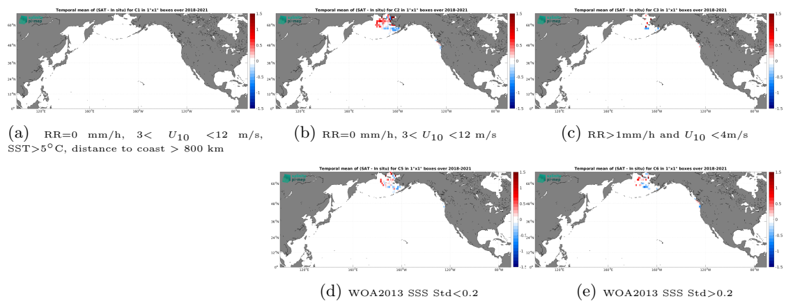
Figure 14: Temporal mean gridded over spatial boxes of size 1^\circ \times 1^\circ of \Delta\text{SSS} (SMOS SSS L3 Arctic v2 - 18 Days (CATDS-CEC-LOCEAN) - Saildrone) for 5 different subdatasets corresponding to:RR=0 mm/h, 3 < U_{10} < 12 m/s, SST >5^\circ\text{C} , distance to coast > 800 km (a), RR=0 mm/h, 3 < U_{10} < 12 m/s (b), RR >1 mm/h and U_{10} < 4 m/s (c), WOA2013 SSS Std <0.2 (d), WOA2013 SSS Std >0.2 (e).
