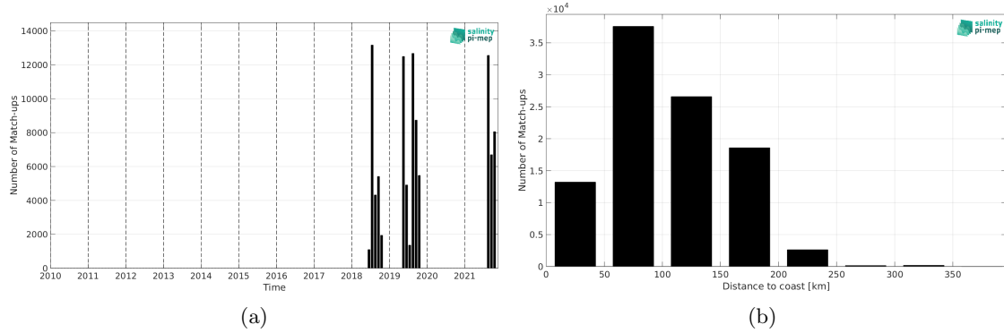
Figure 1: Number of match-ups between Saildrone and SMOS SSS L3 Arctic v2 - 18 Days (CATDS-CEC-LOCEAN) SSS as a function of time (a) and as function of the distance to coast (b) over the North Pacific Ocean Pi-MEP region and for the full satellite product period.
