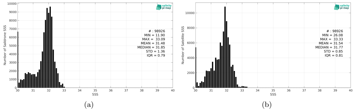
Figure 2: Histograms of SSS from Saildrone (a) and SMOS SSS L3 Arctic v2 - 18 Days (CATDS-CEC-LOCEAN) (b) considering all match-up pairs per bins of 0.1 over the North Pacific Ocean Pi-MEP region and for the full satellite product period.
