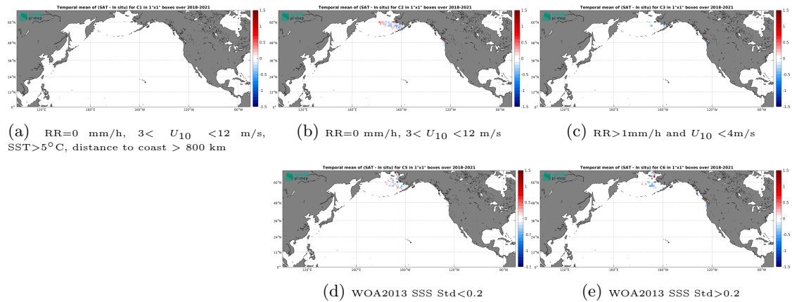
Figure 12: Temporal mean gridded over spatial boxes of size 1^{\circ}\times 1^{\circ} of \Delta\text{SSS} (SMOS SSS L3 Arctic v2 - 18 Days (CATDS-CEC-LOCEAN) - Saildrone) for 5 different subdatasets corresponding to: RR=0 mm/h, 3 < U_{10} < 12 m/s, SST > 5^{\circ}\text{C} , distance to coast > 800 km (a), RR=0 mm/h, 3 < U_{10} < 12 m/s (b), RR > 1 mm/h and U_{10} < 4 m/s (c), WOA2013 SSS Std < 0.2 (d), WOA2013 SSS Std > 0.2 (e).
