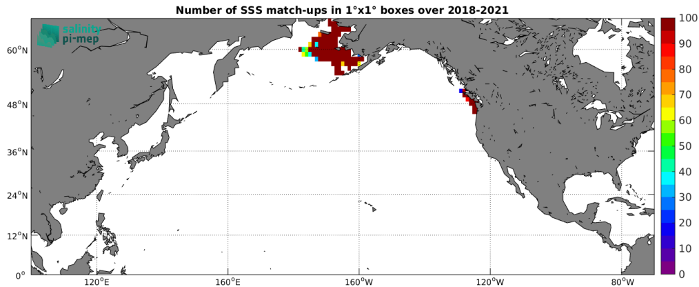
Figure 4: Number of SSS match-ups between Saildrone SSS and the SMOS SSS L3 Arctic v2 - 18 Days (CATDS-CEC-LOCEAN) SSS product for the North Pacific Ocean Pi-MEP region over 1^\circ \times 1^\circ boxes and for the full satellite product period.
