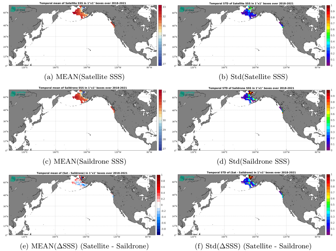
Figure 6: Temporal mean (left) and Std (right) of SSS from SMOS SSS L3 Arctic v2 - 18 Days (CATDS-CEC-LOCEAN) (top), Saildrone (middle), and of \Delta SSS (Satellite - Saildrone). Only match-up pairs are used to generate these maps.
