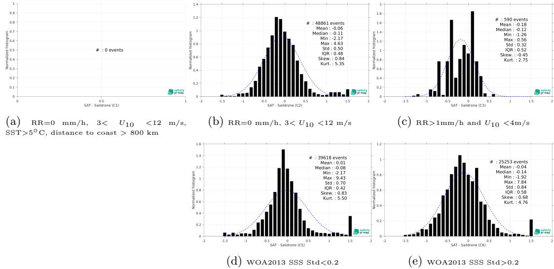
Figure 13: Normalized histogram of \Delta SSS (SMOS SSS L3 Arctic v2 - 18 Days (CATDS-CEC-LOCEAN) - Saildrone) for 5 different subdatasets corresponding to: RR=0 mm/h, 3 < U_{10} < 12 m/s, SST > 5°C, distance to coast > 800 km (a), RR=0 mm/h, 3 < U_{10} < 12 m/s (b), RR > 1mm/h and U_{10} < 4 m/s (c), WOA2013 SSS Std < 0.2 (d), WOA2013 SSS Std > 0.2 (e).
