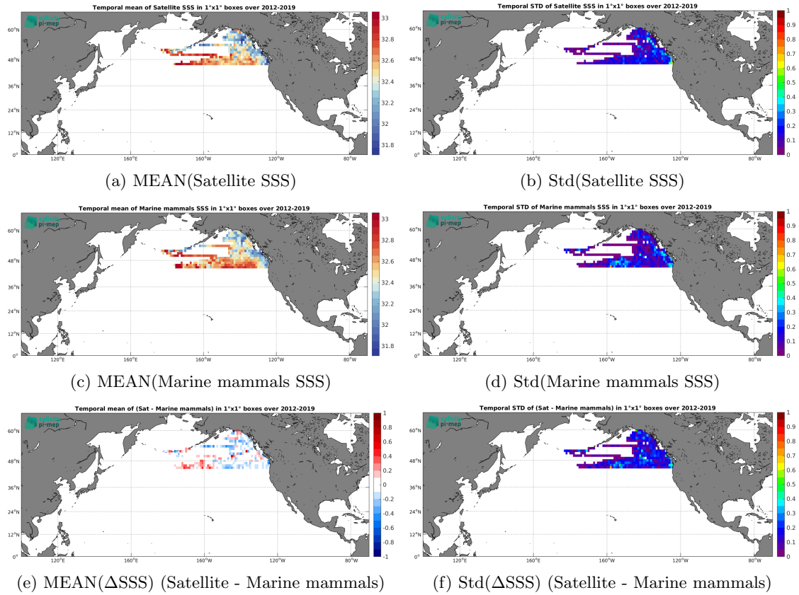
Figure 6: Temporal mean (left) and Std (right) of SSS from SMOS SSS L3 Arctic v2 - 18 Days (CATDS-CEC-LOCEAN) (top), Marine mammals (middle), and of \Delta SSS (Satellite - Marine mammals). Only match-up pairs are used to generate these maps.
