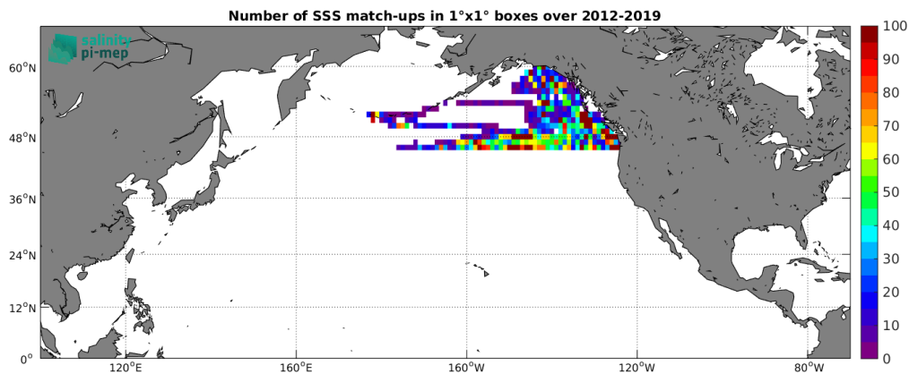
Figure 4: Number of SSS match-ups between Marine mammals SSS and the SMOS SSS L3 Arctic v2 - 18 Days (CATDS-CEC-LOCEAN) SSS product for the North Pacific Ocean Pi-MEP region over 1^\circ \times 1^\circ boxes and for the full satellite product period.
