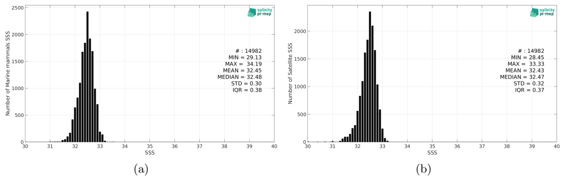
Figure 2: Histograms of SSS from Marine mammals (a) and SMOS SSS L3 Arctic v2 - 18 Days (CATDS-CEC-LOCEAN) (b) considering all match-up pairs per bins of 0.1 over the North Pacific Ocean Pi-MEP region and for the full satellite product period.
