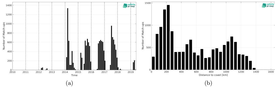
Figure 1: Number of match-ups between Marine mammals and SMOS SSS L3 Arctic v2 - 18 Days (CATDS-CEC-LOCEAN) SSS as a function of time (a) and as function of the distance to coast (b) over the North Pacific Ocean Pi-MEP region and for the full satellite product period.
