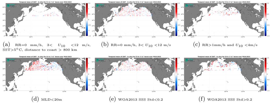
Figure 14: Temporal mean gridded over spatial boxes of size 1^\circ \times 1^\circ of \Delta SSS (SMOS SSS L3 Arctic v2 - 18 Days (CATDS-CEC-LOCEAN) - Argo) for 6 different subdatasets corresponding to:RR=0 mm/h, 3 < U_{10} < 12 m/s, SST >5^\circ C, distance to coast > 800 km (a), RR=0 mm/h, 3 < U_{10} < 12 m/s (b), RR >1 mm/h and U_{10} < 4 m/s (c),MLD <20 m (d),WOA2013 SSS Std <0.2 (e),WOA2013 SSS Std >0.2 (f).
