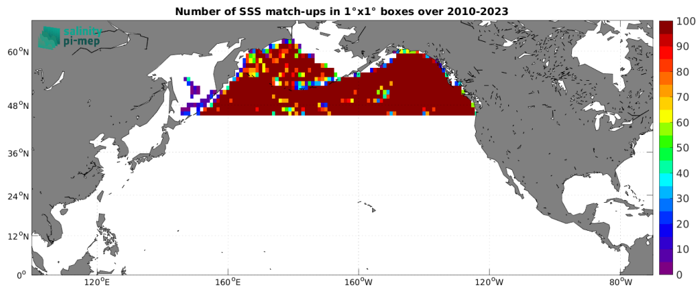
Figure 5: Number of SSS match-ups between Argo SSS and the SMOS SSS L3 Arctic v2 - 18 Days (CATDS-CEC-LOCEAN) SSS product for the North Pacific Ocean Pi-MEP region over 1^\circ \times 1^\circ boxes and for the full satellite product period.
