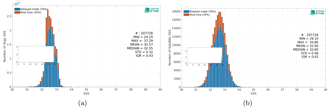
Figure 3: Histograms of SSS from Argo (a) and SMOS SSS L3 Arctic v2 - 18 Days (CATDS-CEC-LOCEAN) (b) considering all match-up pairs per bins of 0.1 over the North Pacific Ocean Pi-MEP region and for the full satellite product period.
