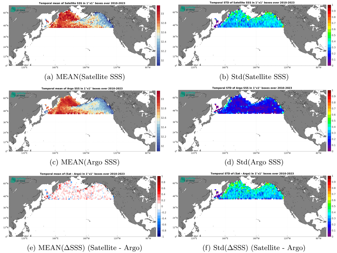
Figure 7: Temporal mean (left) and Std (right) of SSS from SMOS SSS L3 Arctic v2 - 18 Days (CATDS-CEC-LOCEAN) (top), Argo (middle), and of \Delta SSS (Satellite - Argo). Only match-up pairs are used to generate these maps.
