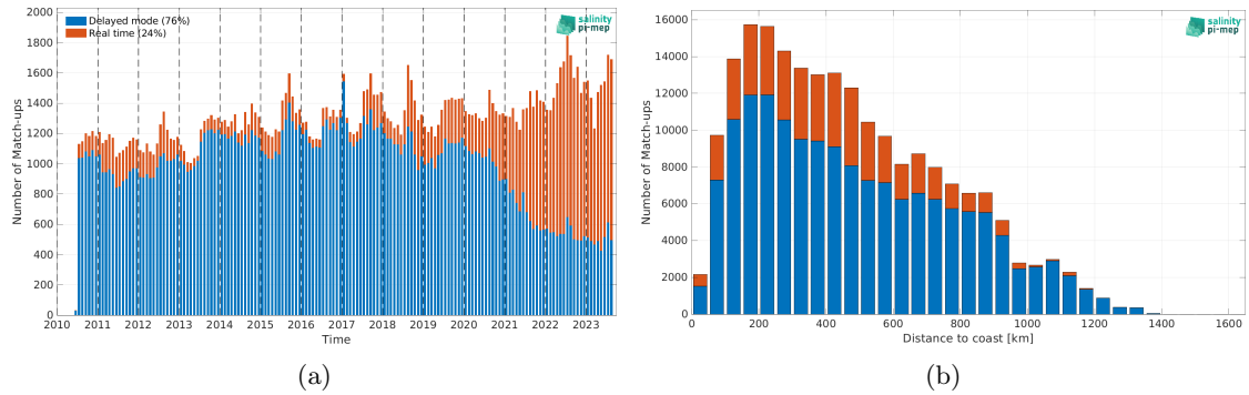
Figure 2: Number of match-ups between Argo and SMOS SSS L3 Arctic v2 - 18 Days (CATDS-CEC-LOCEAN) SSS as a function of time (a) and as function of the distance to coast (b) over the North Pacific Ocean Pi-MEP region and for the full satellite product period.
