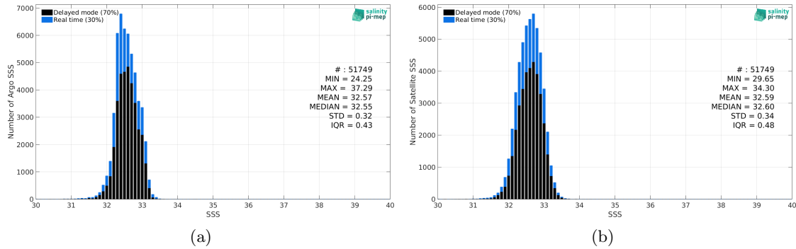
Figure 2: Histograms of SSS from Argo (a) and SMOS SSS L3 Arctic v2 - 18 Days (CATDS-CEC-LOCEAN) (b) considering all match-up pairs per bins of 0.1 over the North Pacific Ocean Pi-MEP region and for the full satellite product period.
