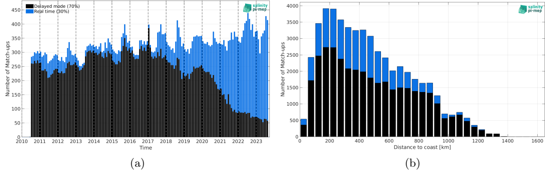
Figure 1: Number of match-ups between Argo and SMOS SSS L3 Arctic v2 - 18 Days (CATDS-CEC-LOCEAN) SSS as a function of time (a) and as function of the distance to coast (b) over the North Pacific Ocean Pi-MEP region and for the full satellite product period.
