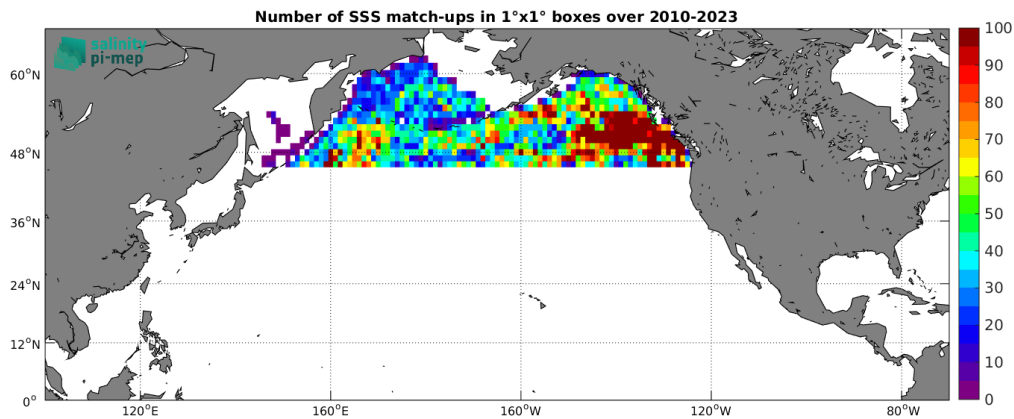
Figure 4: Number of SSS match-ups between Argo SSS and the SMOS SSS L3 Arctic v2 - 18 Days (CATDS-CEC-LOCEAN) SSS product for the North Pacific Ocean Pi-MEP region over 1^\circ \times 1^\circ boxes and for the full satellite product period.
