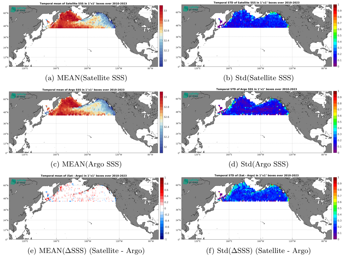
Figure 6: Temporal mean (left) and Std (right) of SSS from SMOS SSS L3 Arctic v2 - 18 Days (CATDS-CEC-LOCEAN) (top), Argo (middle), and of \Delta SSS (Satellite - Argo). Only match-up pairs are used to generate these maps.
