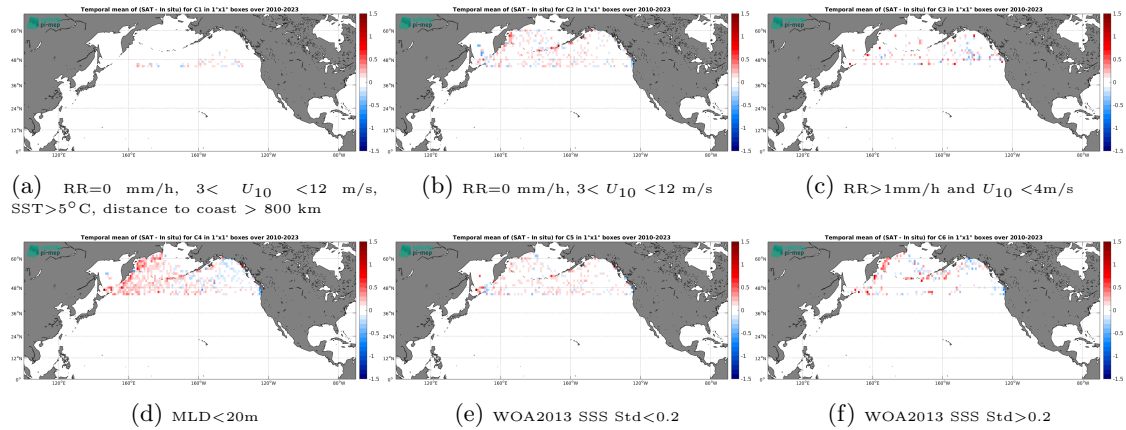
Figure 12: Temporal mean gridded over spatial boxes of size 1^{\circ}\times 1^{\circ} of \Delta\text{SSS} (SMOS SSS L3 Arctic v2 - 18 Days (CATDS-CEC-LOCEAN) - Argo) for 6 different subdatasets corresponding to:RR=0 mm/h, 3 < U_{10} < 12 m/s, SST > 5^{\circ}\text{C} , distance to coast > 800 km (a), RR=0 mm/h, 3 < U_{10} < 12 m/s (b), RR > 1\text{mm/h} and U_{10} < 4\text{m/s} (c),MLD < 20\text{m} (d),WOA2013 SSS Std < 0.2 (e),WOA2013 SSS Std > 0.2 (f).
